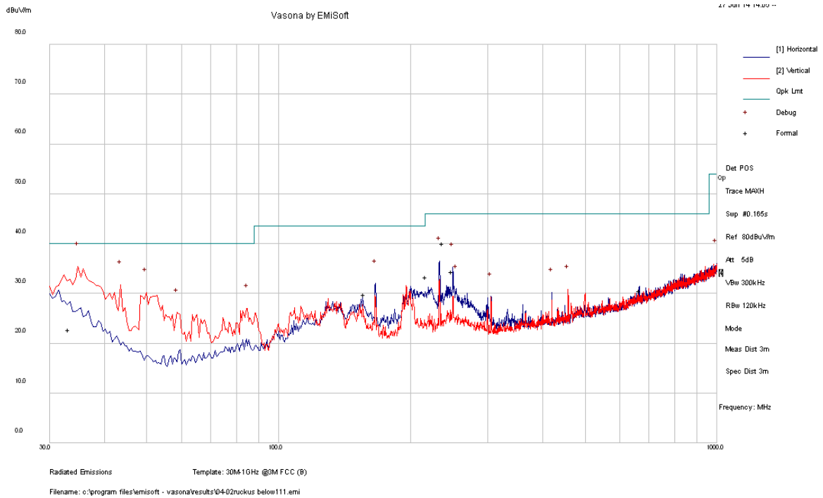
2.4 GHz Band, Quasi-Peak Measurements, worst case
