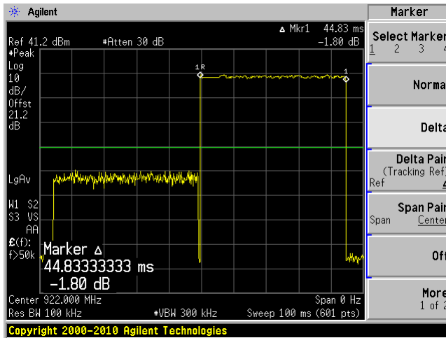
Channel: 922.0 MHz
