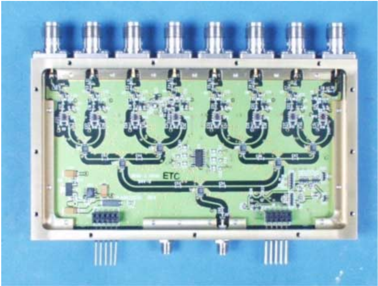
Multiplexer, Bottom
