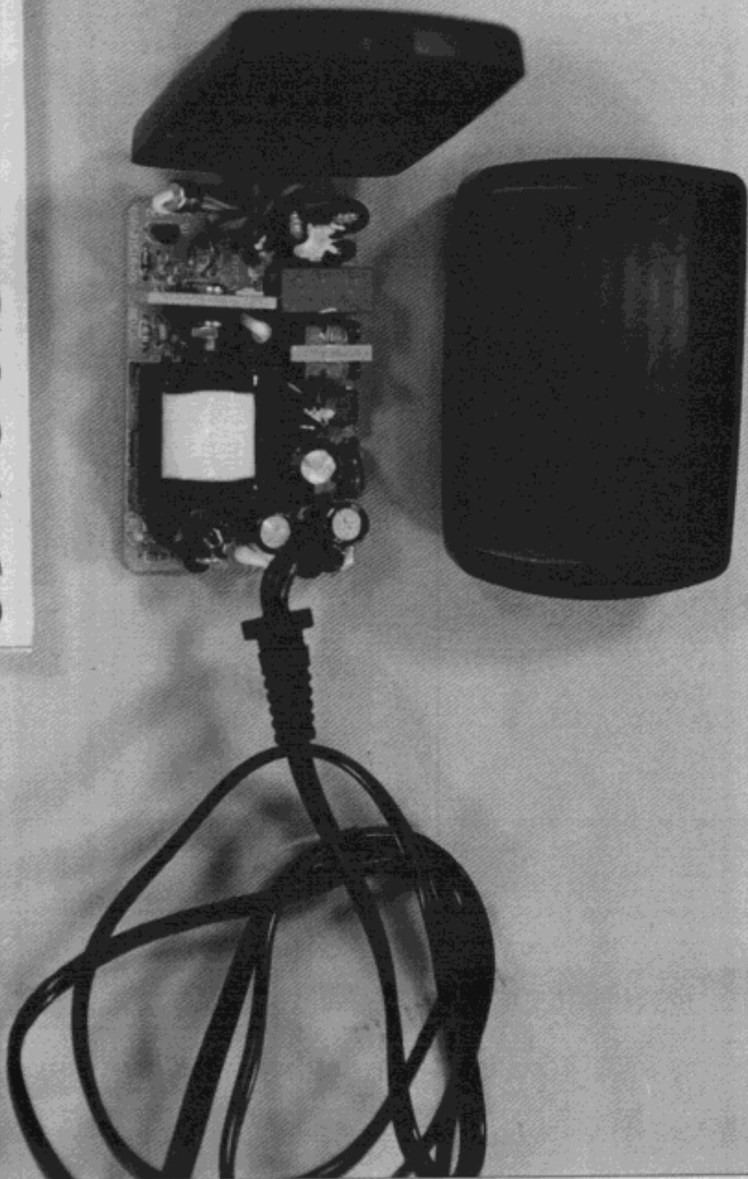
Figure 3 Cover & PCB View of Power Adapter
