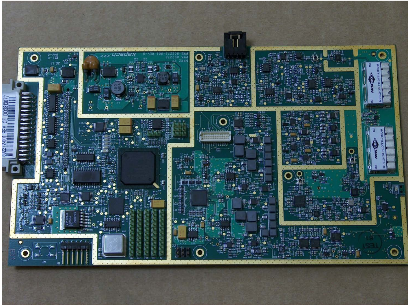
JANUS MRFM-S RX section – top view
