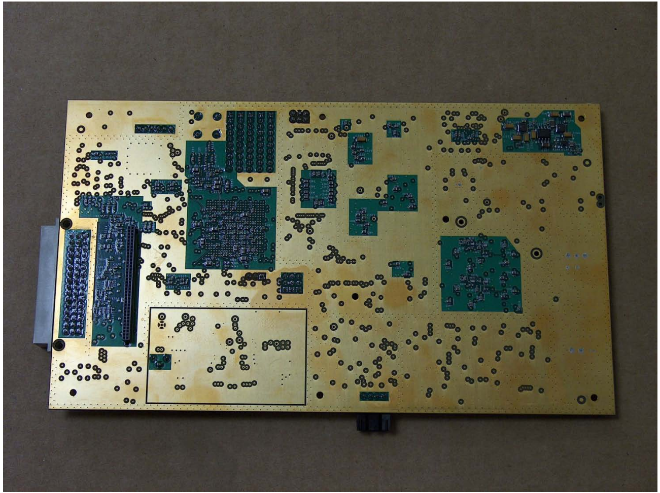
JANUS MRFM-S RX section – bottom view
