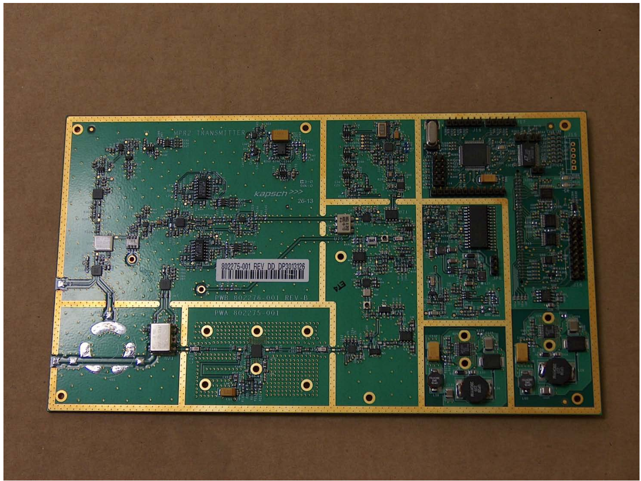
JANUS MRFM-S TX section – top view
