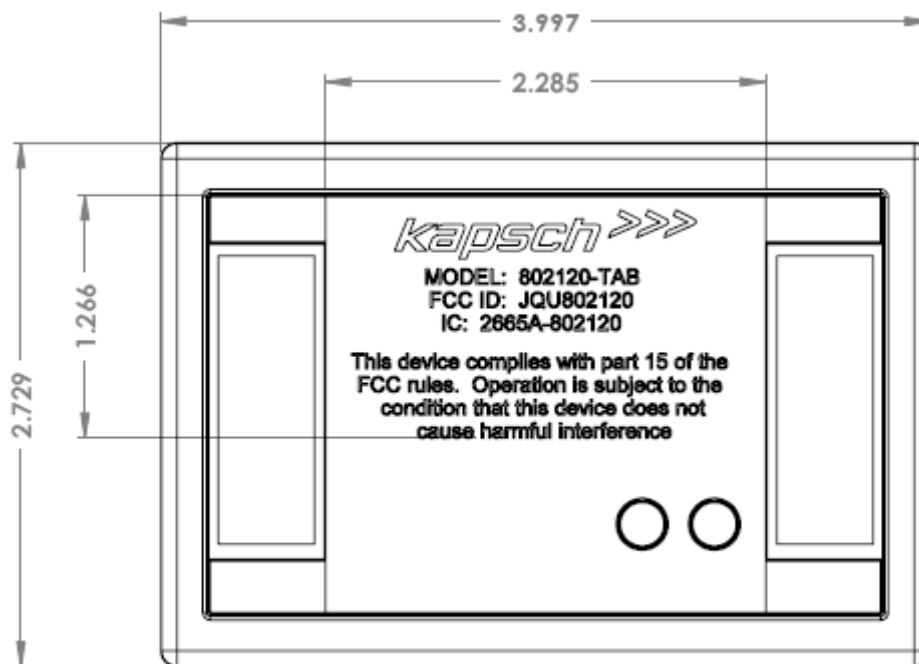
HOT TRANSPONDER REAR VIEW PROPOSED MARKING
