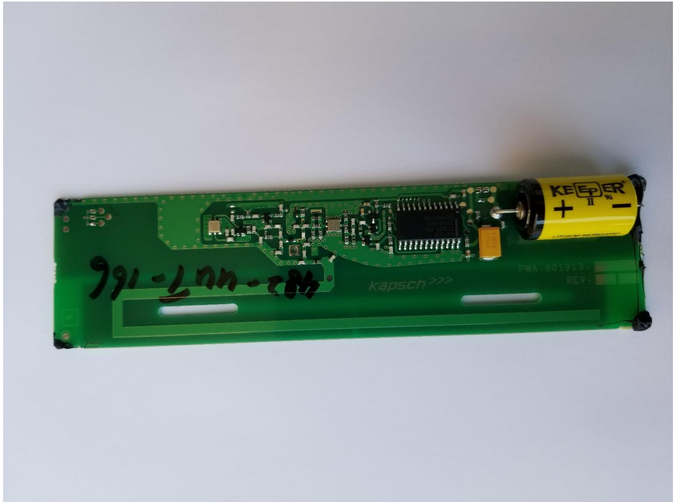
PWA Front Photo – Model 801800C -TAB
