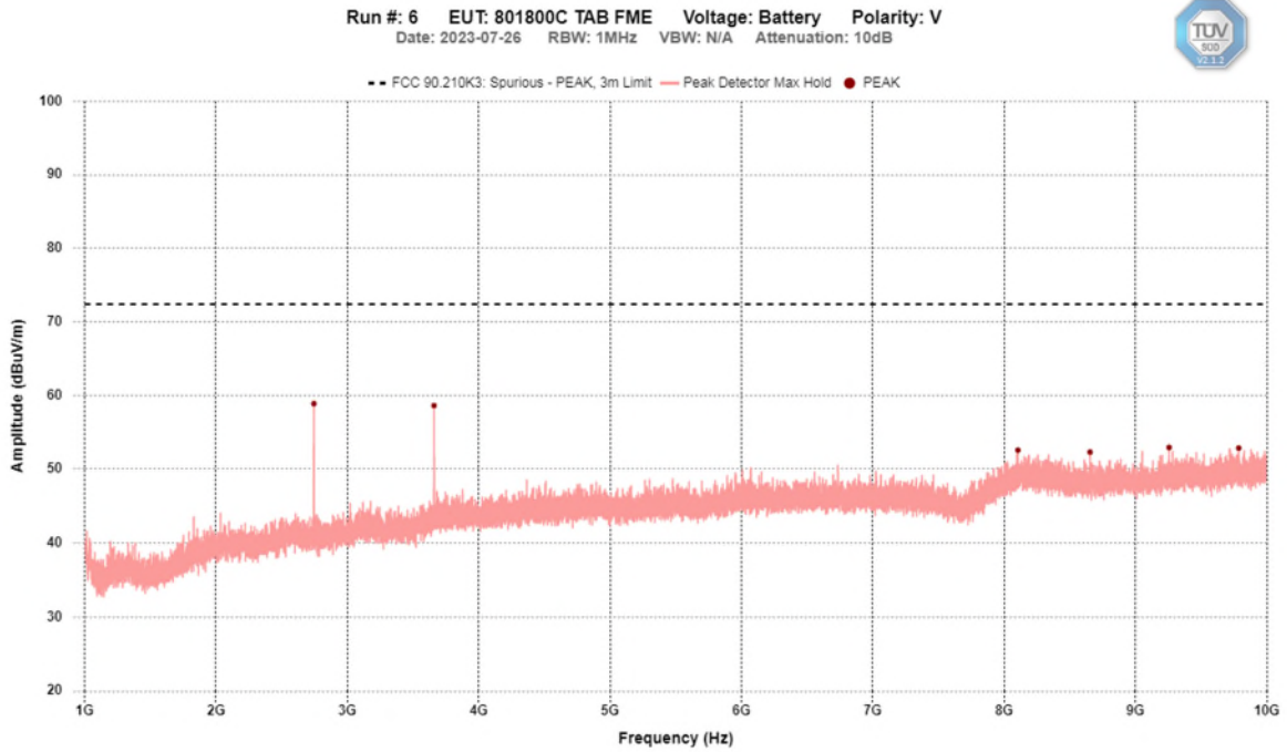
Vertical – Peak Emission Graph 1 GHz – 10 GHz
