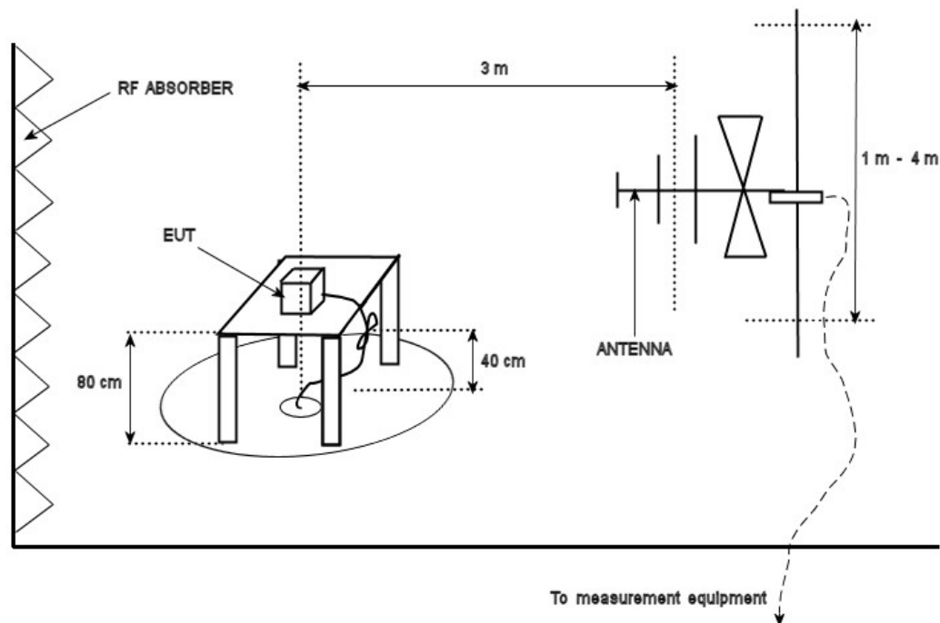
Typical Radiated Emissions Setup
