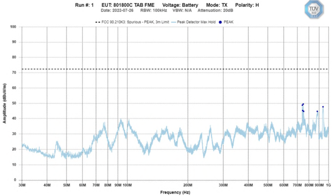
Horizontal – Peak Emission Graph 30 MHz – 1 GHz
