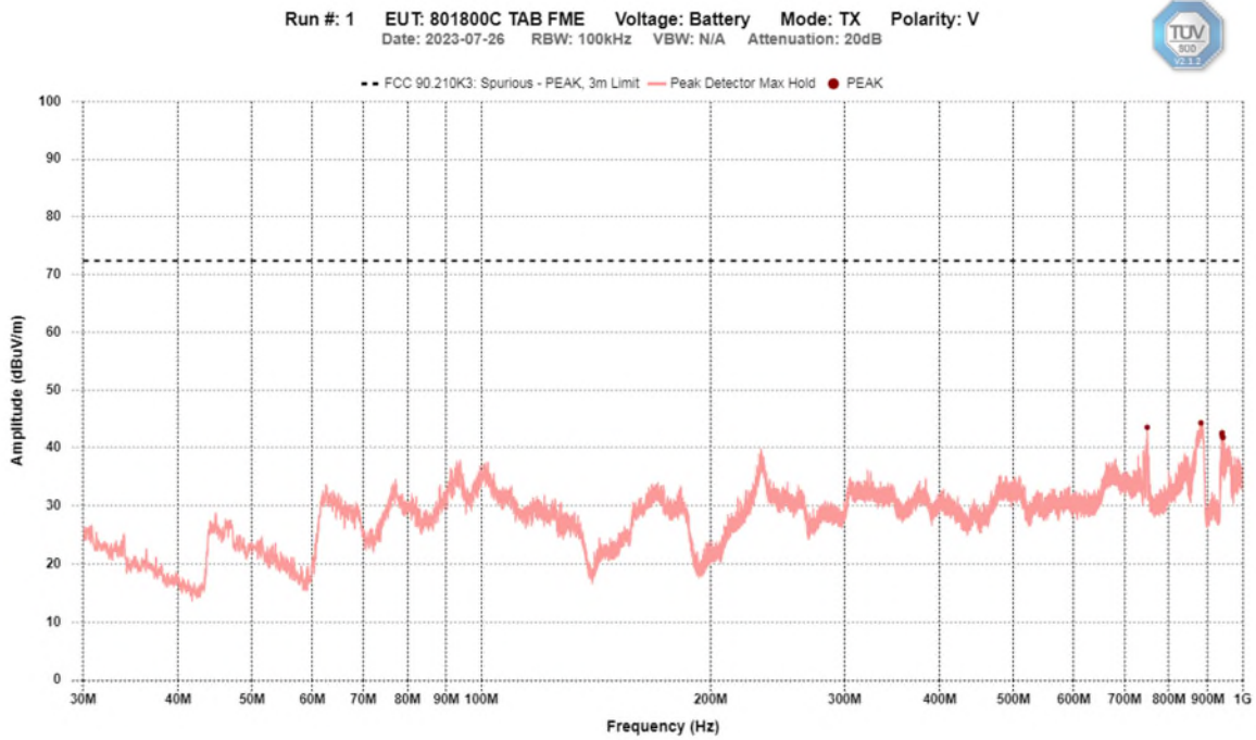
Vertical – Peak Emission Graph 30 MHz – 1 GHz
