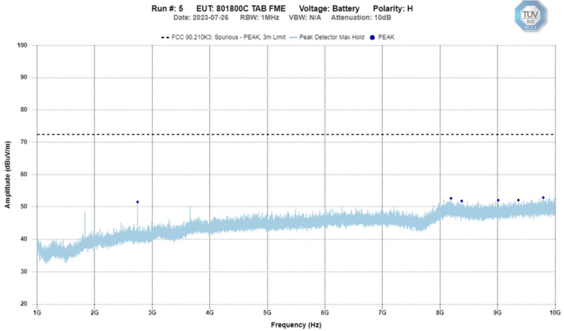
Horizontal – Peak Emission Graph 1 GHz – 10 GHz
