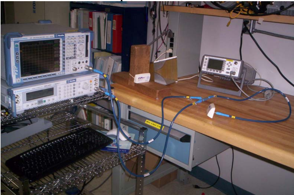
Conducted Measurement Setup:
