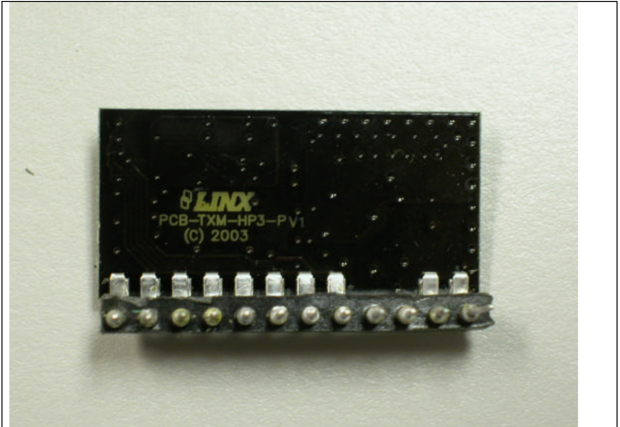
RF Circuit PCB Back Side
