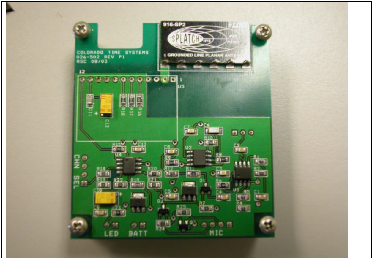
PCB RF Circuit Removed
