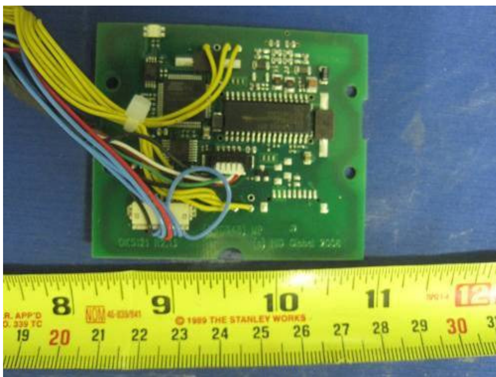
PCB 5 Component View (5121 RFID)
