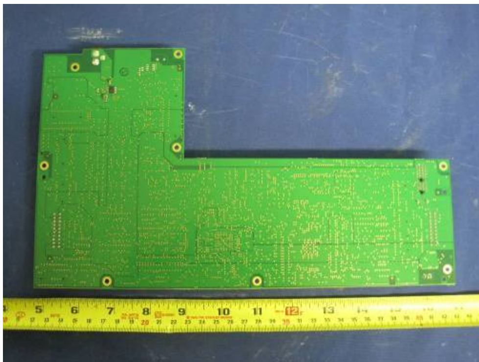
PCB 2 Solder View (Ribbon RFID)
