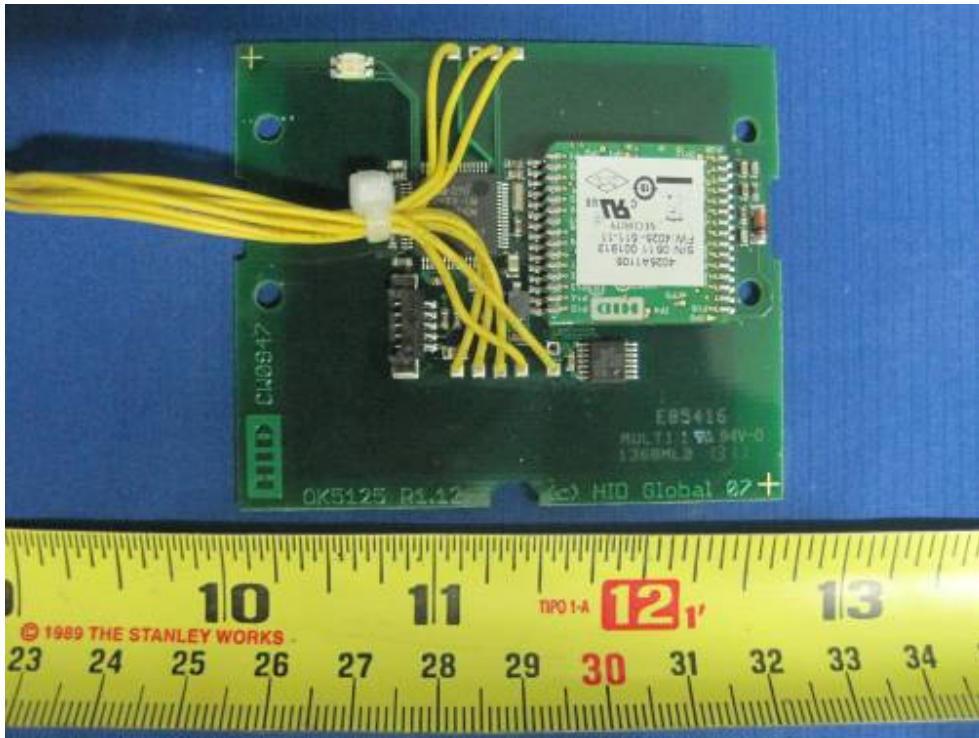
PCB 4 Component View (E-card 125KHz 5125RFID and antenna)
