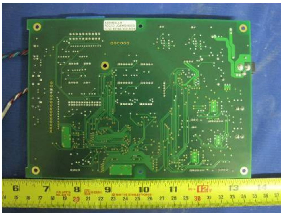
PCB 1 Solder View ( Laminator RFID)
