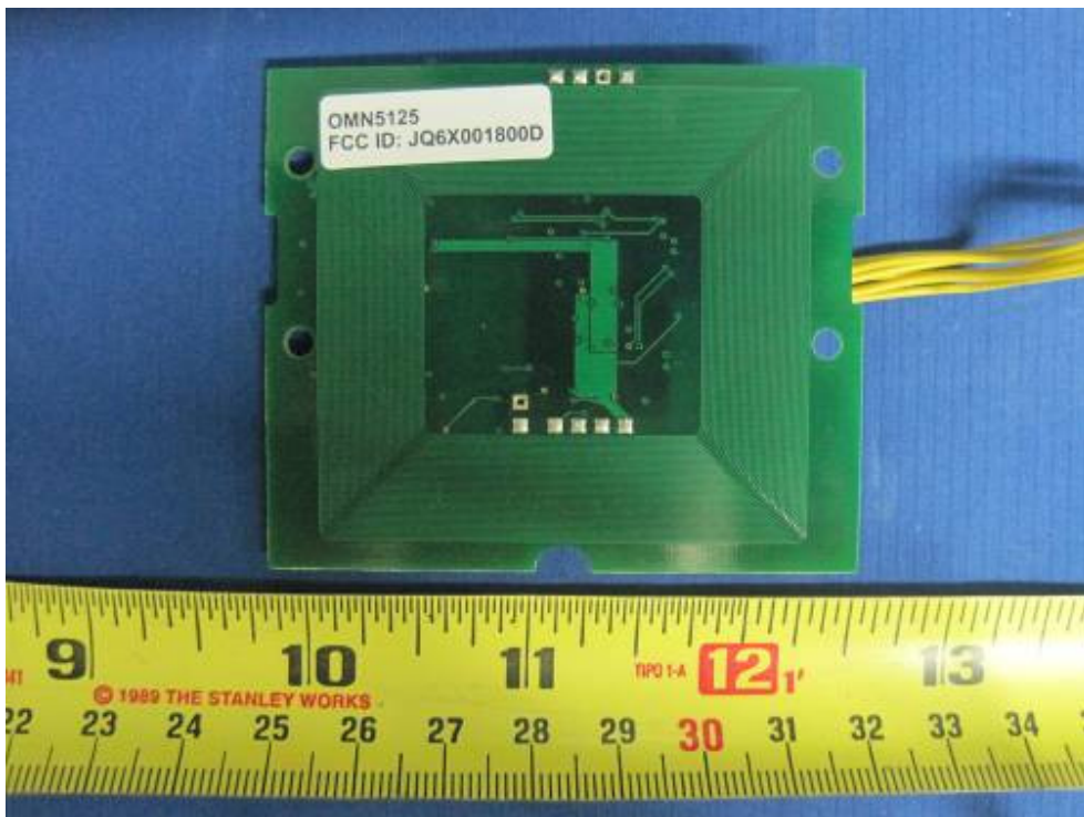
PCB 4 Solder View (E-card 125KHz 5125RFID and antenna)
