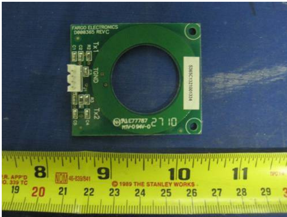
13.56MHz RFID Antenna Board (Ribbon) Component View
