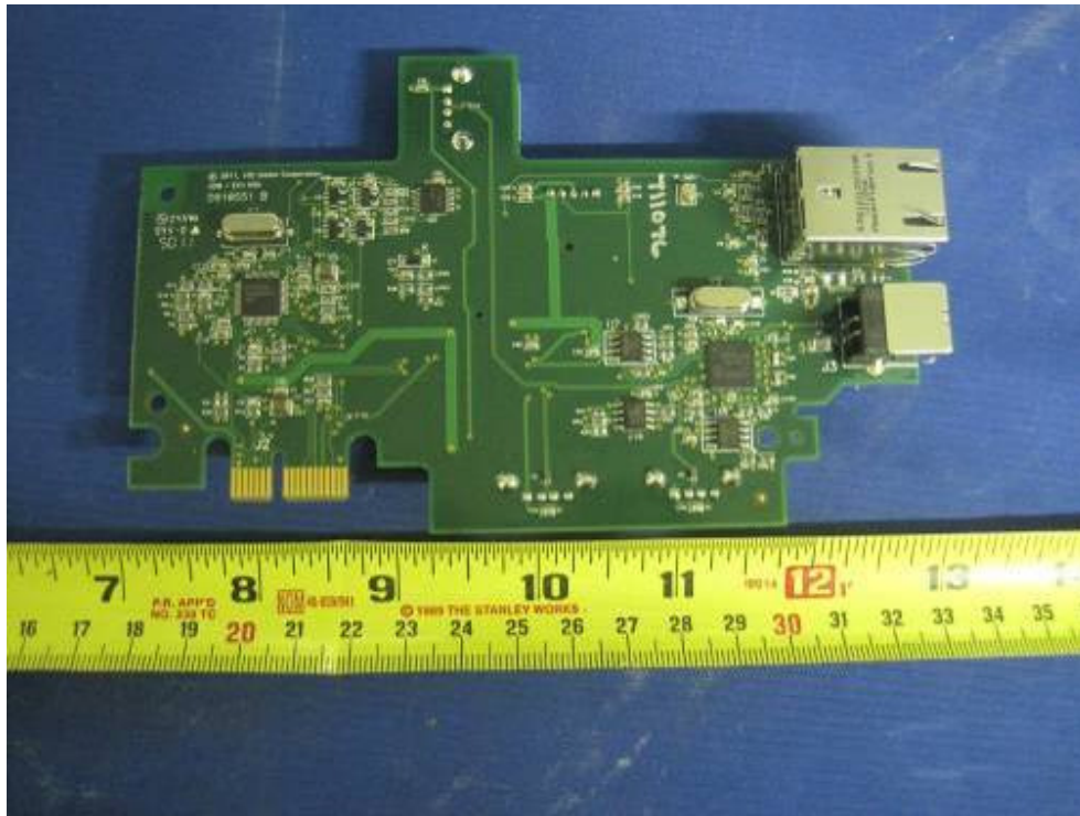
PCB 6 Component View
