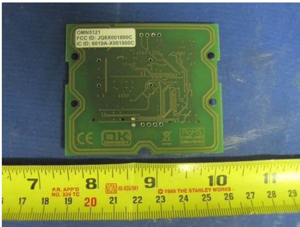
PCB 3 Solder View (5121SDI RFID)
