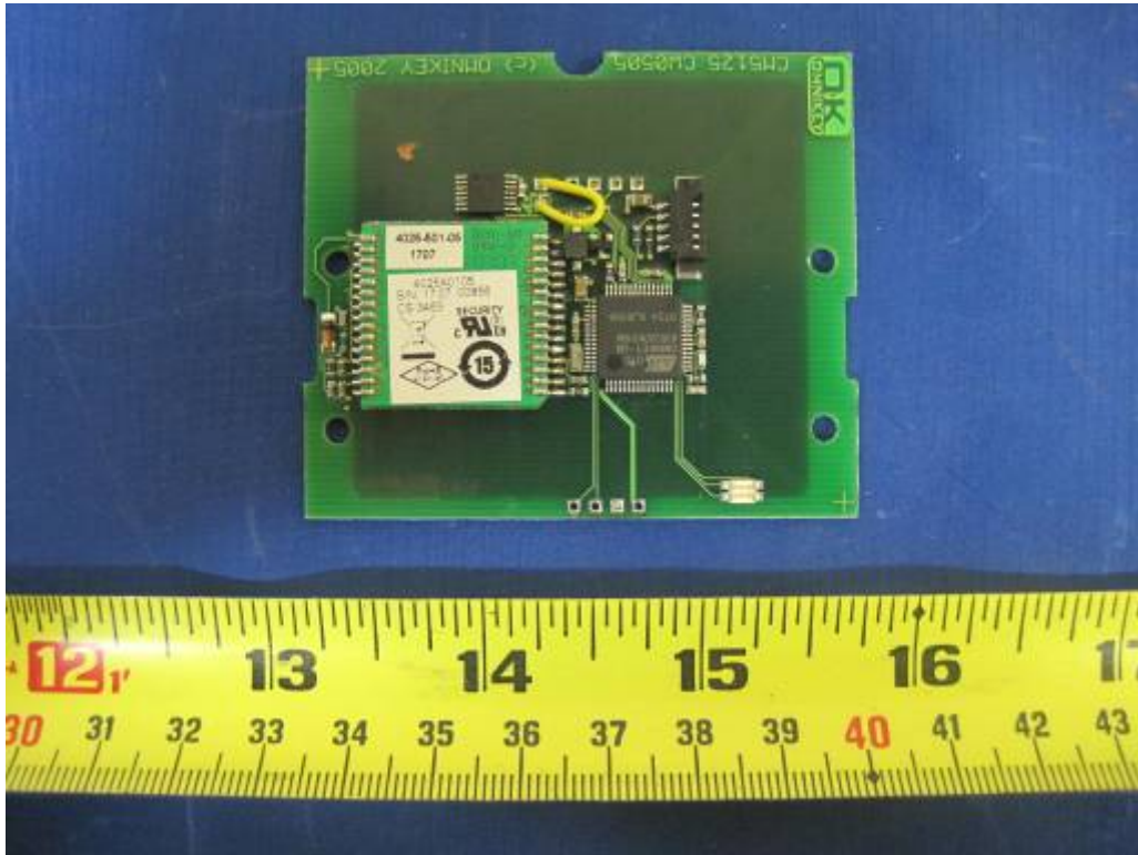
Component View (OMNI 5125 E-card 125KHz RFID and antenna)
