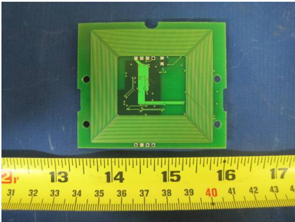
Solder View (OMNI 5125 E-card 125KHz RFID and antenna)
