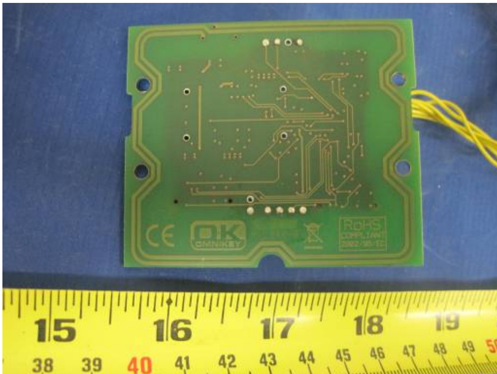
PCB 3 Solder View (OMN5121 E-card 13.56MHz RFID and antenna)
