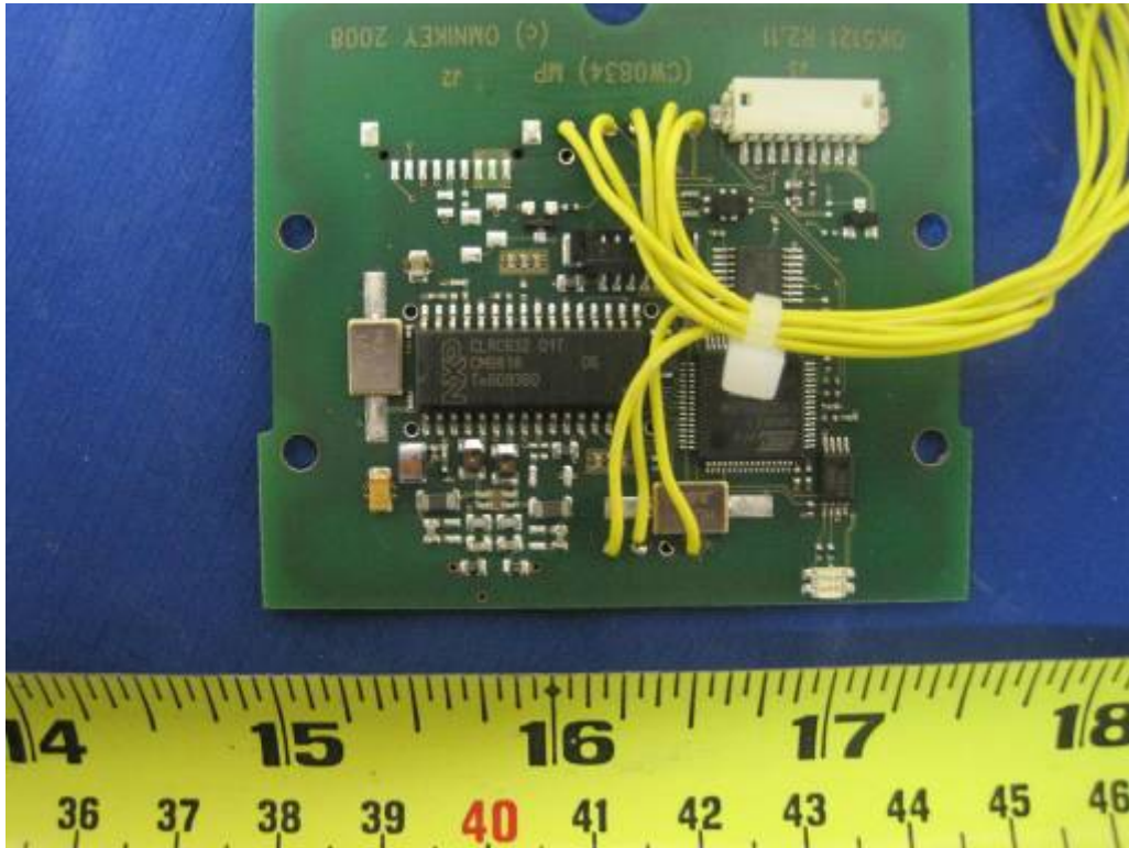
PCB 3 Component View (OMN 5121 E-card 13.56MHz RFID and Antenna)
