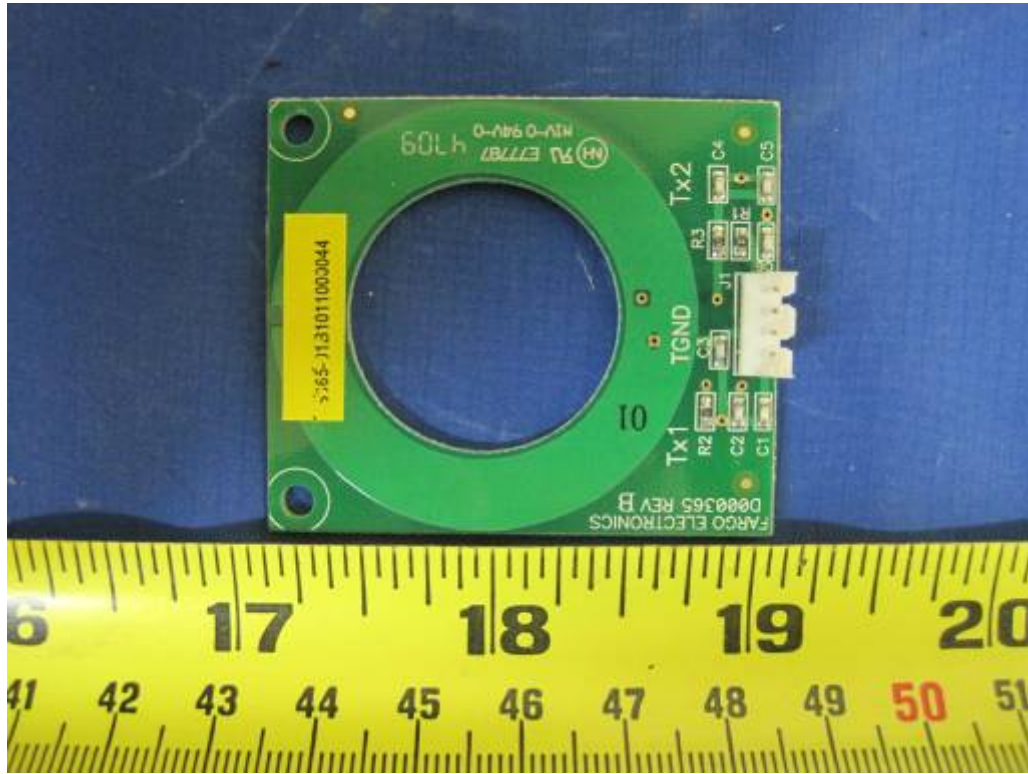
13.56MHz RFID Antenna Board (Laminator) Component View
