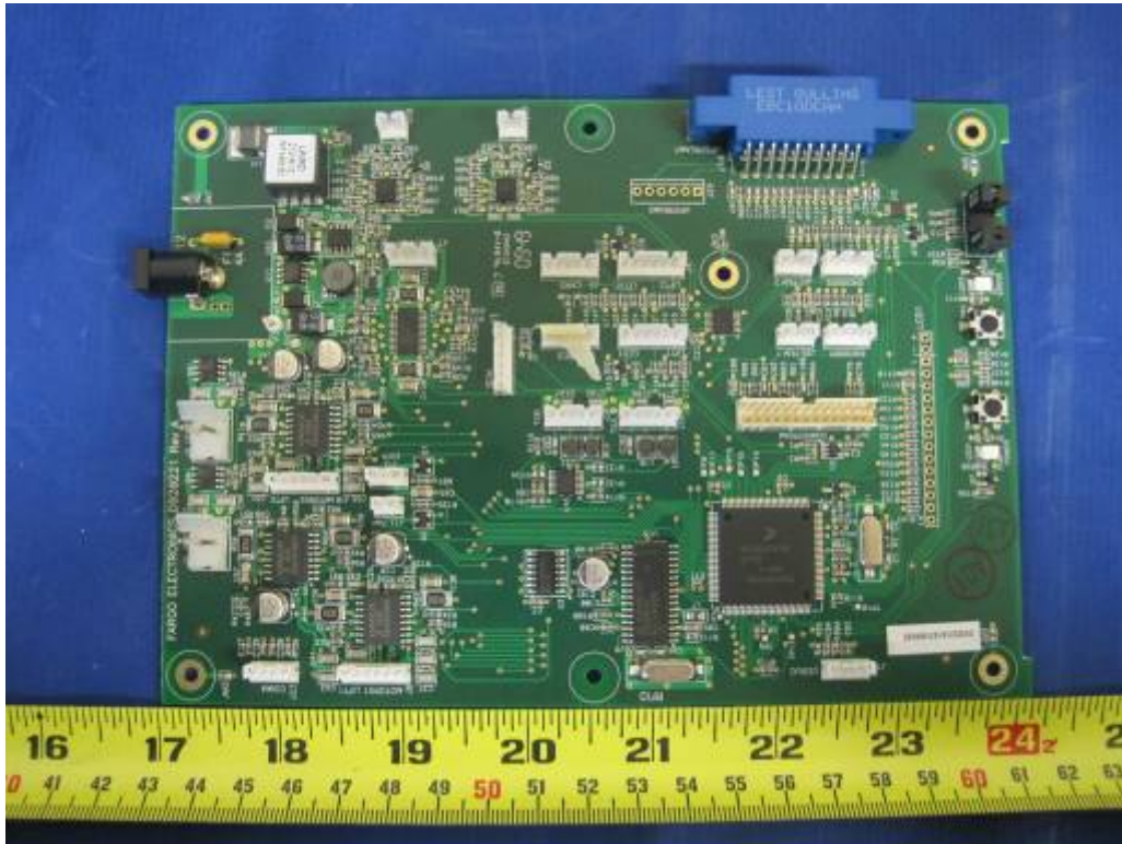
PCB 1 Component View ( Laminator RFID)
