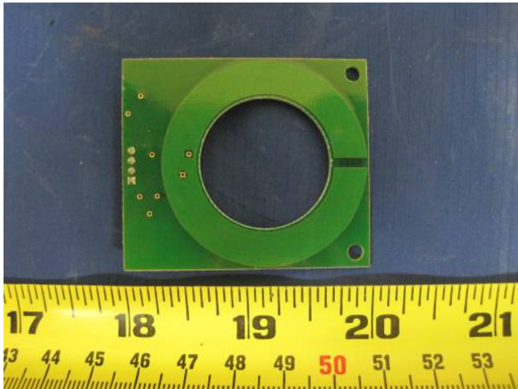
13.56MHz RFID Antenna Board (Laminator) Solder View
