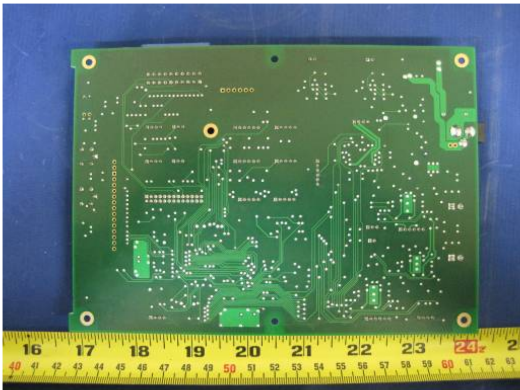
PCB 1 Solder View ( Laminator RFID)
