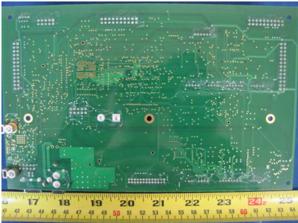
PCB 2 Solder View ( Ribbon RFID)
