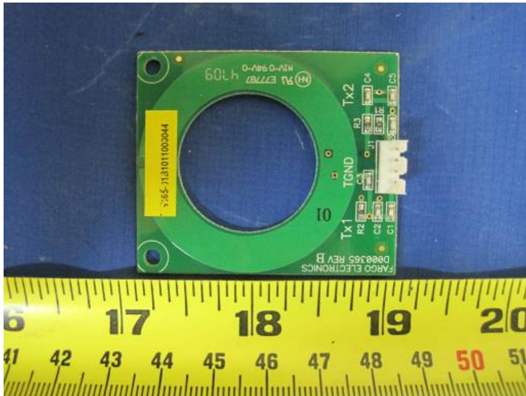
13.56MHz RFID Antenna Board (Ribbon) Component View
