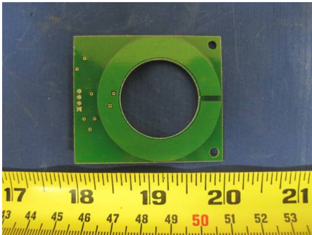
13.56MHz RFID Antenna Board (Ribbon) Solder View
