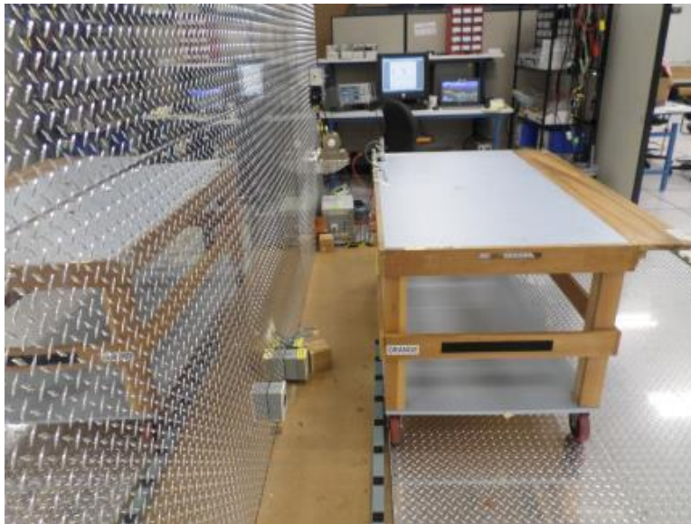
Figure 2: Conducted Emissions Limits, Pigtail, Back View, Test Setup
