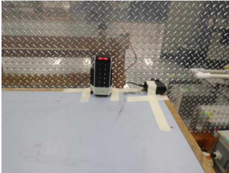
Figure 7: Conducted Emissions Limits, Terminal, EUT View, Test Setup
