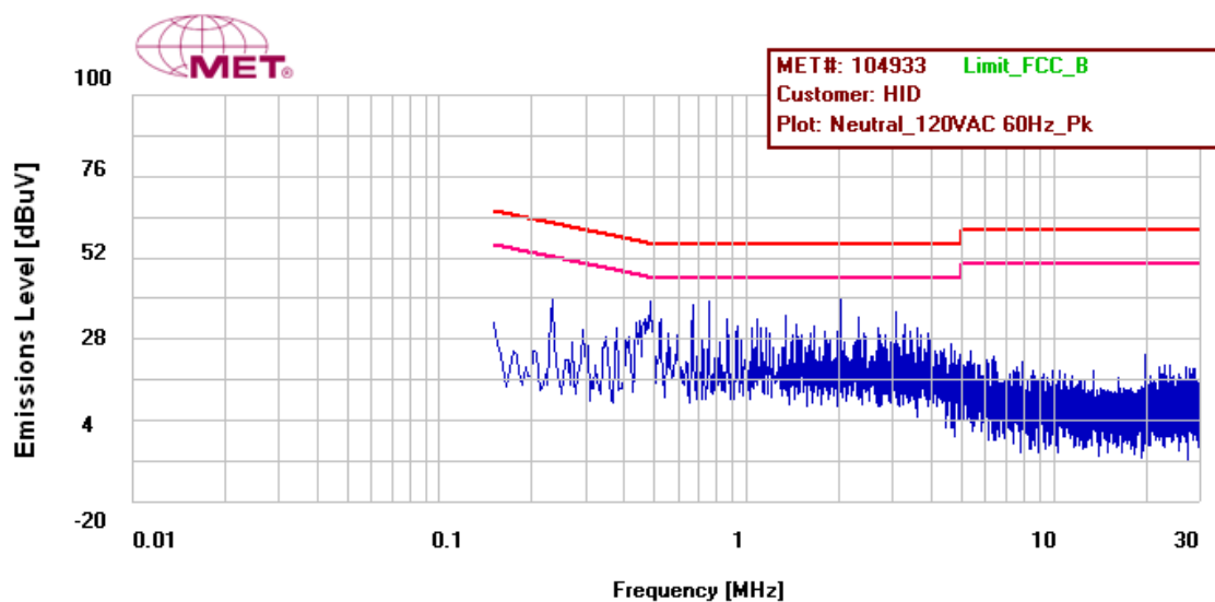
Figure 32: Conducted Emissions Limits, Terminal, Neutral Line, Prescan
