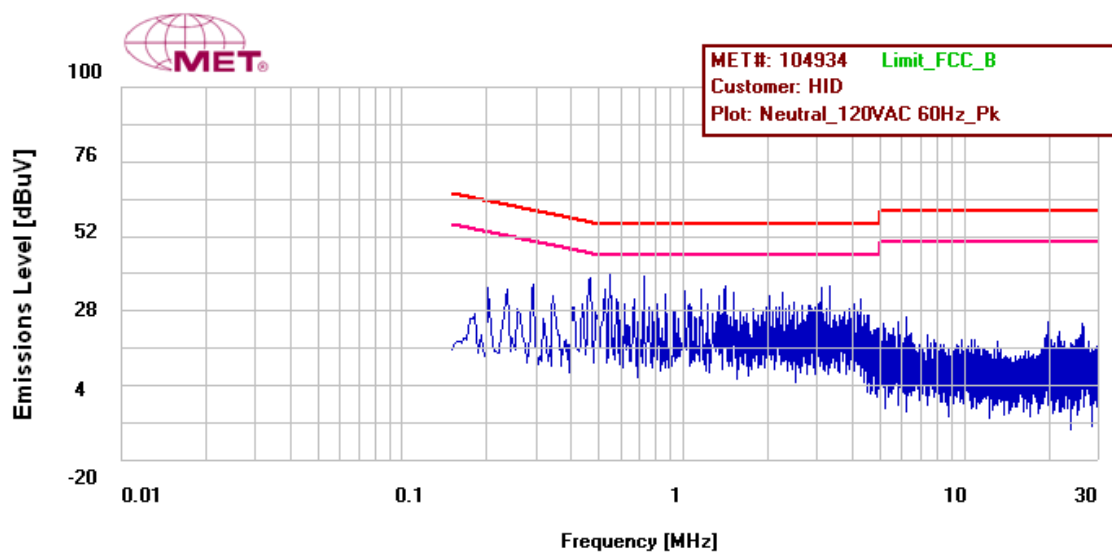
Figure 28: Conducted Emissions Limits, Pigtail, Neutral Line, Prescan
