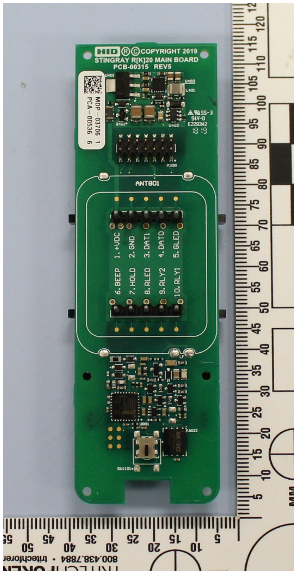
Model 20 (terminal version) main board reverse
