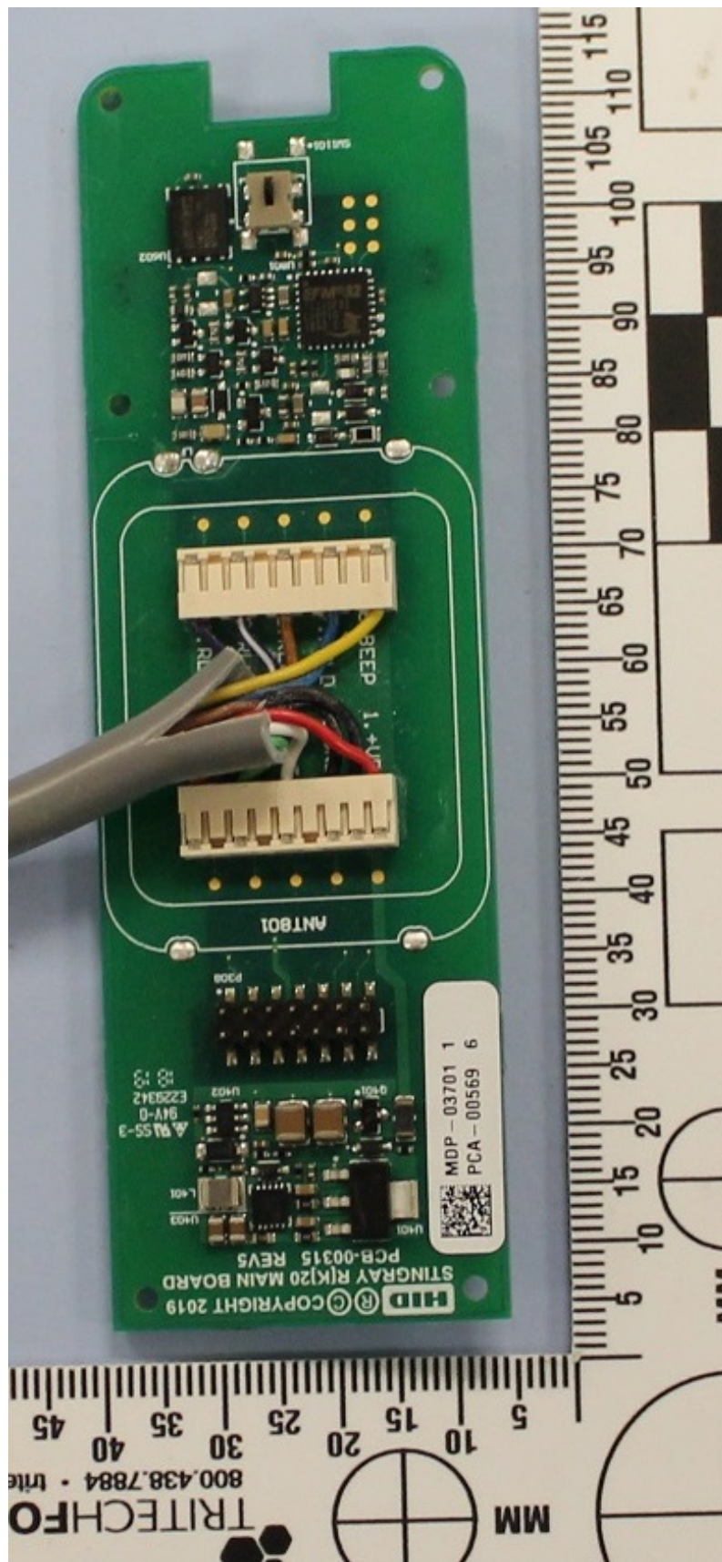
Model 20 (pigtail version) main board reverse detail
