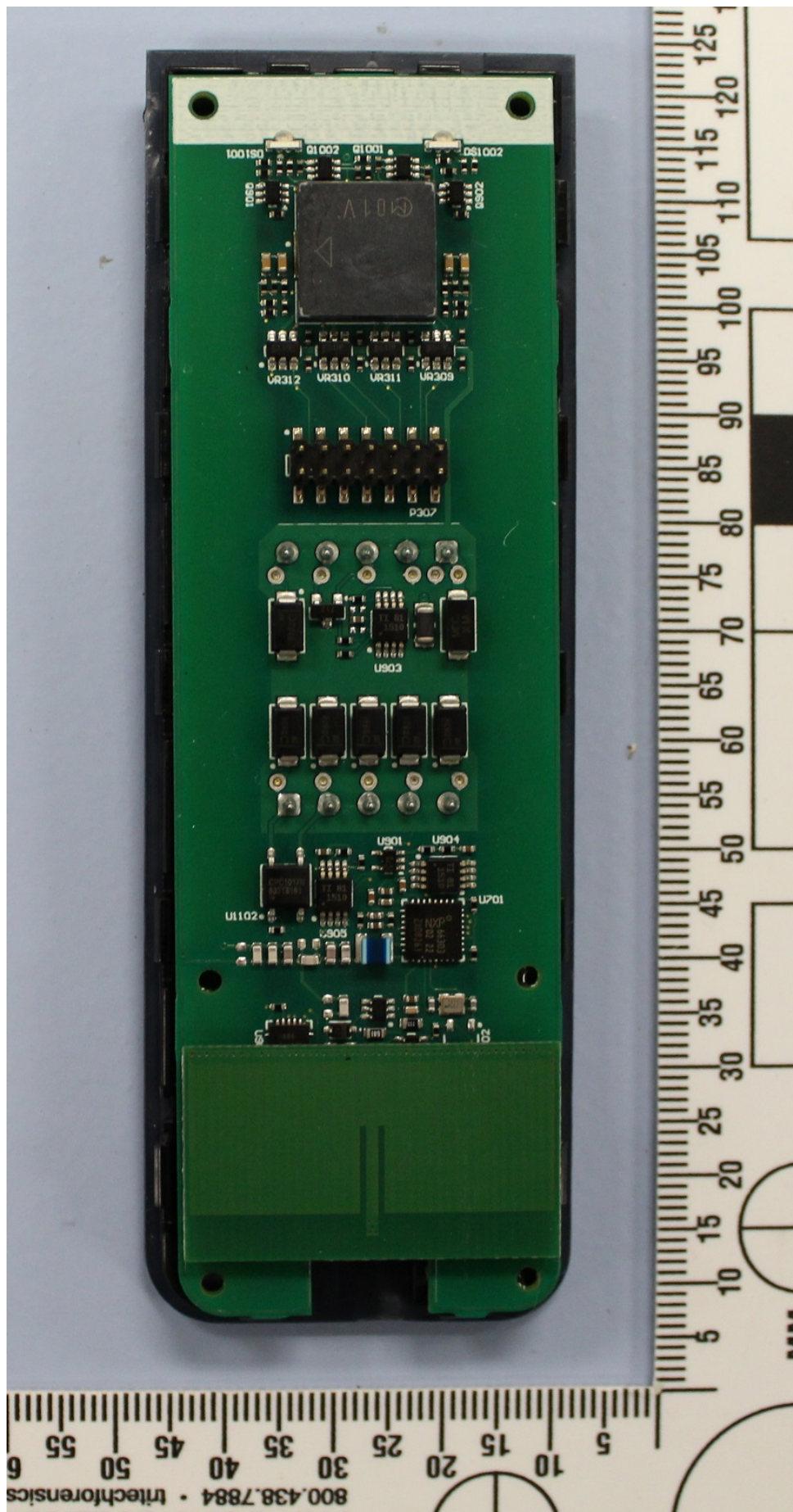
Model 20 (pigtail version) main board obverse with patch antenna
