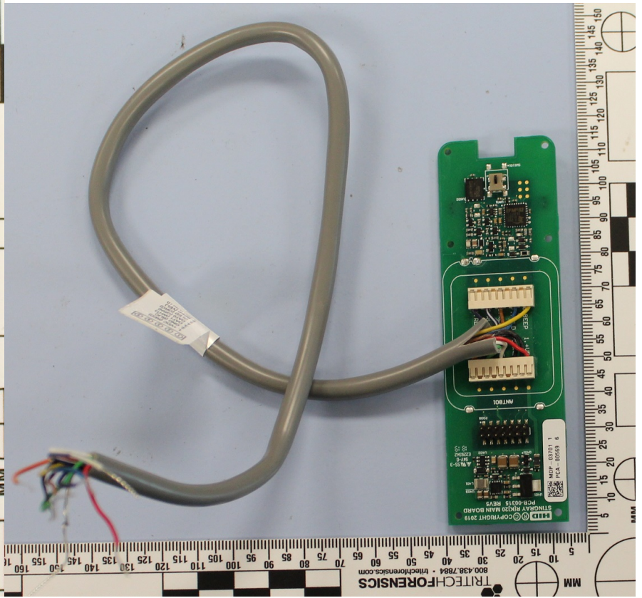
Model 20 (pigtail version) main board reverse
