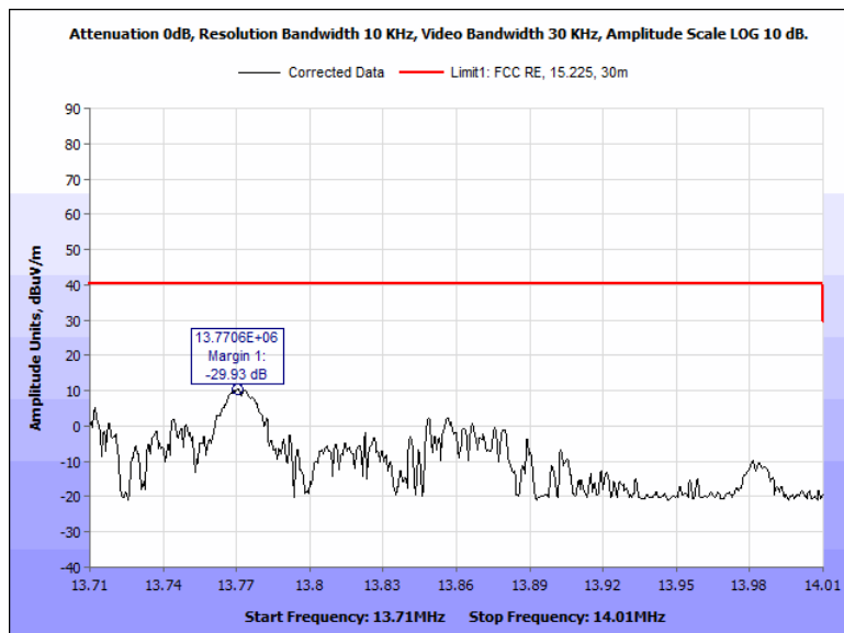
Figure 45: Spurious Emission Limits, within the bands 13.110 – 13.410 MHz and 13.710 – 14.010 MHz, Terminal, 13.710-14.010 MHz, 90 Deg
