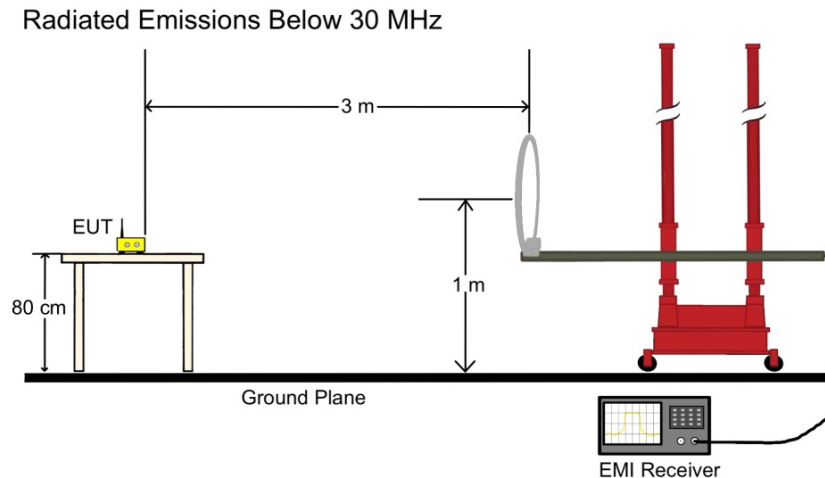
Figure 37: Radiated Emissions, Test Setup
