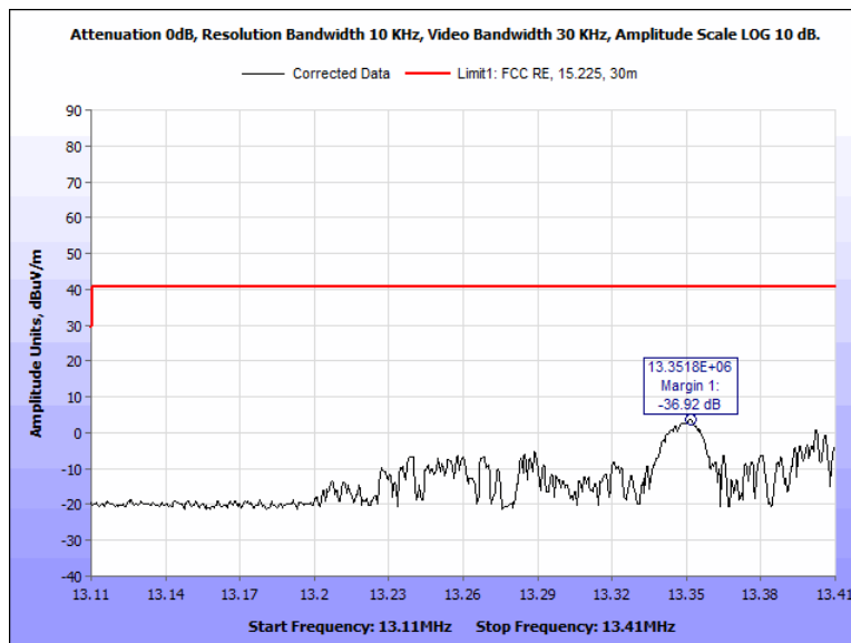
Figure 43: Spurious Emission Limits, within the bands 13.110 – 13.410 MHz and 13.710 – 14.010 MHz, Terminal, 13.110-13.410 MHz, 90 Deg
