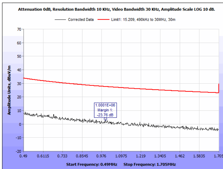
Figure 51: Spurious Emission Limits, outside the bands 13.110 – 14.010 MHz, Pigtail, 0.490 MHz – 1.705 MHz, 0 Deg
