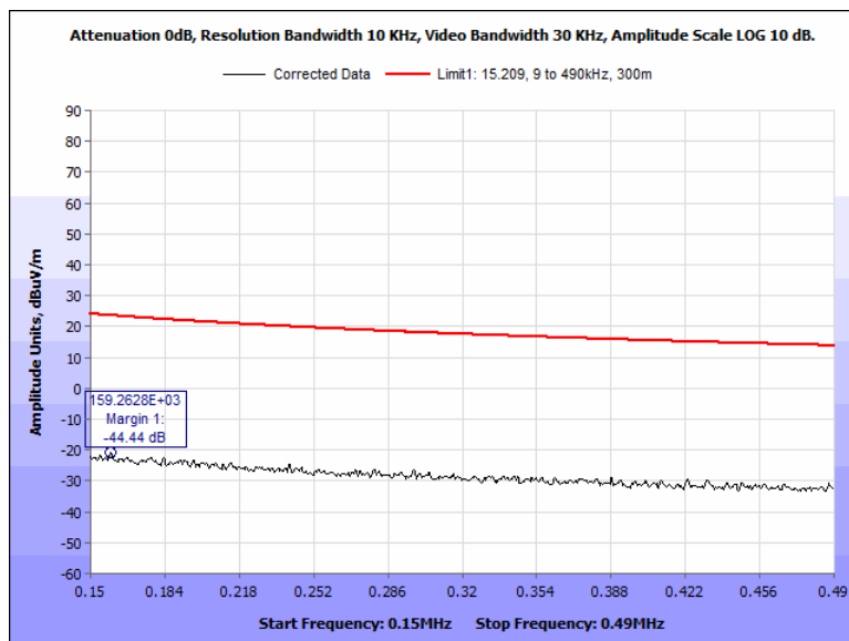
Figure 60: Spurious Emission Limits, outside the bands 13.110 – 14.010 MHz, Terminal, 0.150 MHz – 0.49 MHz, 0 Deg
