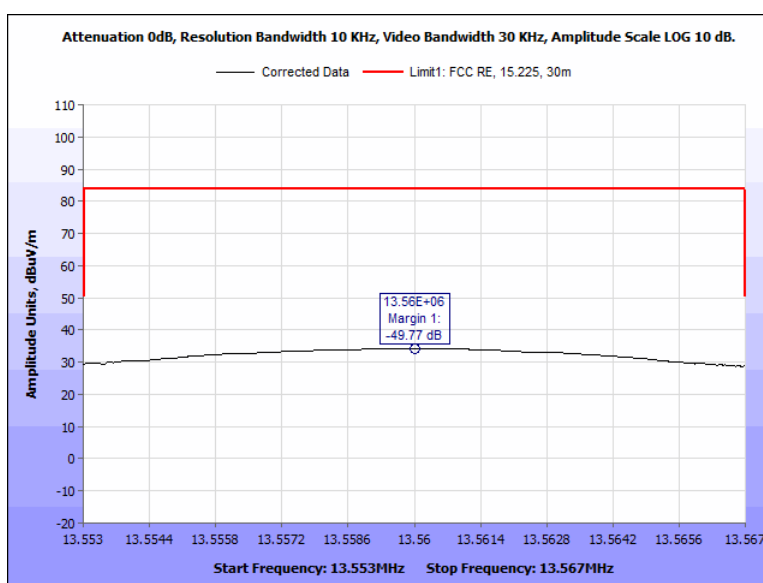
Figure 26: Spurious Emission Limits, within the band 13.553 – 13.567 MHz, Terminal, 0 Deg
