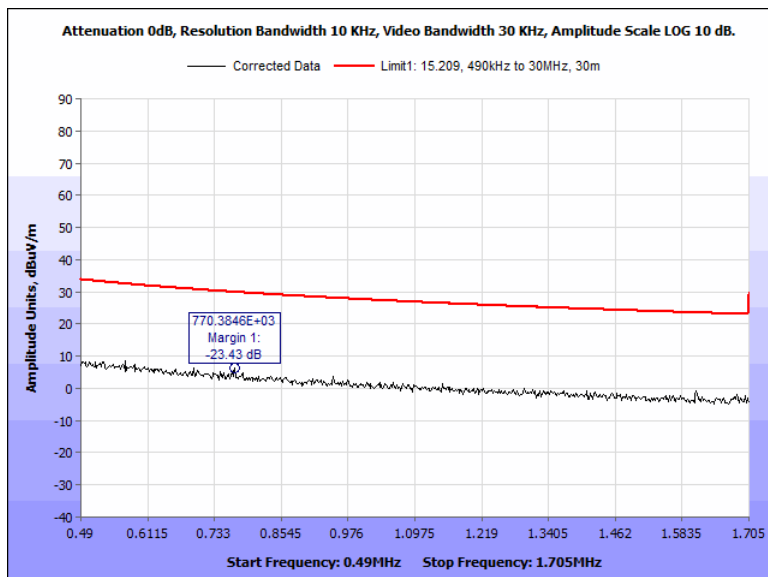
Figure 63: Spurious Emission Limits, outside the bands 13.110 – 14.010 MHz, Terminal, 0.490 – 1.705 MHz, 90 Deg
