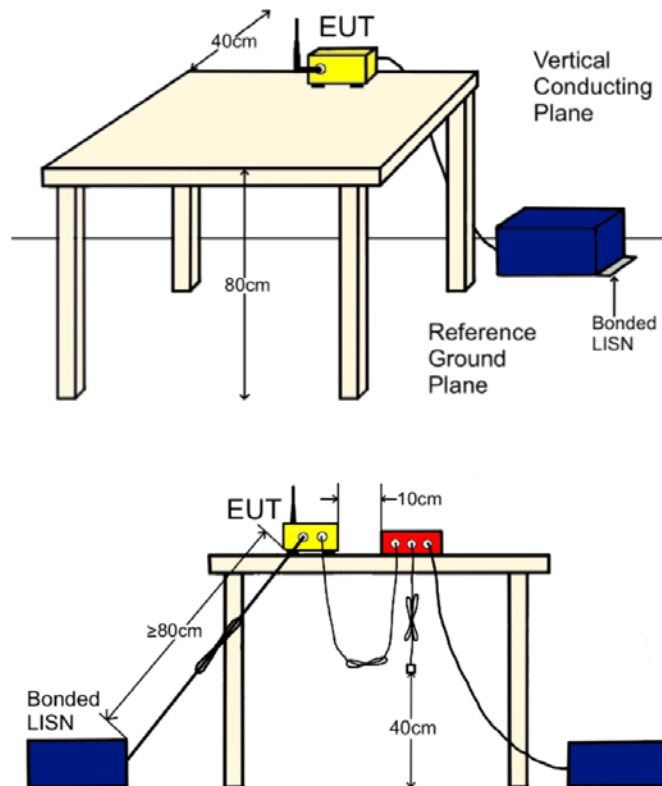
Figure 10: CEV Test Setup
