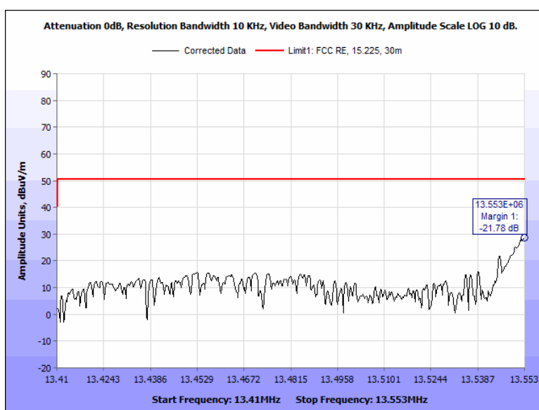
Figure 33: Spurious Emission Limits, within the bands 13.410 – 13.553 MHz and 13.567 – 13.710 MHz, Terminal, 13.410-13.553 MHz, 0 Deg
