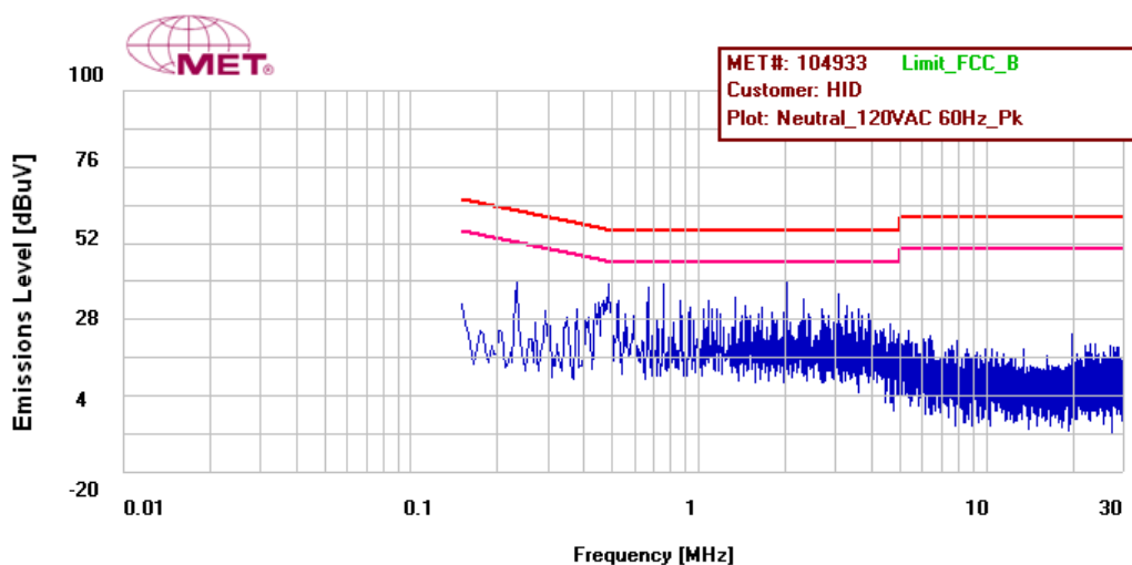
Figure 18: Conducted Emissions Limits, Terminal, Neutral Line, Prescan
