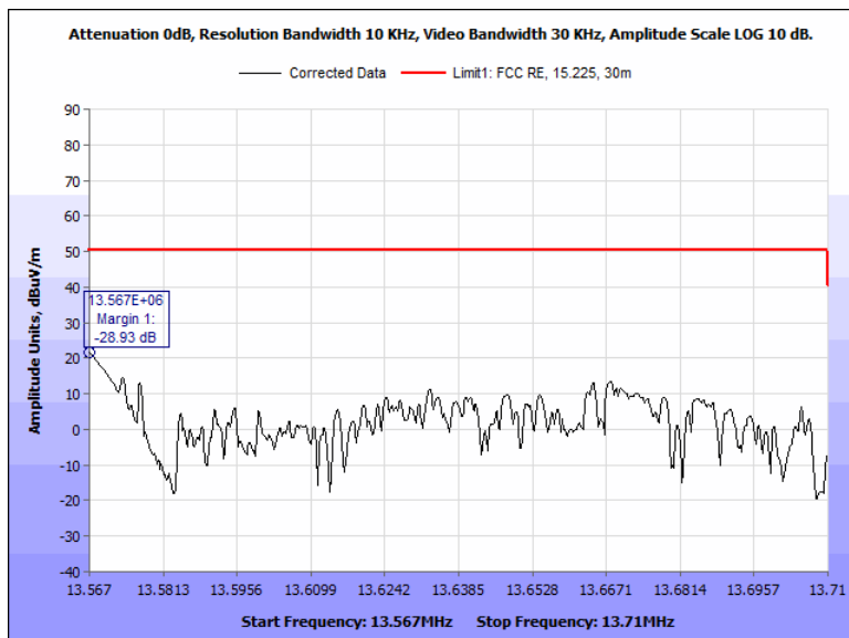
Figure 36: Spurious Emission Limits, within the bands 13.410 – 13.553 MHz and 13.567 – 13.710 MHz, Terminal, 13.567-13.710 MHz, 90 Deg
