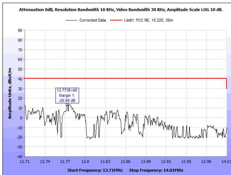
Figure 44: Spurious Emission Limits, within the bands 13.110 – 13.410 MHz and 13.710 – 14.010 MHz, Terminal, 13.710-14.010 MHz, 0 Deg
