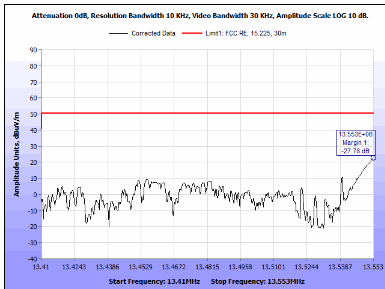
Figure 34: Spurious Emission Limits, within the bands 13.410 – 13.553 MHz and 13.567 – 13.710 MHz, Terminal, 13.410-13.553 MHz, 90 Deg
