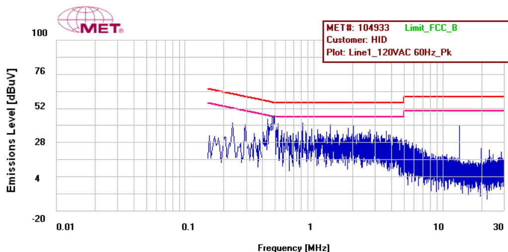
Figure 16: Conducted Emissions Limits, Terminal, Phase Line, Prescan
