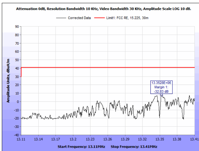
Figure 42: Spurious Emission Limits, within the bands 13.110 – 13.410 MHz and 13.710 – 14.010 MHz, Terminal, 13.110-13.410 MHz, 0 Deg
