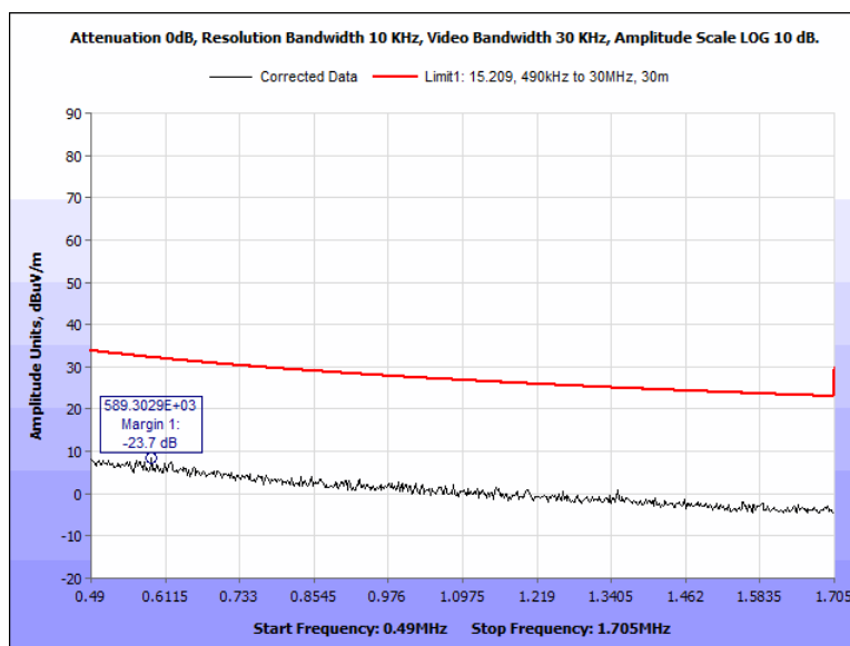
Figure 62: Spurious Emission Limits, outside the bands 13.110 – 14.010 MHz, Terminal, 0.490 MHz – 1.705 MHz, 0 Deg
