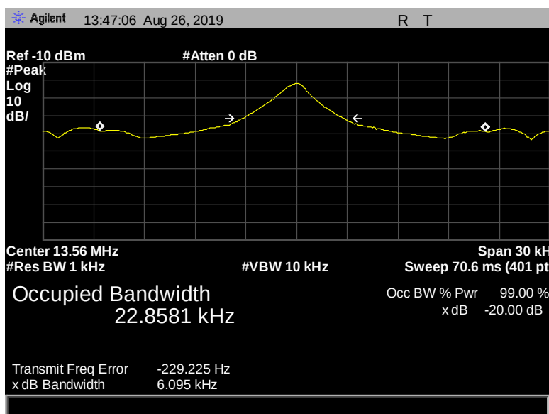
Figure 20: 20 dB Occupied Bandwidth, Pigtail, 20dB 6.095 KHz
