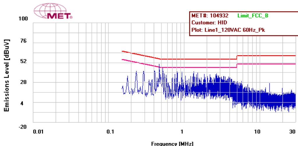
Figure 12: Conducted Emission Limits, Pigtail, Phase Line, Prescan
