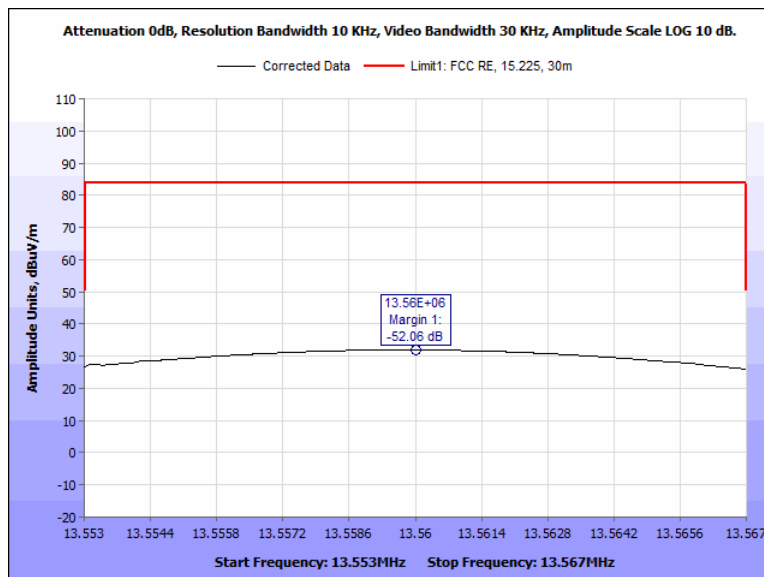
Figure 25: Spurious Emission Limits, within the band 13.553 – 13.567 MHz, Pigtail, 90 Deg
