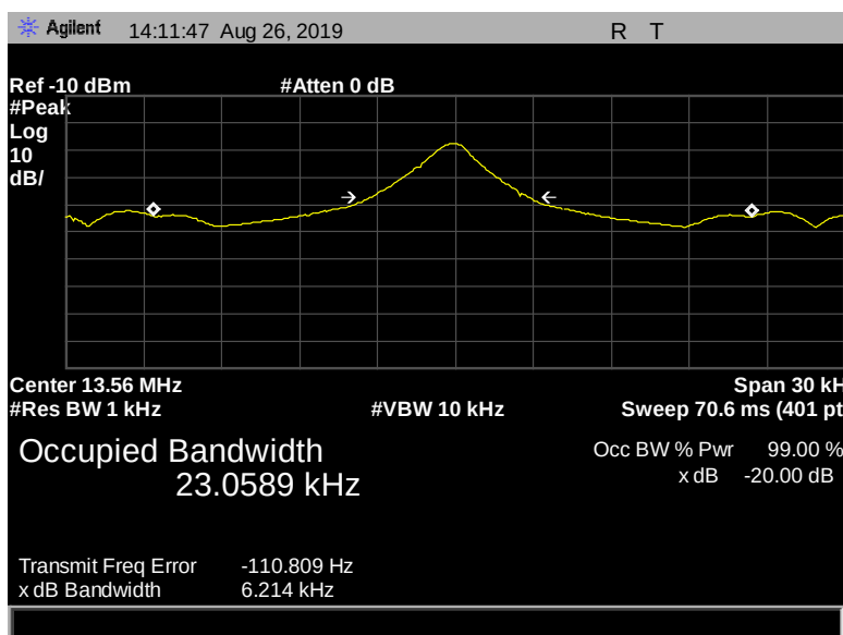
Figure 22: 20 dB Occupied Bandwidth, Terminal, -20dB 6.214 KHz
