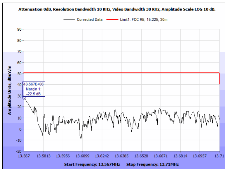
Figure 35: Spurious Emission Limits, within the bands 13.410 – 13.553 MHz and 13.567 – 13.710 MHz, Terminal, 13.567-13.710 MHz, 0 Deg
