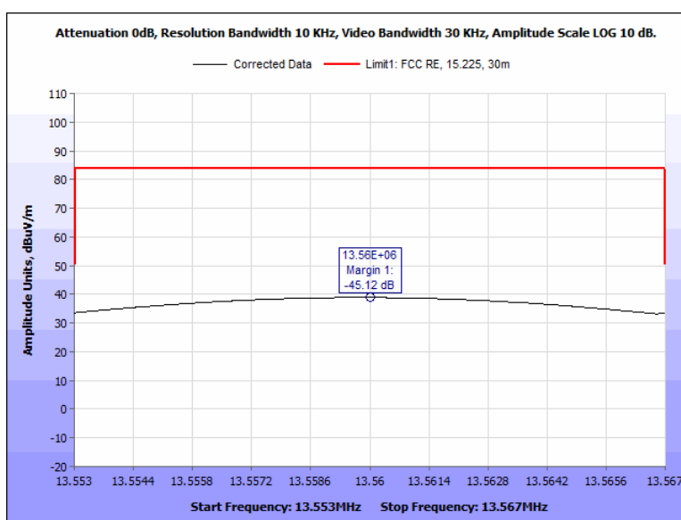
Figure 24: Spurious Emission Limits, within the band 13.553 – 13.567 MHz, Pigtail, 0 Deg
