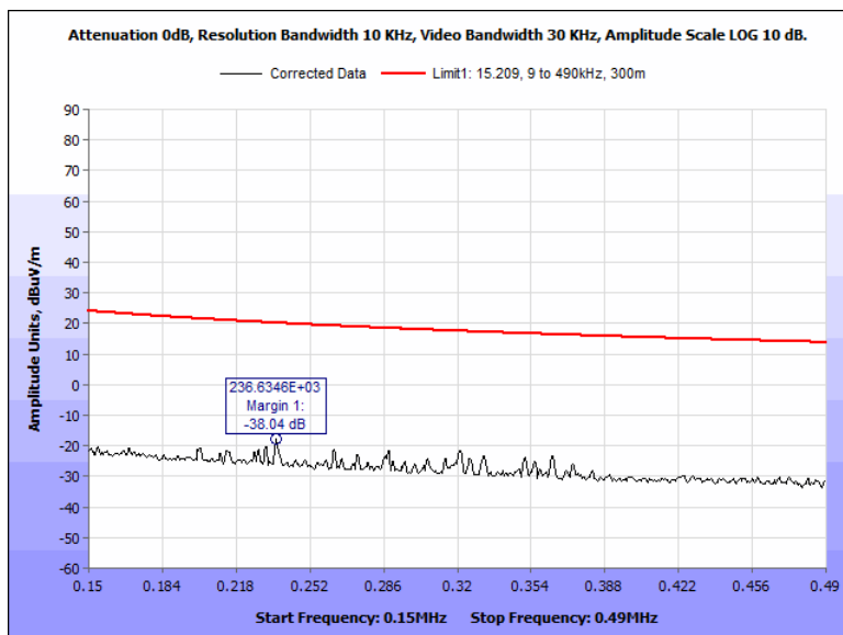
Figure 49: Spurious Emission Limits, outside the bands 13.110 – 14.010 MHz, Pigtail, 0.150 MHz – 0.490 MHz, 0 Deg
