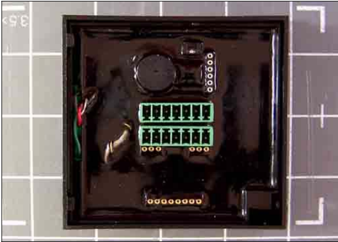
Back Plate Removed – Potted – 6111B
