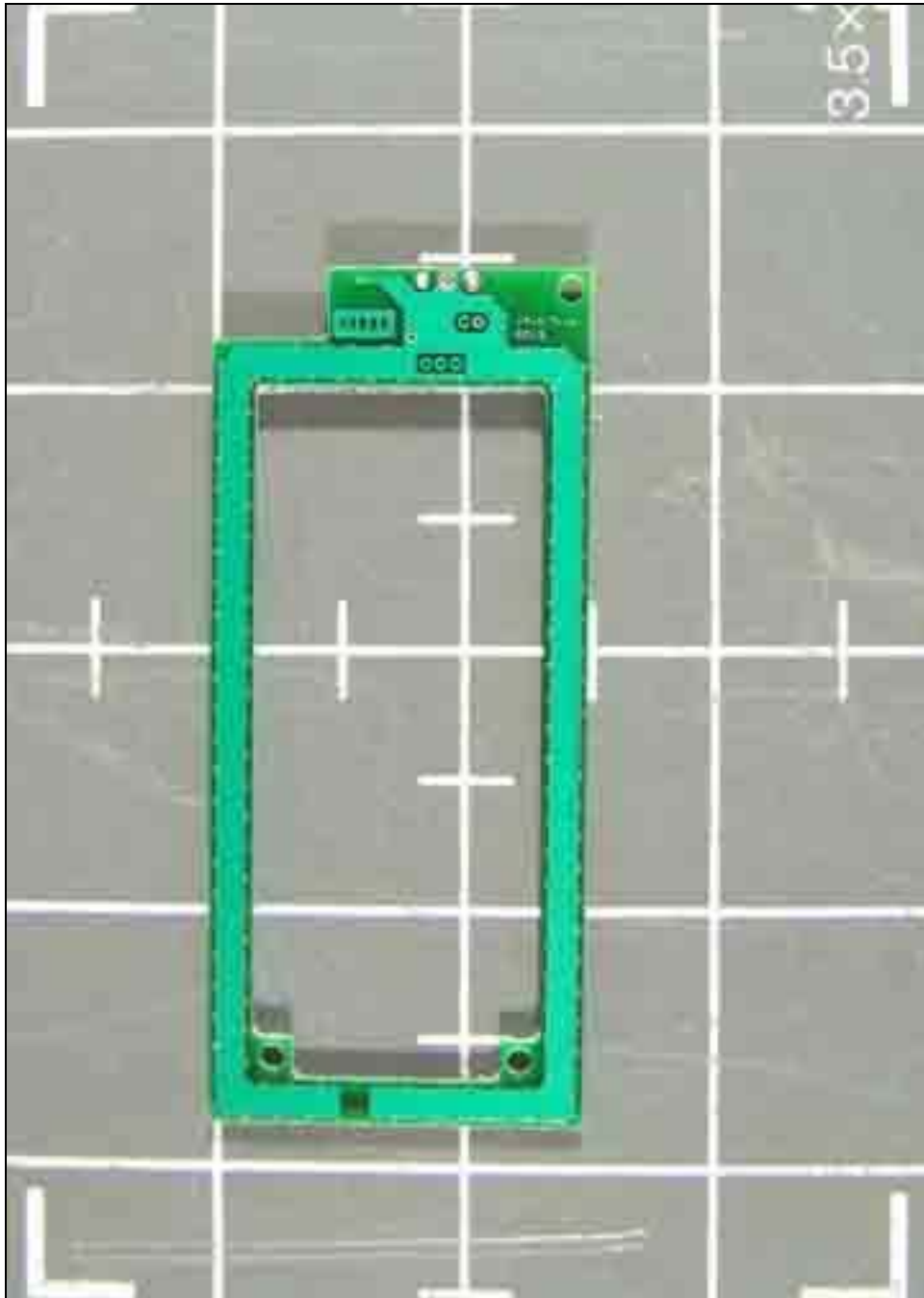
Antenna PCB Back – 6101B
