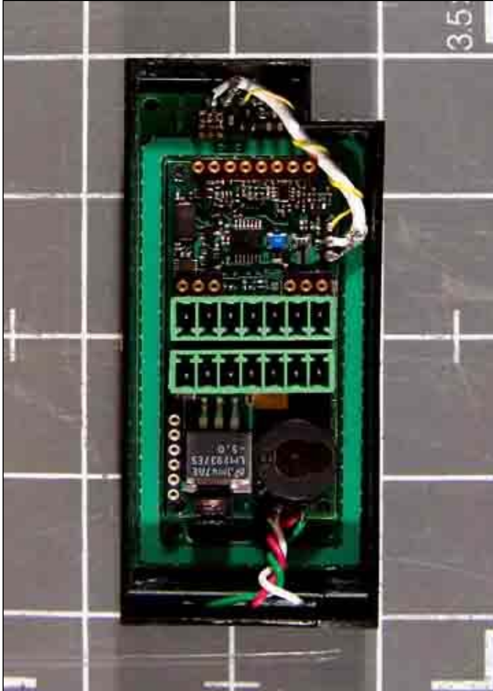
Interior Overall – Daughter PCB Removed – 6101B
