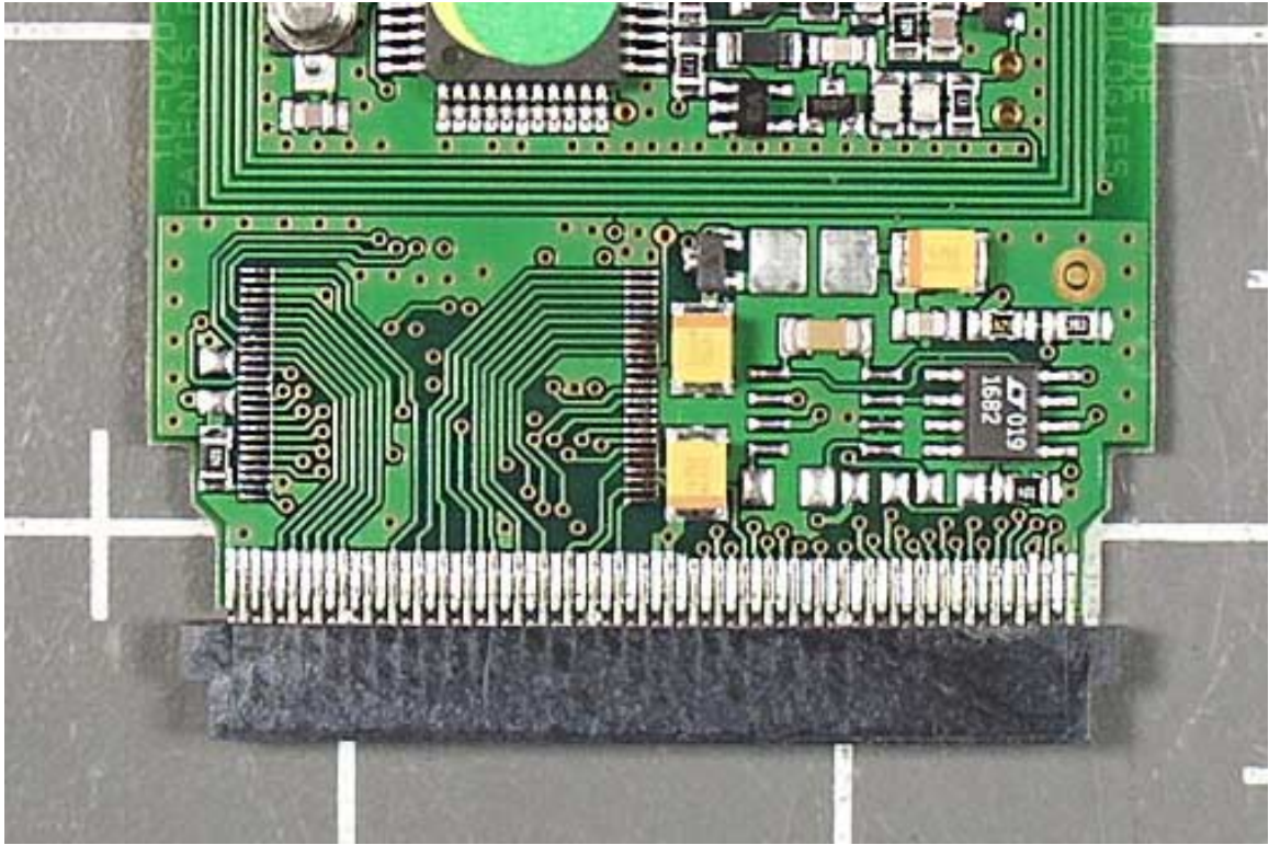
PCB 1 Closeup 1
