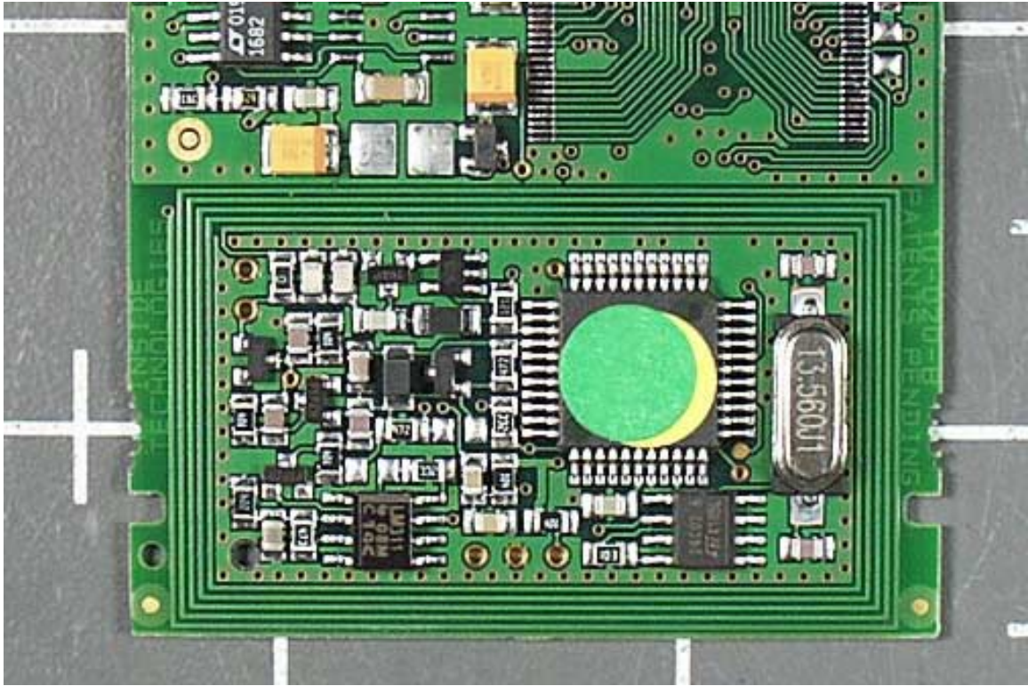
PCB 1 Closeup 2
