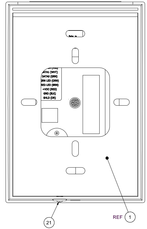
BACK VIEW ITEM 7 (MOUNTING PLATE) SHOWN
