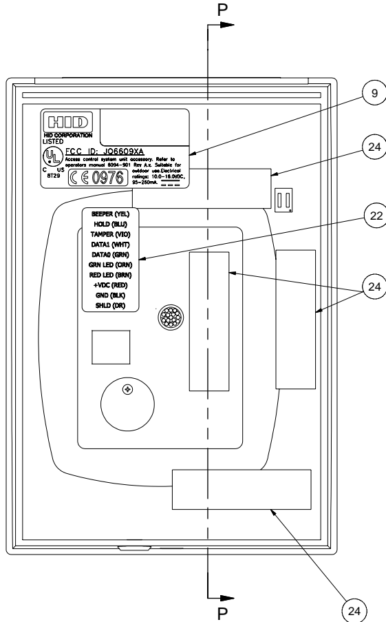
BACK VIEW ITEM 1 (MOUNTING PLATE) NOT SHOWN
