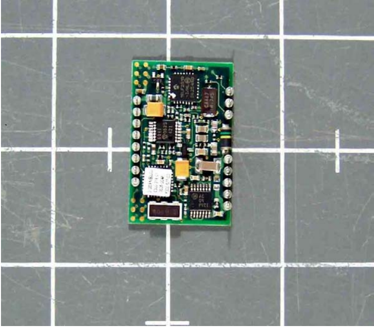
125 kHz Expansion PCB Front Models A & N
