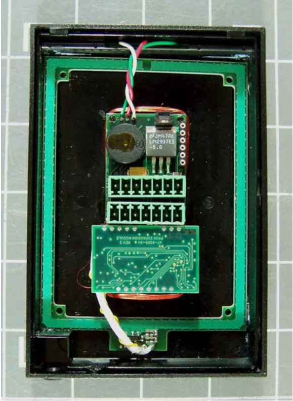
Internal Overall Model A & N
