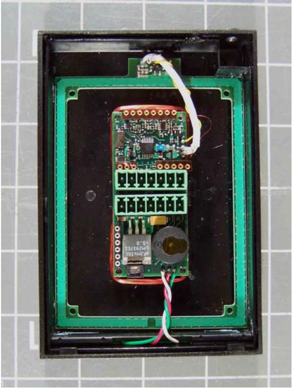
Interior Overall without Expansion PCB
