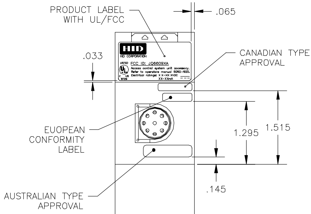
FRONT VIEW SHOWN WITHOUT BEZEL FOR CLARITY
