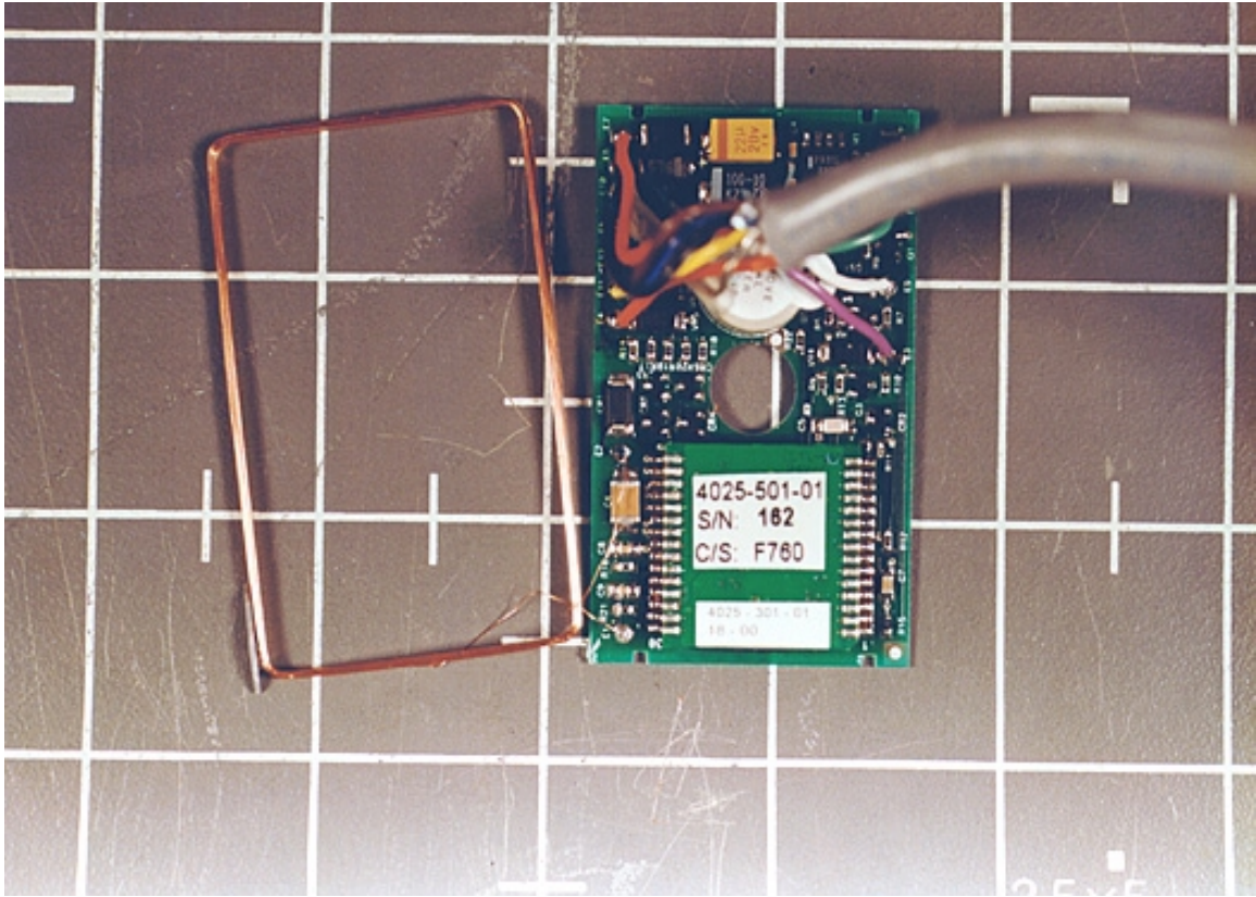
MODEL: 6005/8B BOARD AND ANTENNA REMOVED
