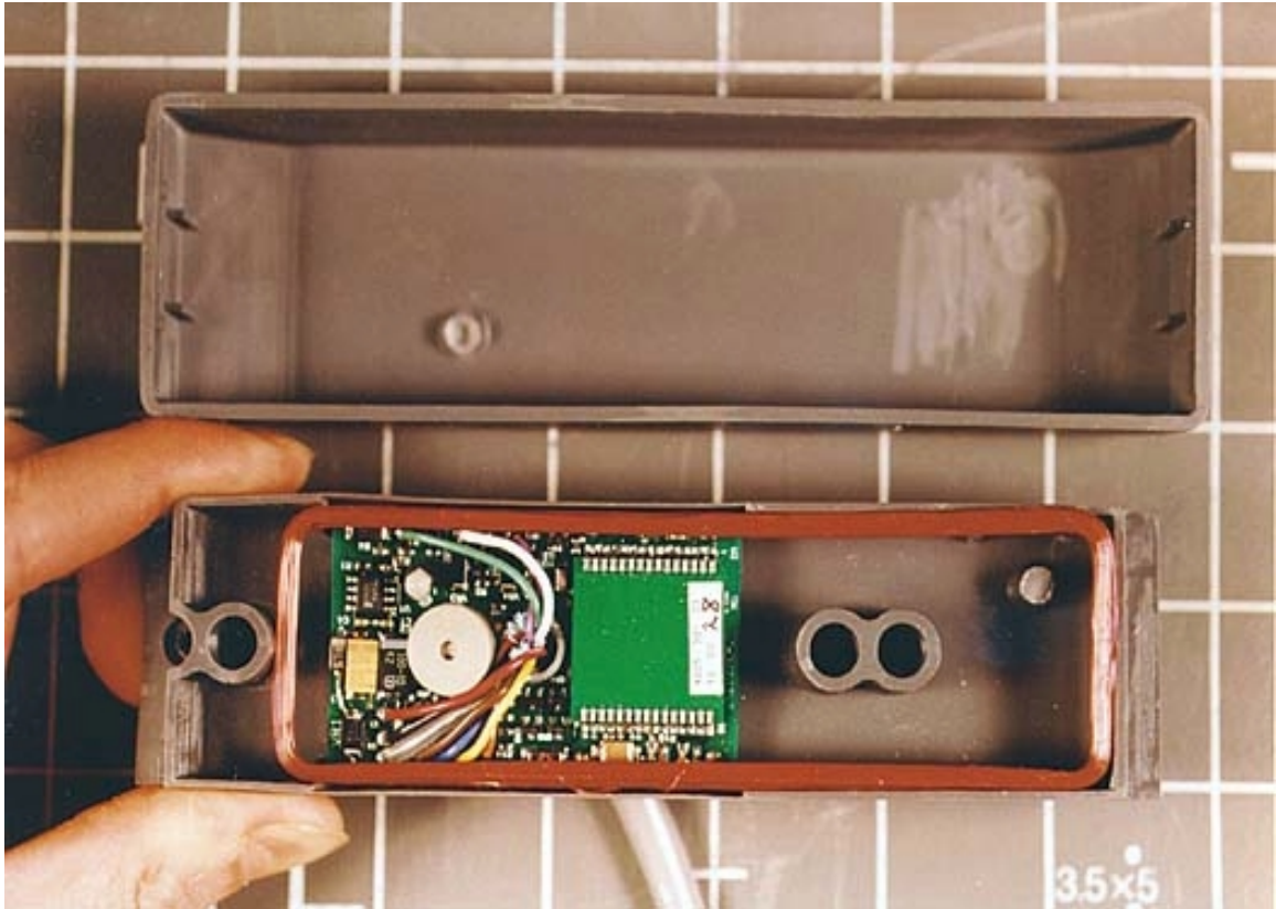
MODEL: 5365/8E INSIDE WITH FRONT COVER REMOVED
