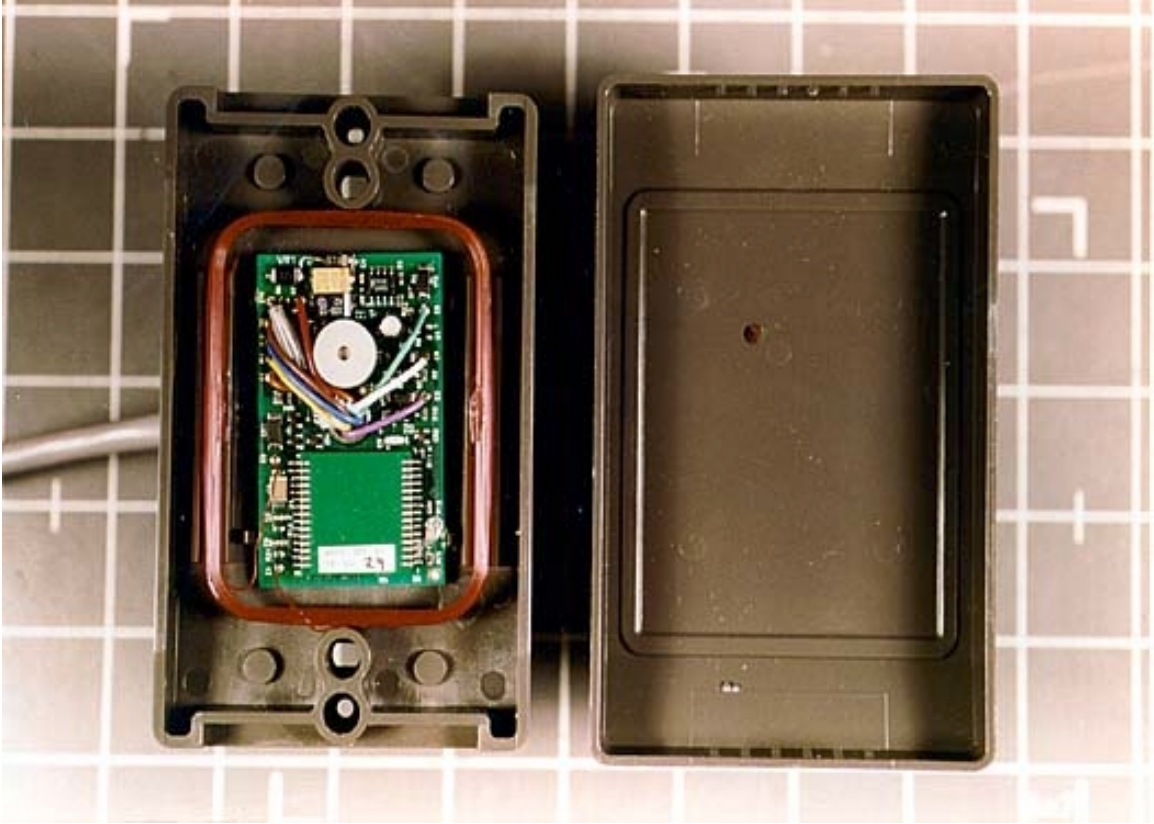
MODEL: 5395/8C INSIDE WITH FRONT COVER REMOVED
