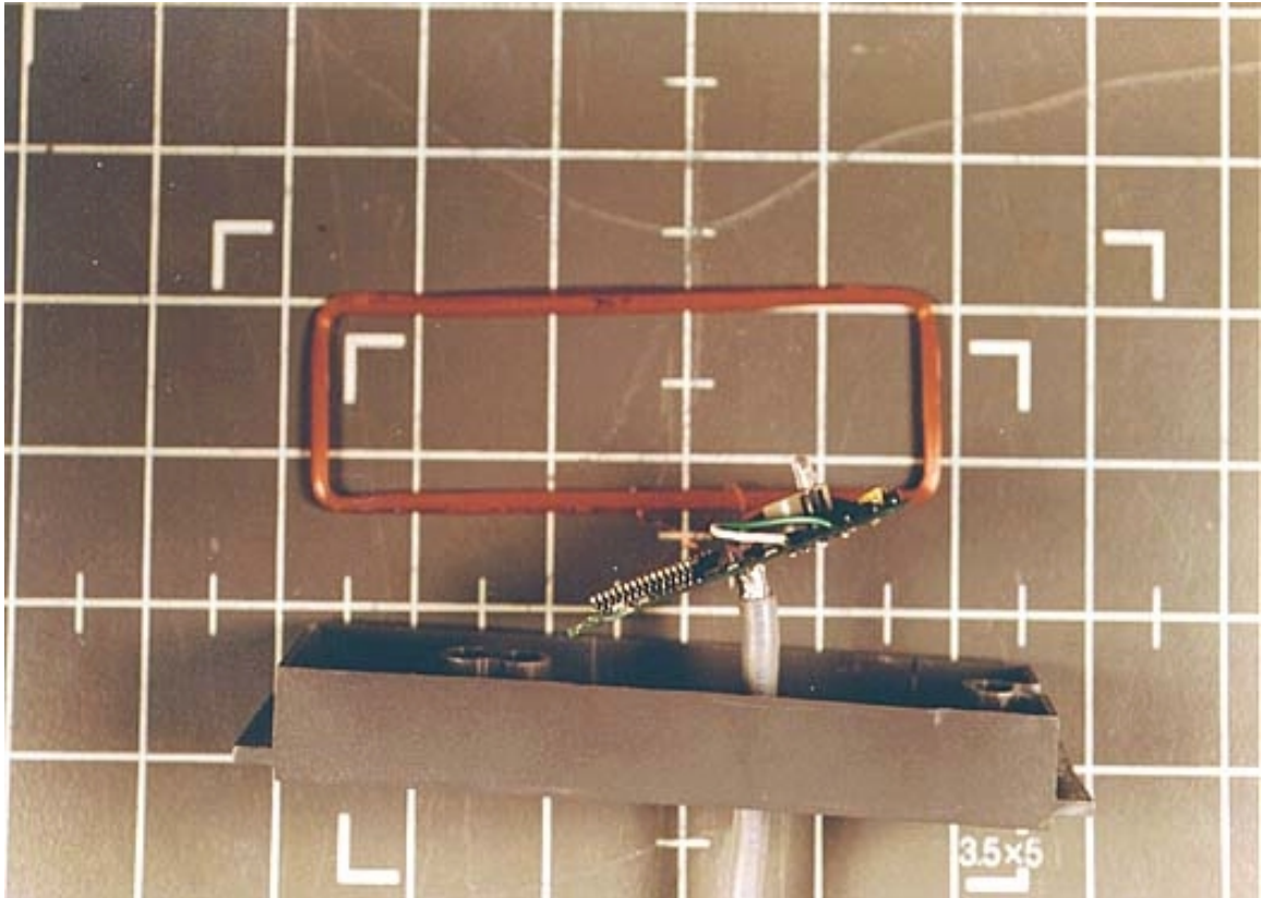
INSIDE TOP WITH ANTENNA REMOVED
