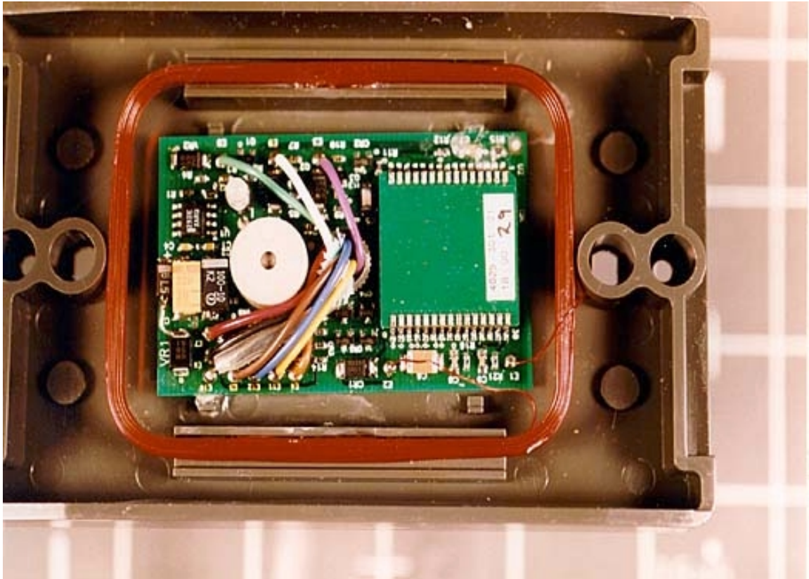
MODEL: 5395/8C INSIDE TOP
