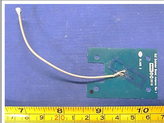
Antenna View 1
