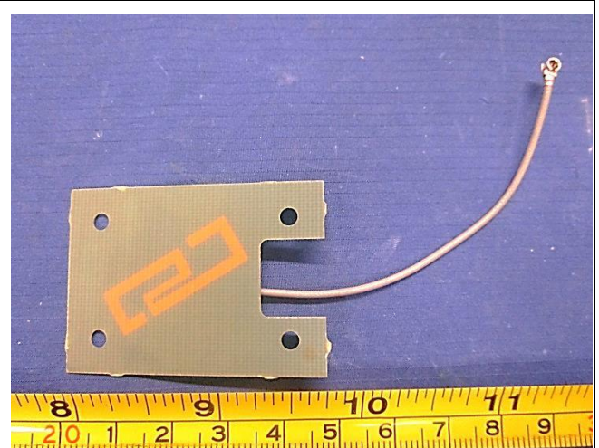
Antenna View 2
