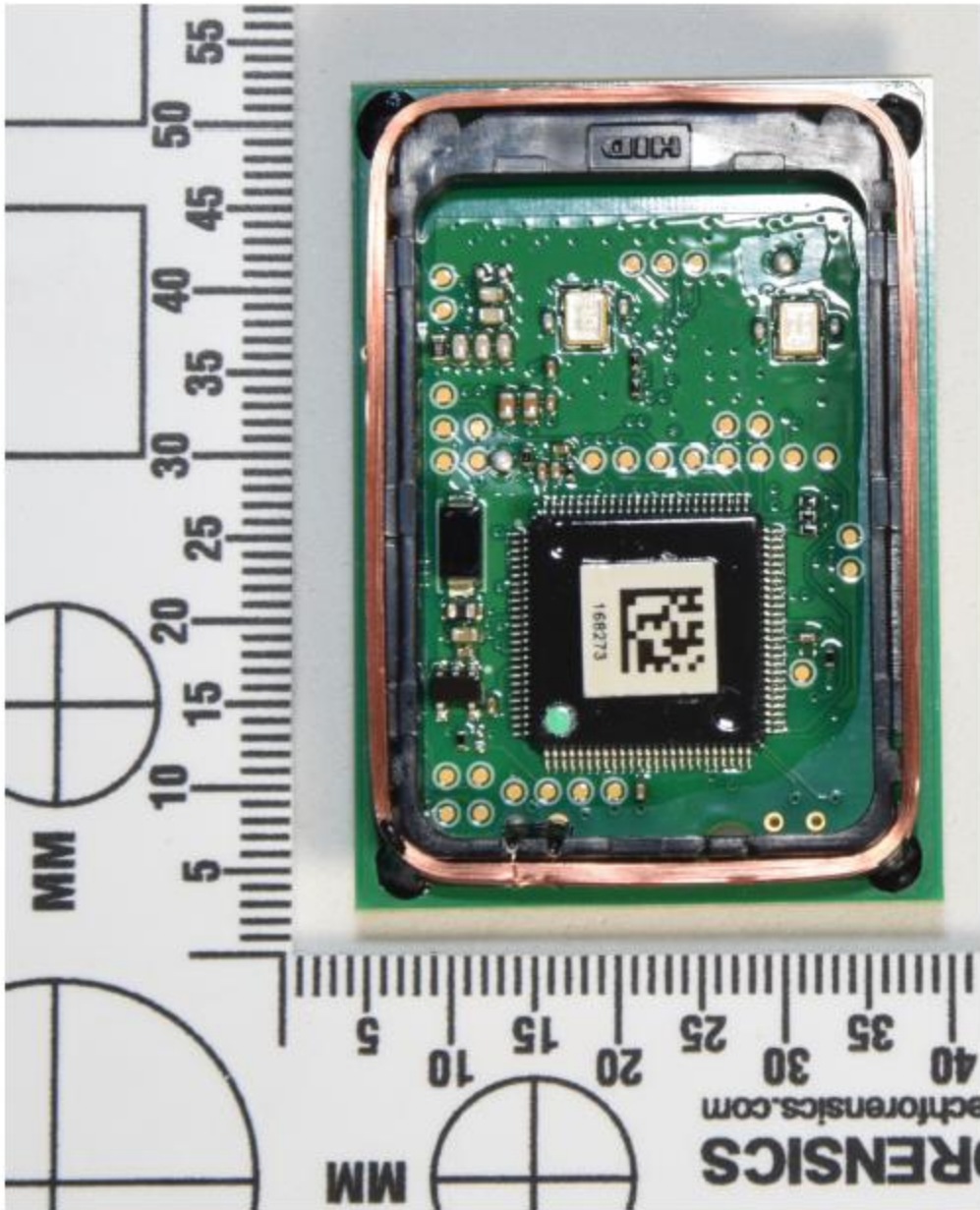
Input hopper OMNIKEY 5127CK MINI, bottom side
