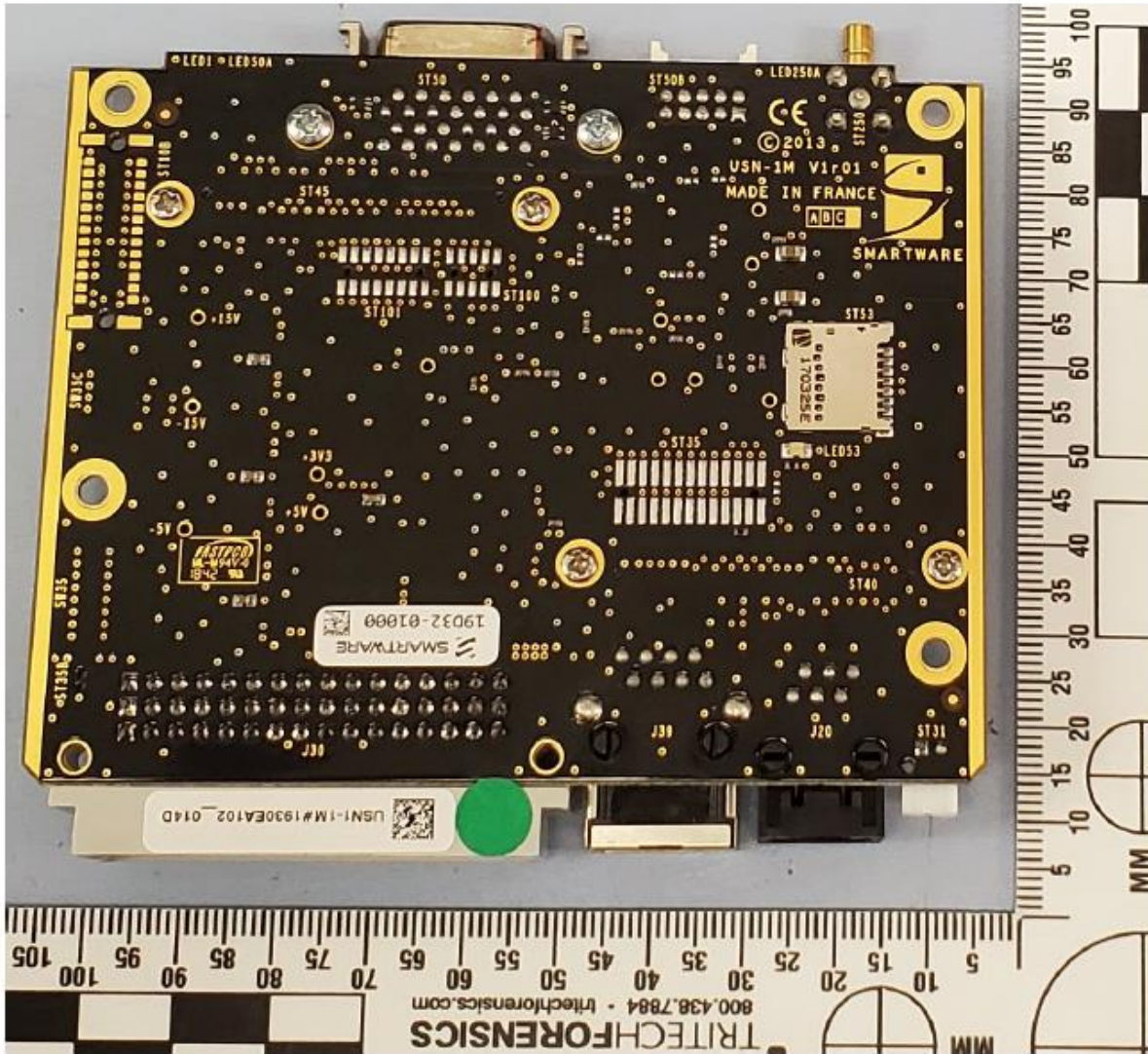
Encoder module Smartware® USN1se-1M radio, bottom side
