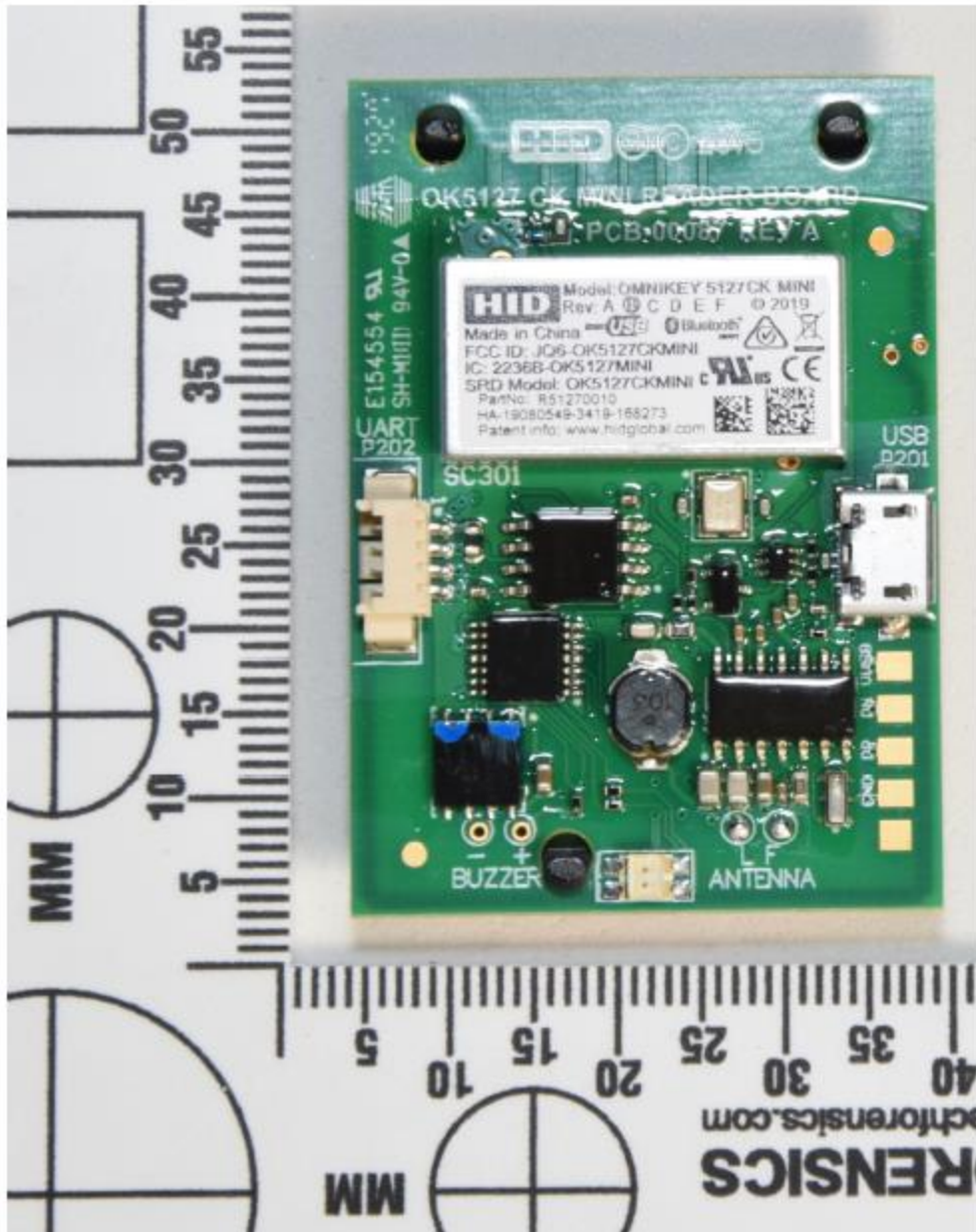
Input hopper OMNIKEY 5127CK MINI, top side
