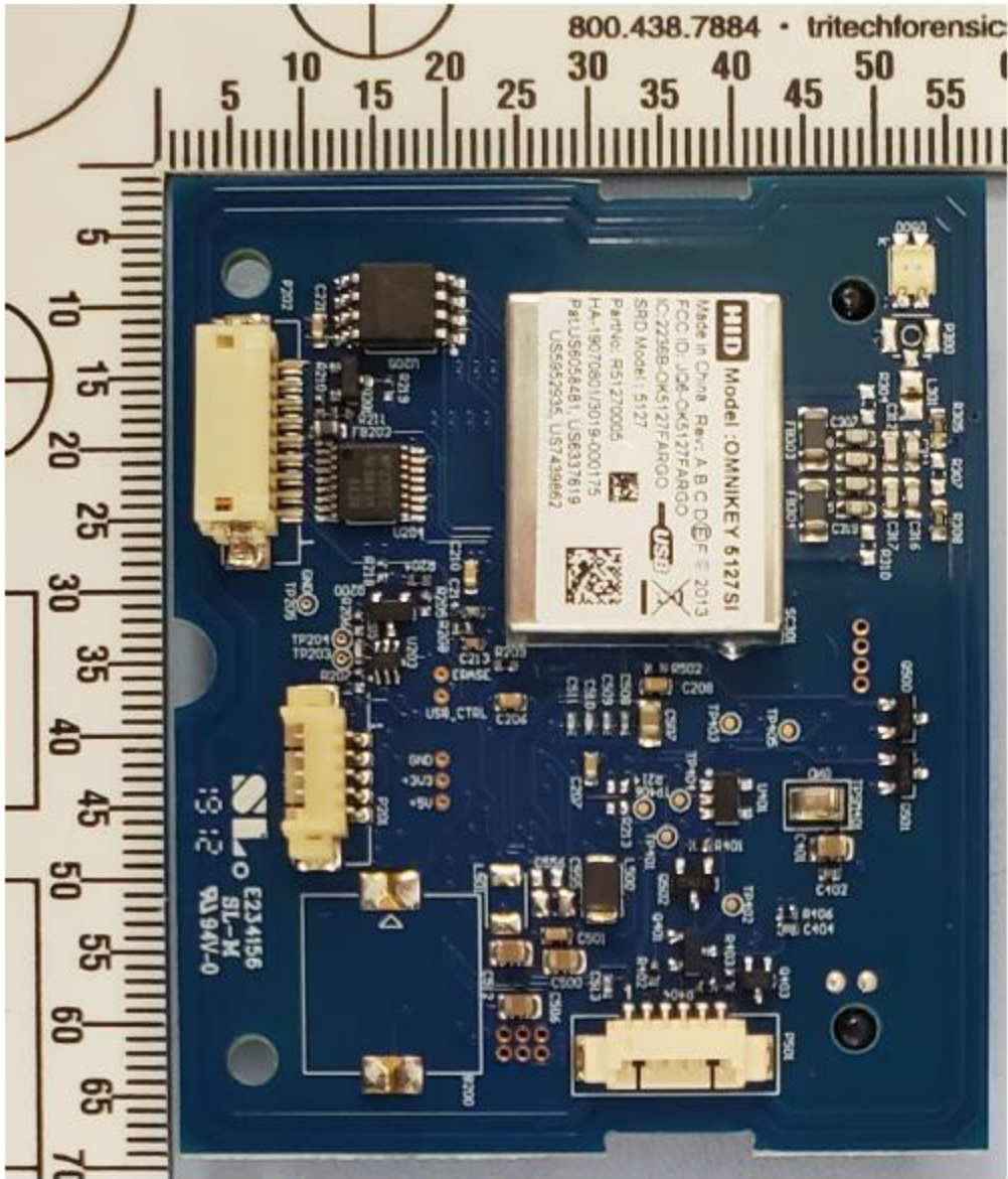
Input hopper OMNIKEY 5127CK SI, bottom side
