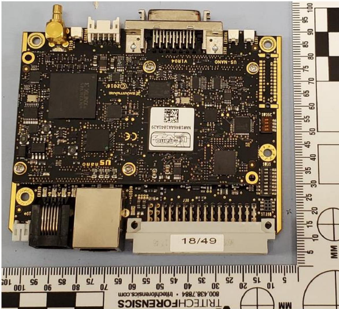
Encoder module Smartware® USN1se-1M radio, top side
