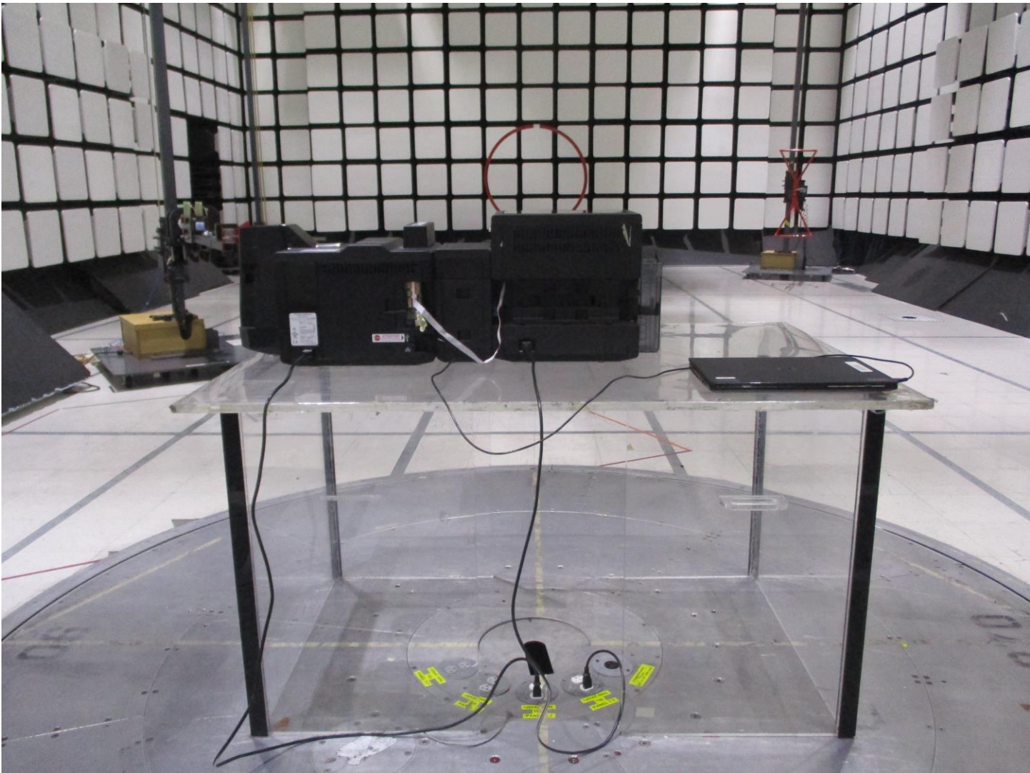
Photograph 6. Radiated Emissions, 9 kHz to 30 MHz, Rear View
