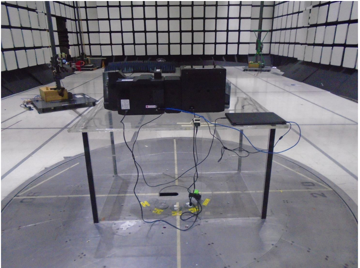
Photograph 3. REE 30-1000 MHz Rear View
