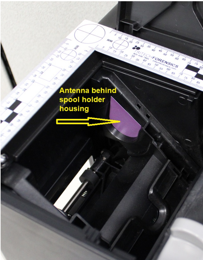
Left side spool housing antenna location
