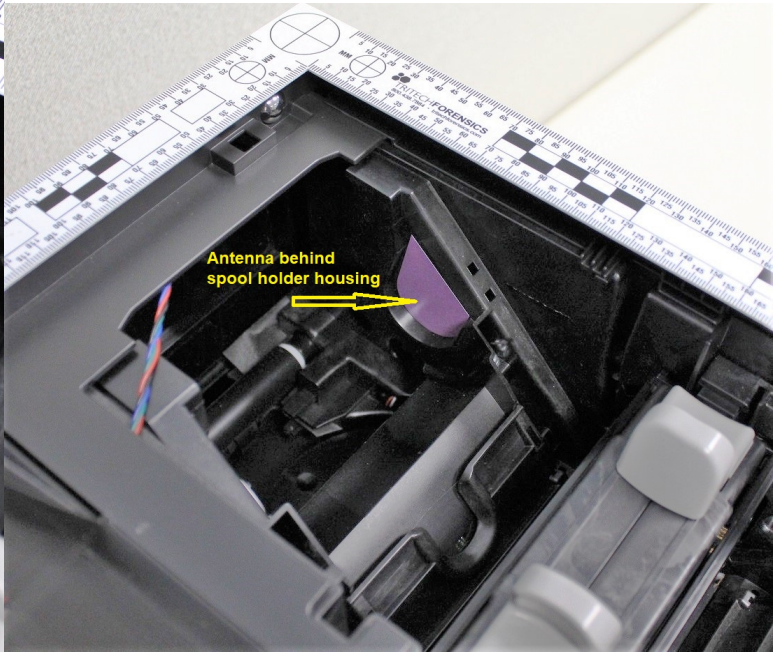
Right side spool housing antenna location
