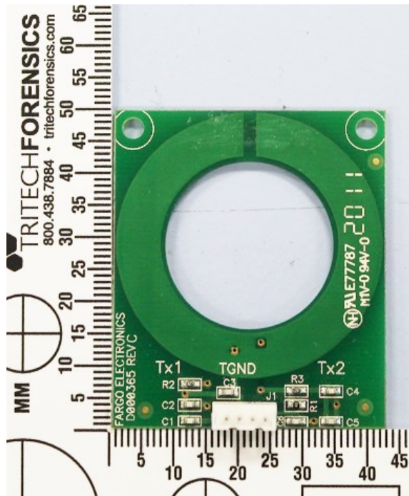
HDP6600 Laminator Accessory spool antenna board
