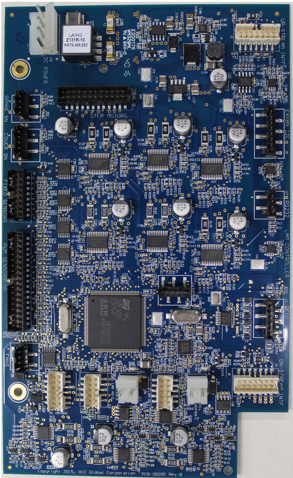
HDP6600 Laminator Accessory main board, high resolution
