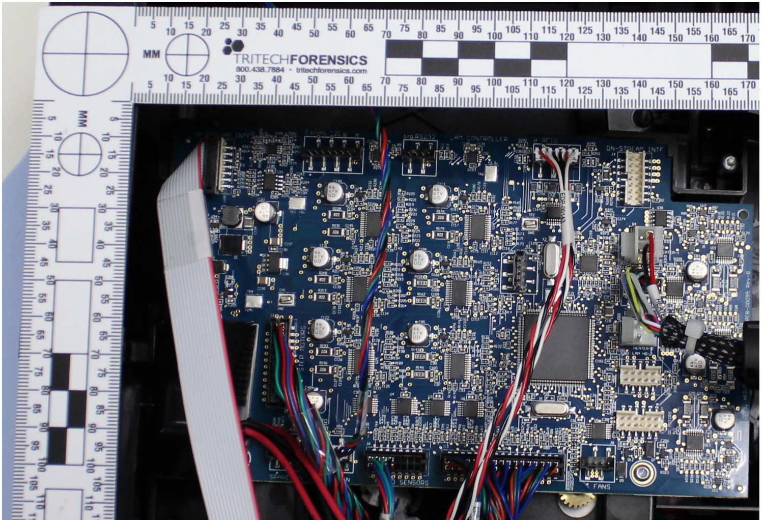
HDP6600 Laminator Accessory main board
