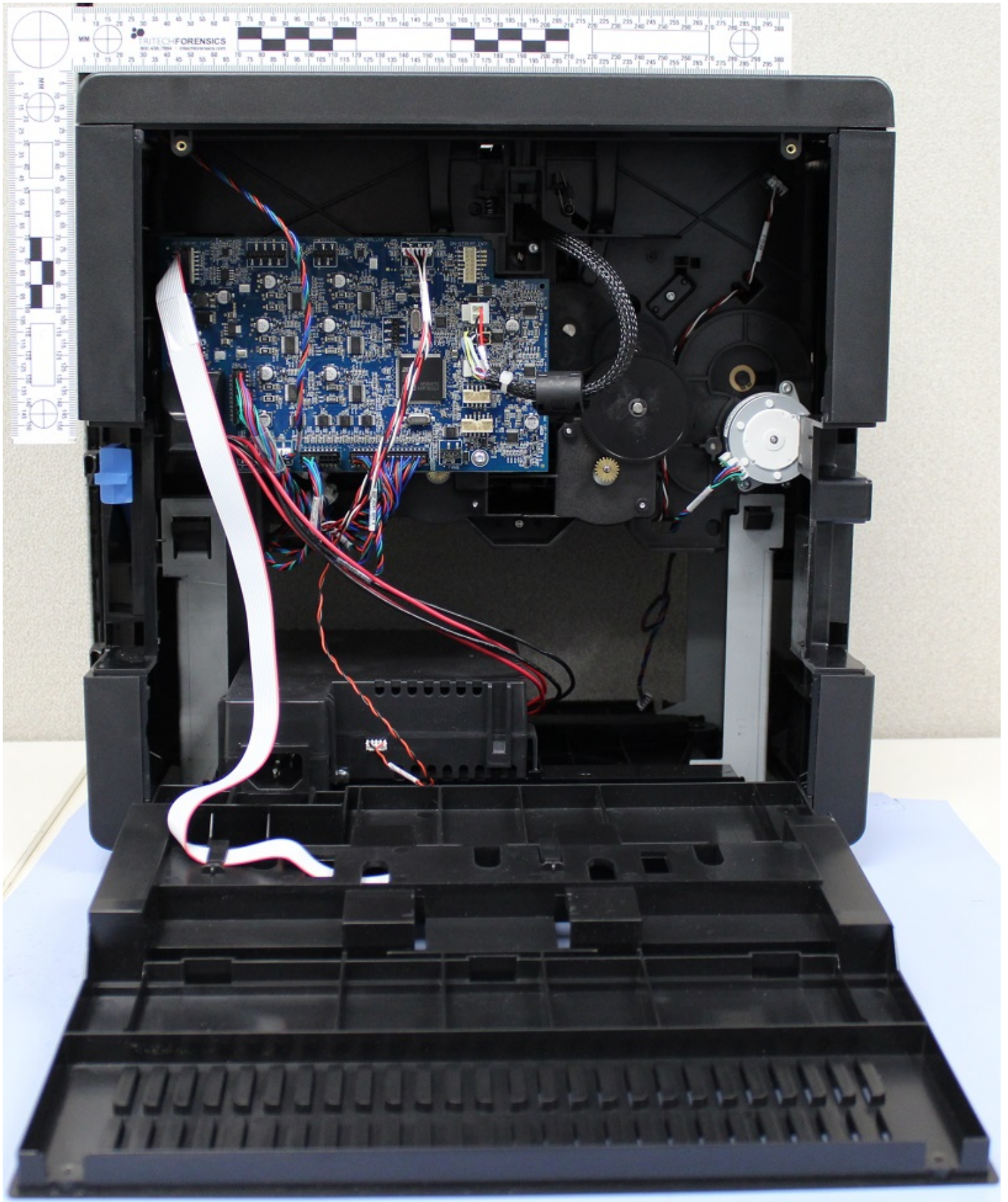
HDP6600 Laminator Accessory, back side view with door open
