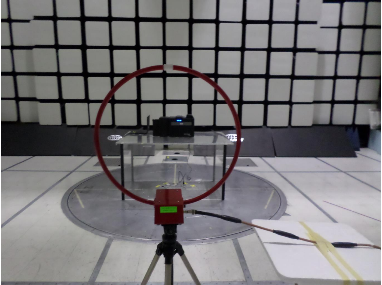
Photograph 4. 13.553-13.567 MHz Antenna View Test Setup
