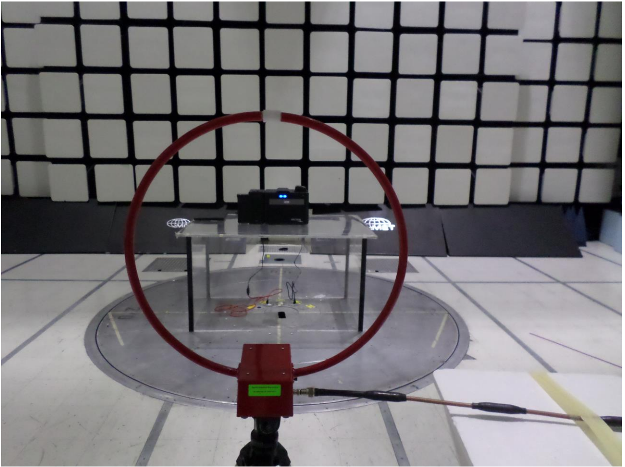
Photograph 9. RSE, Front View Test Setup (0.009 – 30 MHz)
