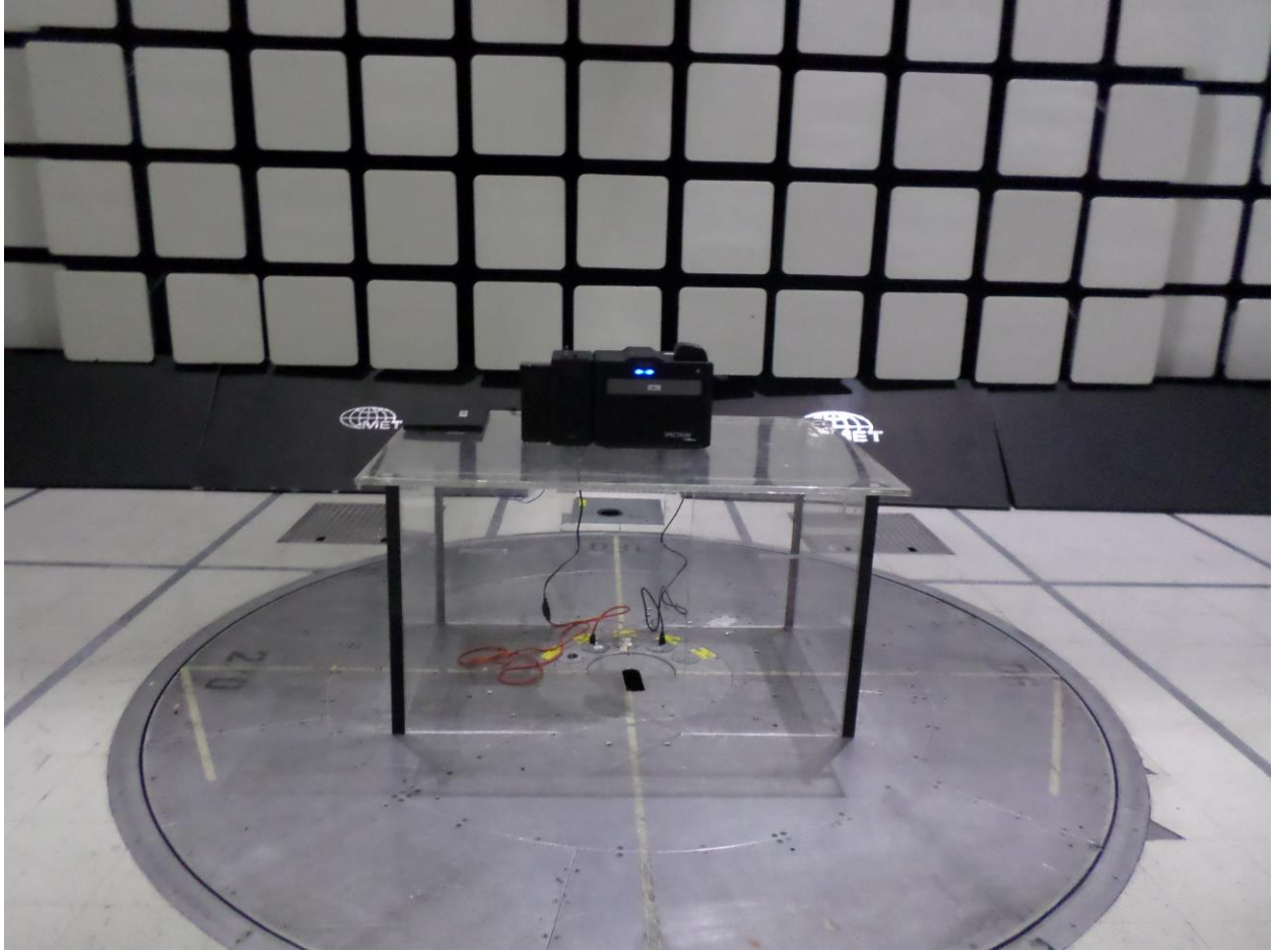
Photograph 6. 13.553-13.567 MHz Front View Test Setup
