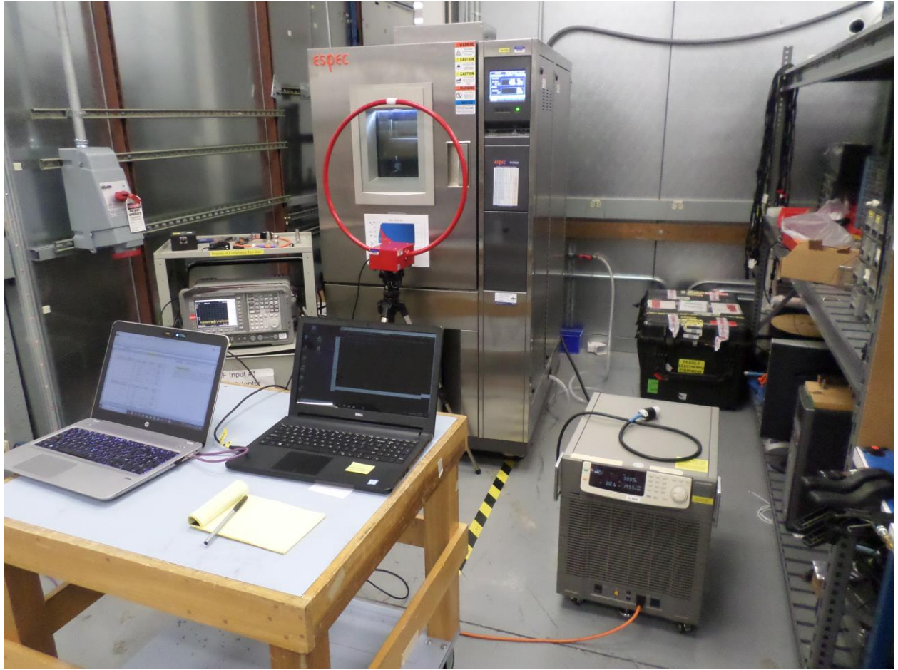
Photograph 13. FS, Right Side Test Setup
