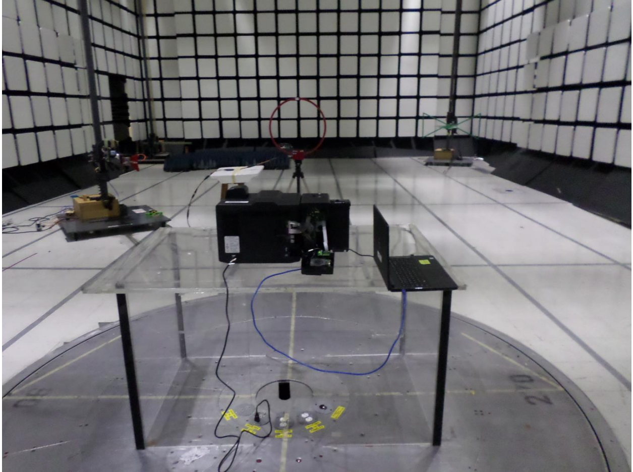
Photograph 5. 13.553-13.567 MHz Back View Test Setup
