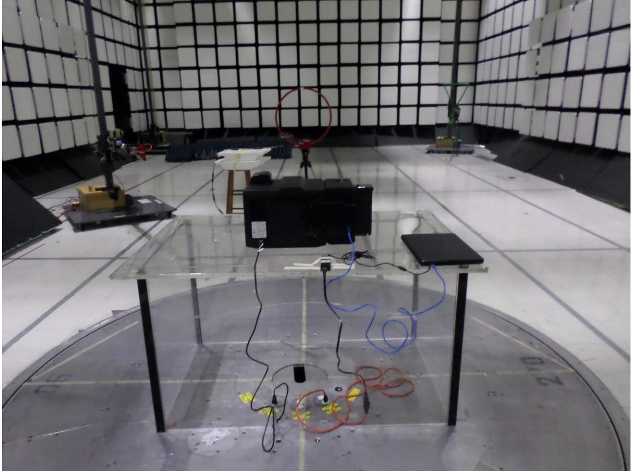
Photograph 10. RSE, Rear View Test Setup (0.009 – 30 MHz)
