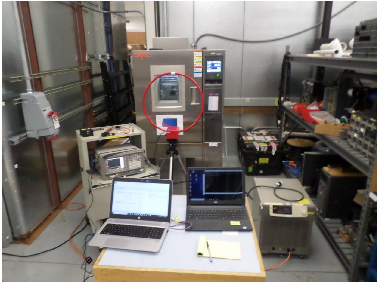
Photograph 11. FS, Front View Test Setup
