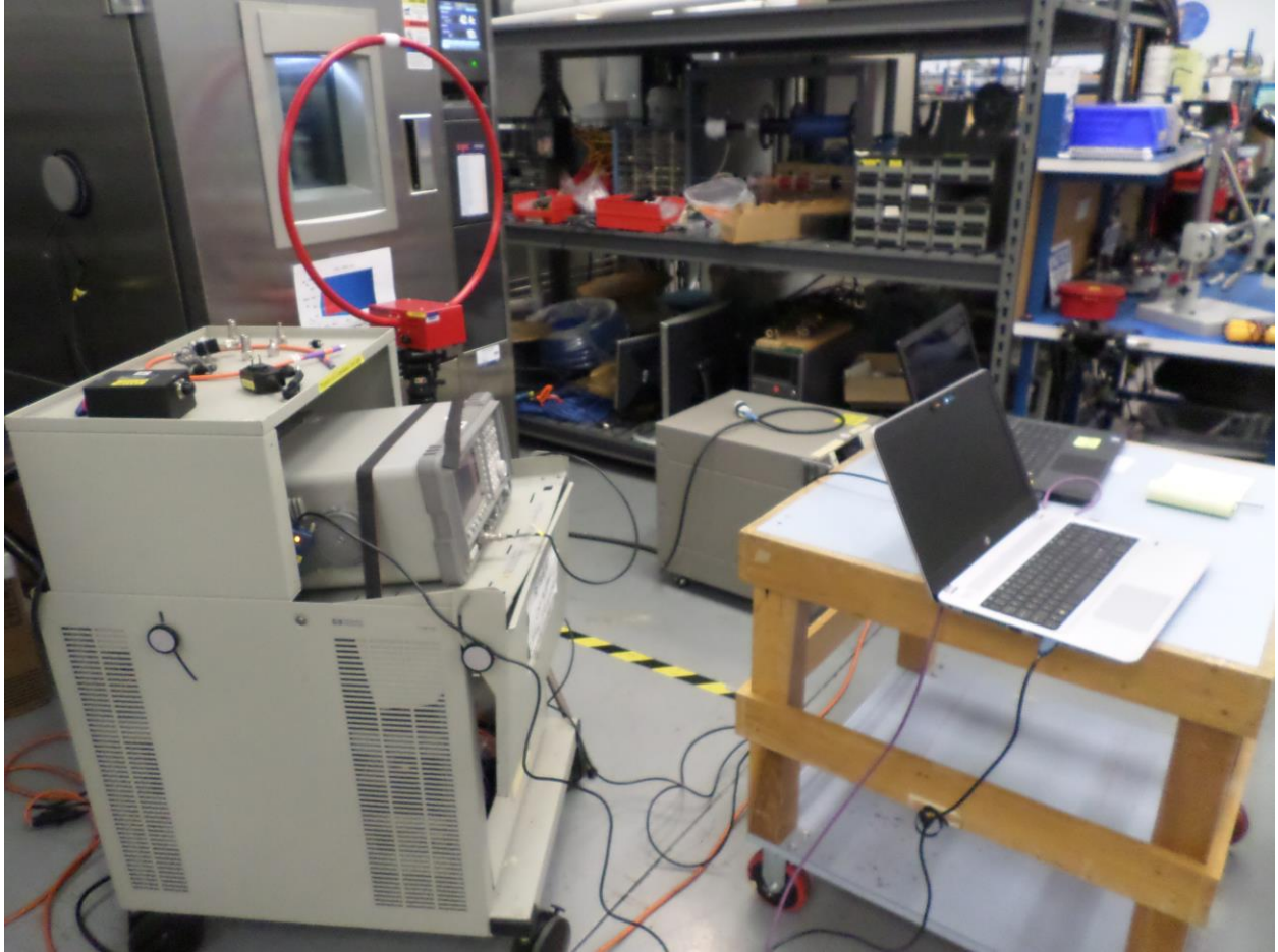
Photograph 12. FS, Left Side Test Setup
