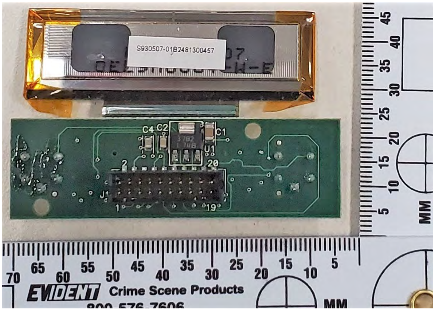
OLED Display Board Bottom Side
