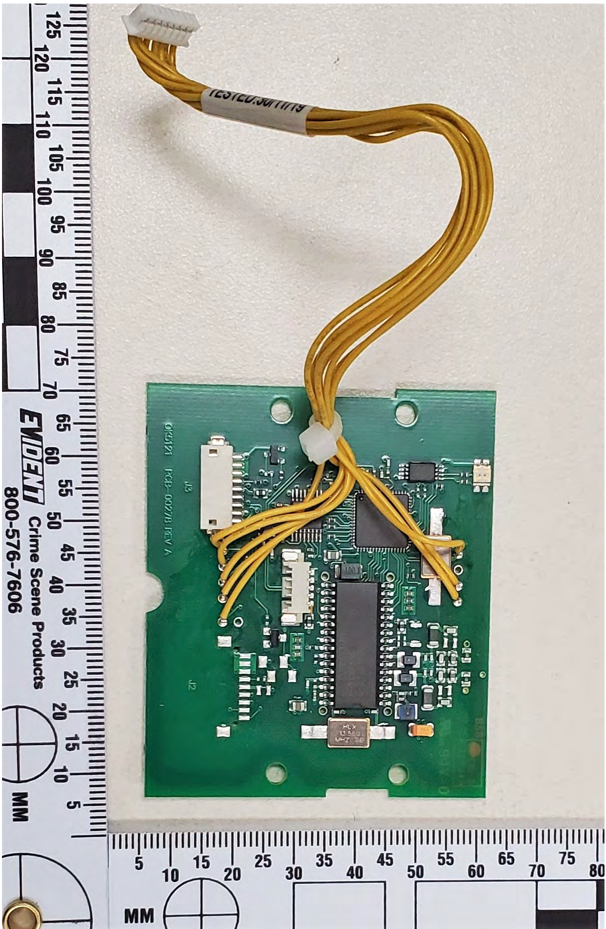
E-Card Encoder Board Top Side
