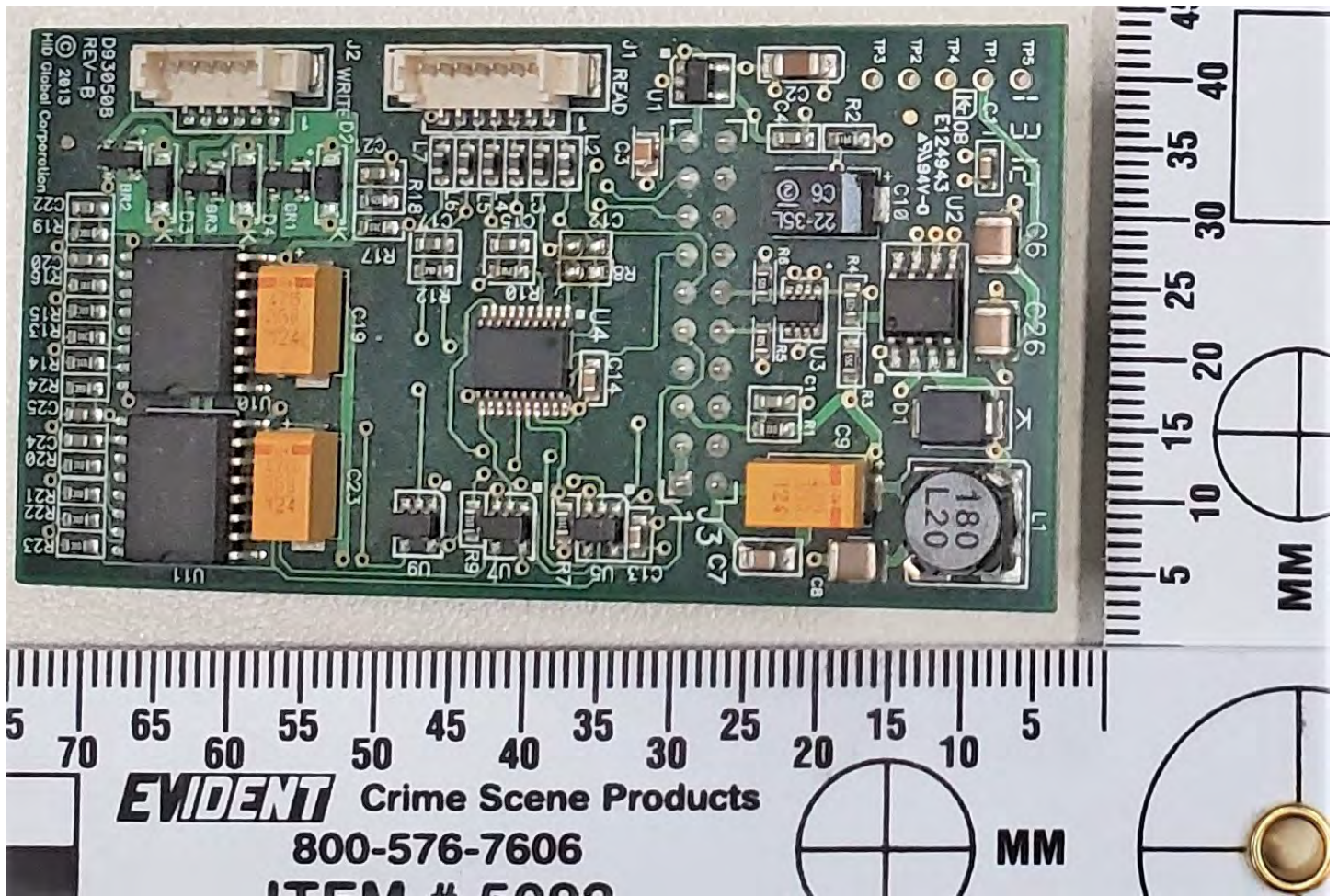
Magnetic Encoder Board Top Side
