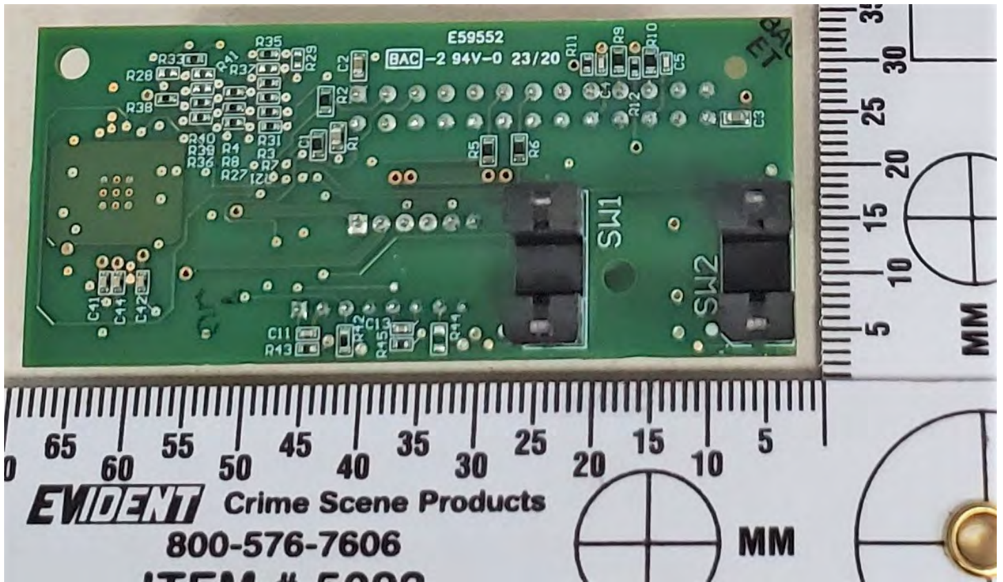
Input Hopper Controller Board Bottom Side
