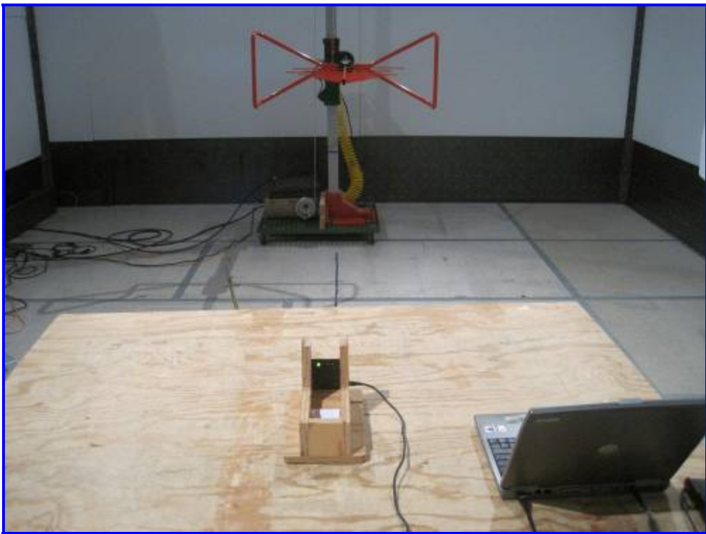
Radiated Emission, Model 3500 (>30MHz) – Rear View
