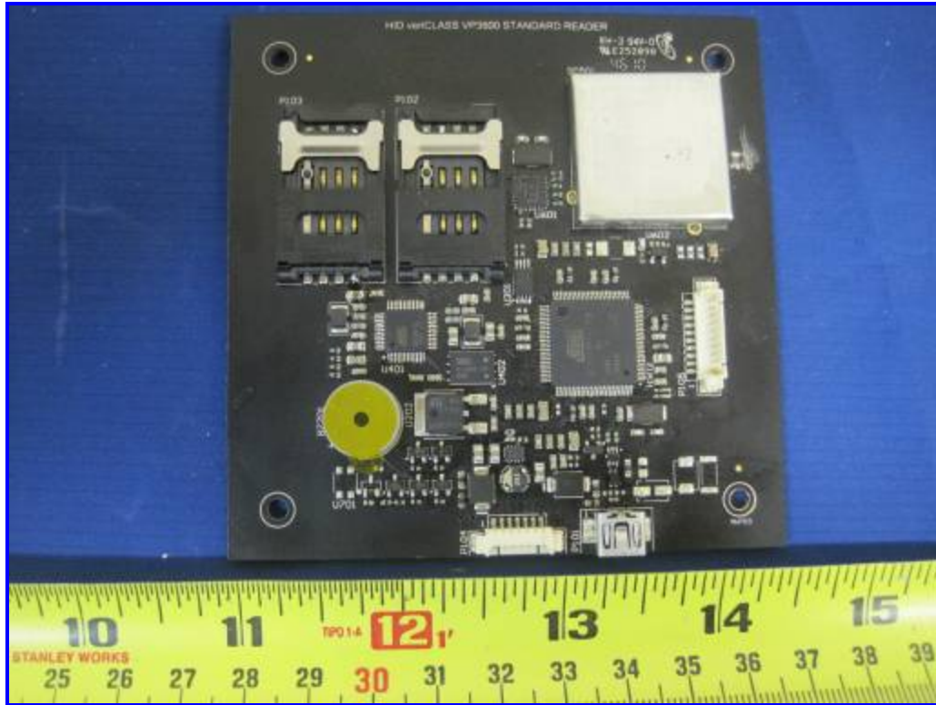
13.56MHz veriCLASS Reader Board – RF Shield ON Component View 1
