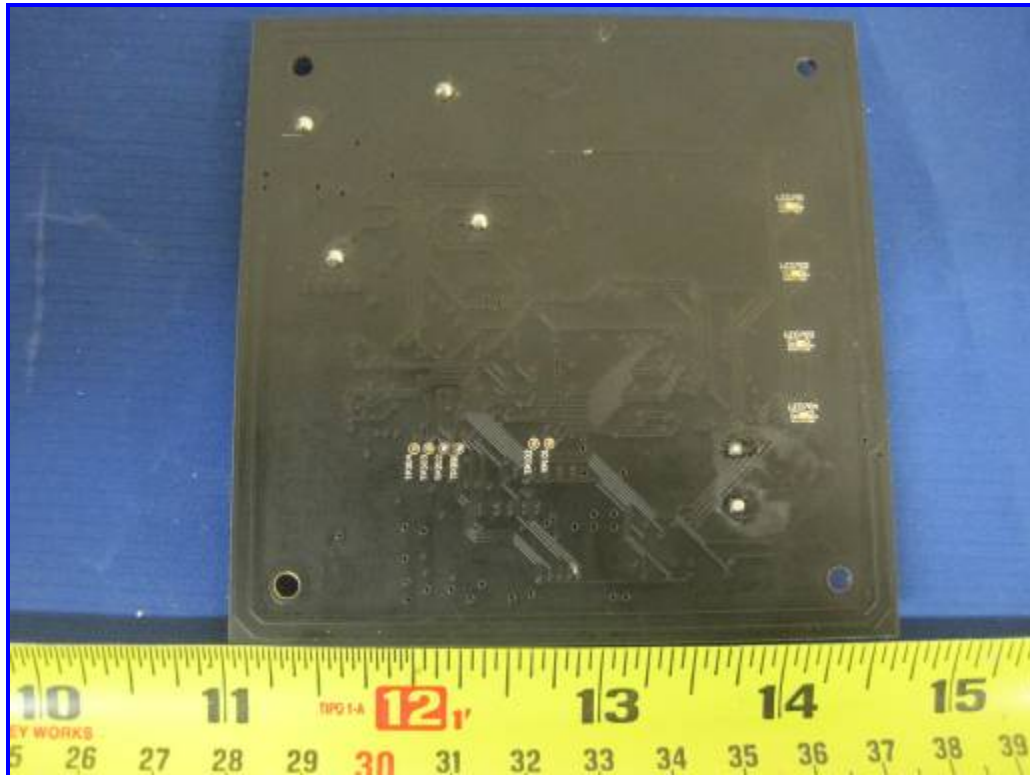
13.56MHz veriCLASS Reader Board – Solder View
