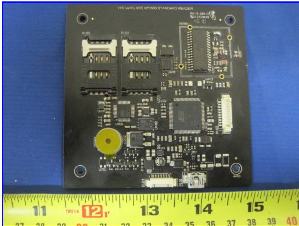
13.56MHz veriCLASS Reader Board – RF Shield OFF Component View 2
