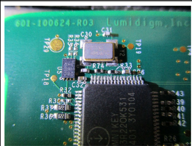
Oscillator
