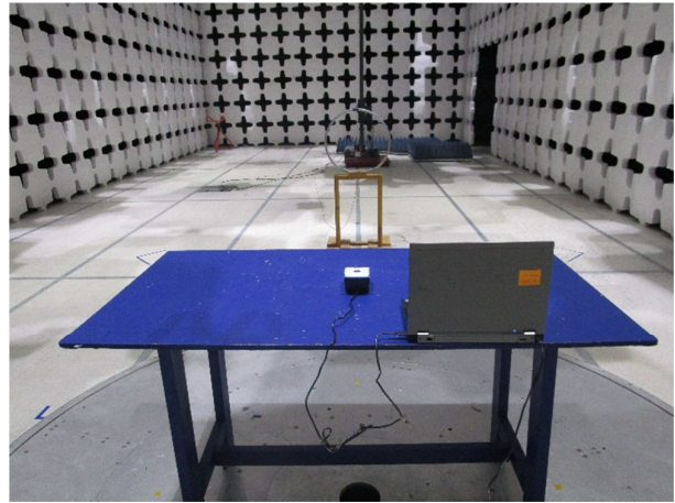
R Emission Test setup (<30MHz) – Rear View
