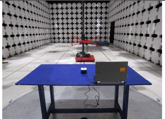
Radiated Emission Test setup (<1GHz) – Rear View
