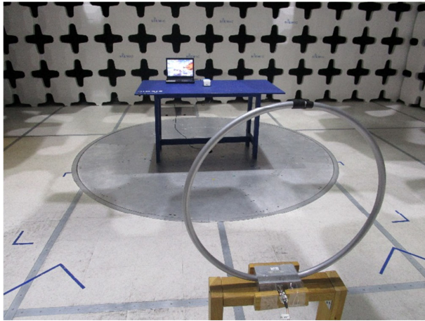
Radiation Emission Test setup (<30MHz) – Front View
