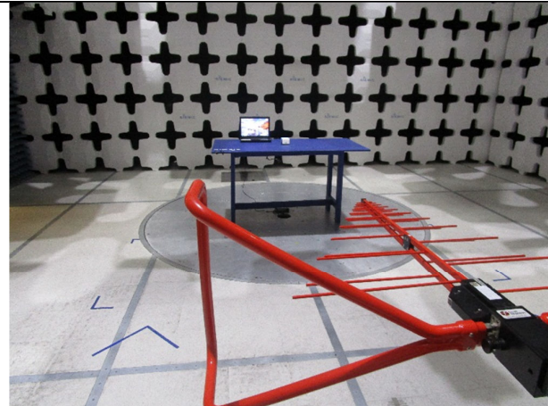
Radiated Emission Test setup (<1GHz) – Front View
