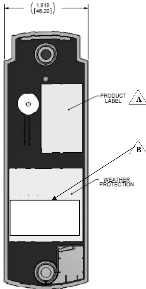
REAR VIEW
