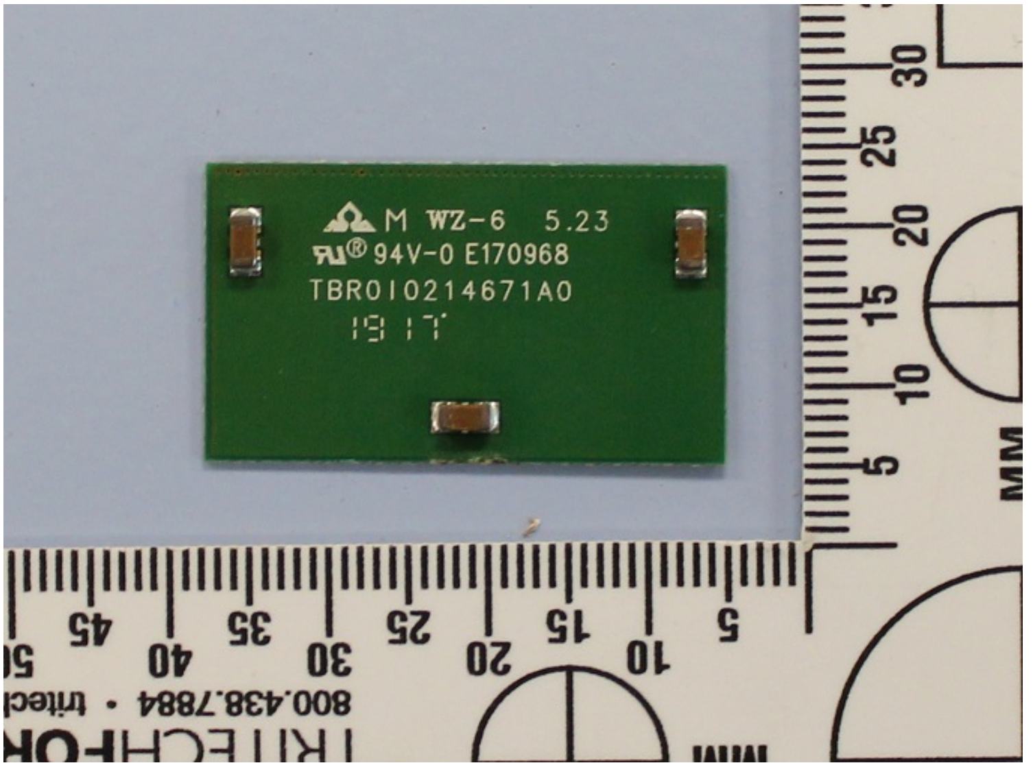
Model 40 (terminal version) patch antenna reverse
