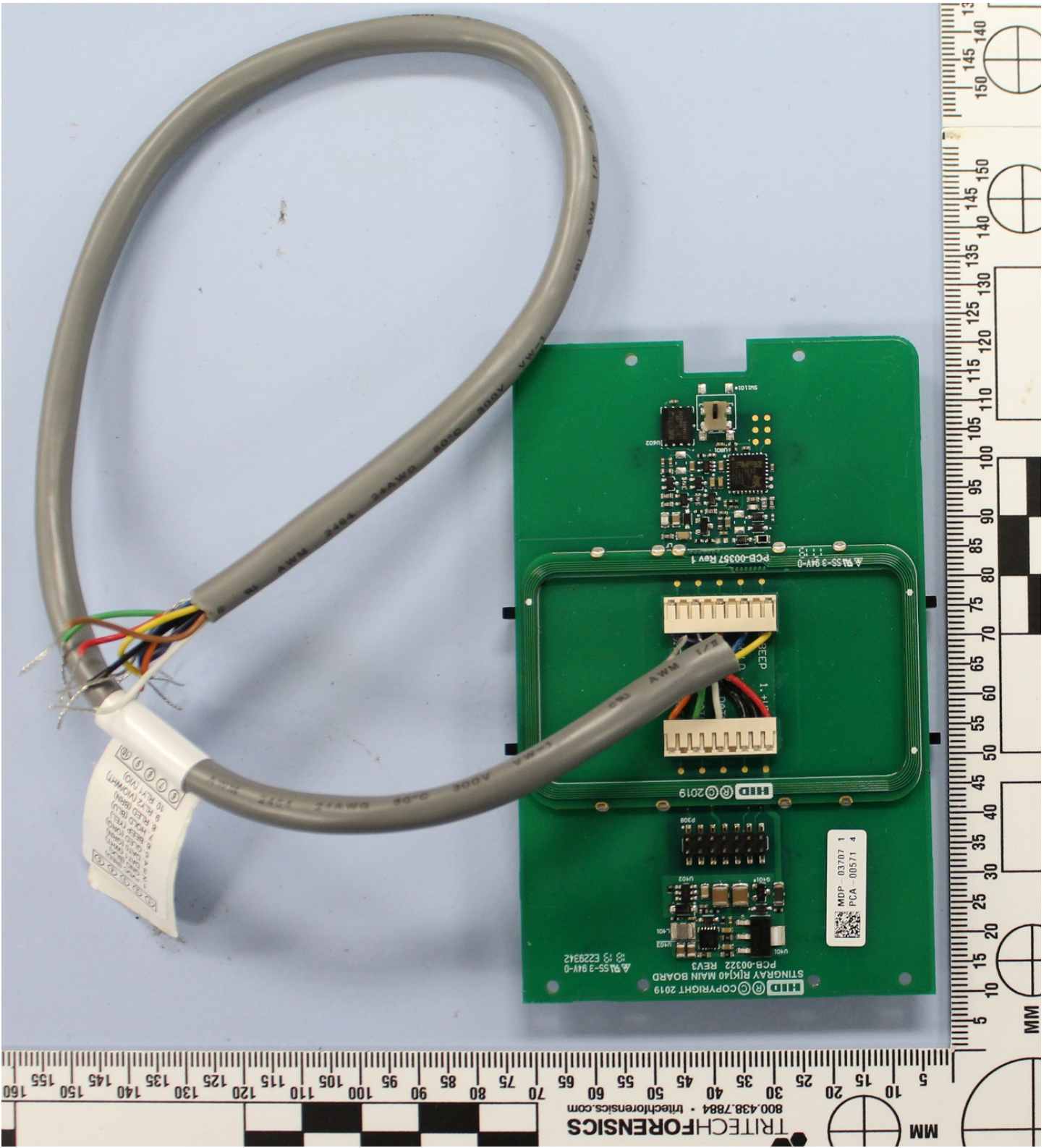
Model 40K (pigtail version) main board reverse
