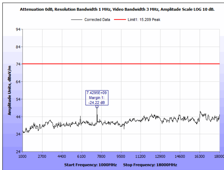
Figure 107: Radiated Spurious Emissions, Terminal, 2480 MHz, 1 GHz - 18 GHz, Peak, Vertical
