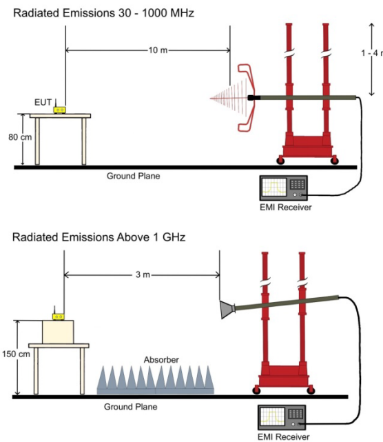
Figure 51: Radiated Emissions Test Setup
