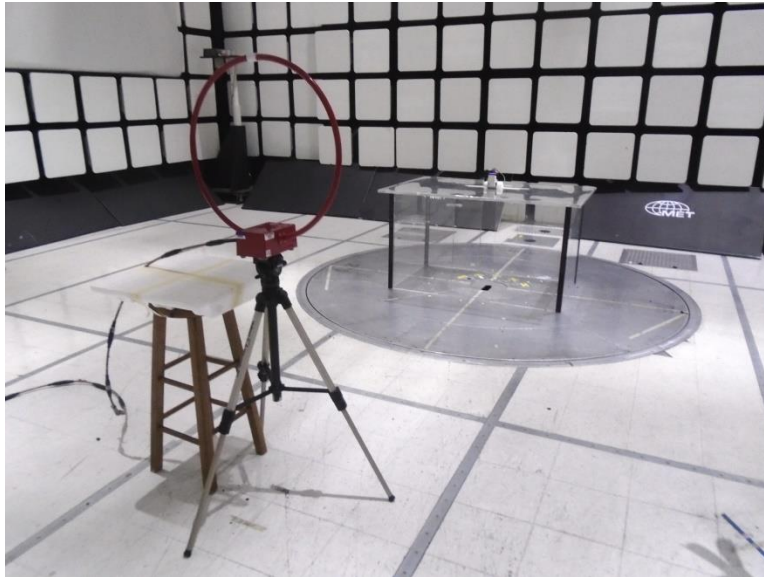
Figure 1: Radiated Spurious Emissions, Test Setup
