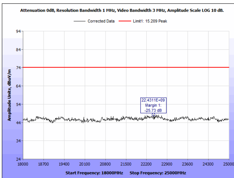
Figure 93: Radiated Spurious Emissions, Terminal, 2402 MHz, 18 GHz - 25 GHz, Peak, Horizontal
