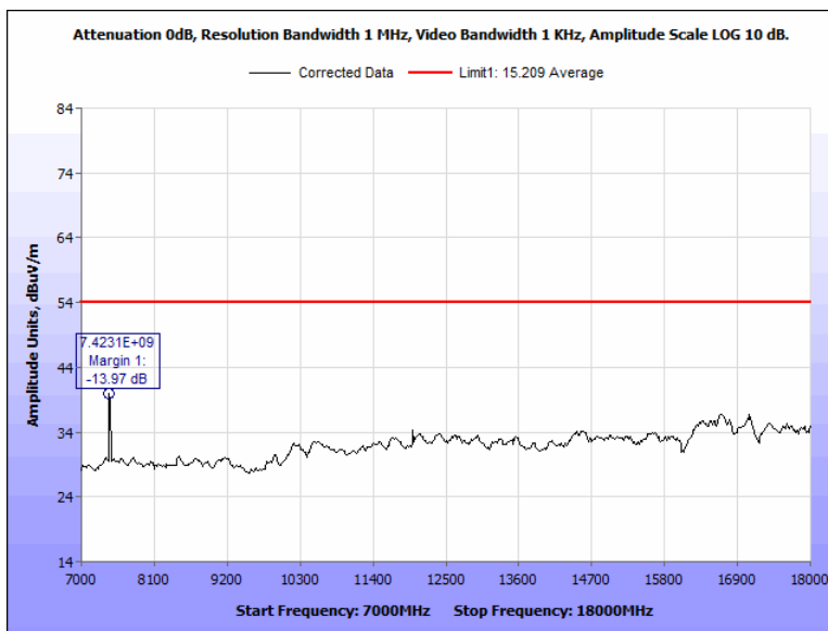
Figure 111: Radiated Spurious Emissions, Terminal, 2480 MHz, 7 GHz - 18 GHz, Average, Horizontal
