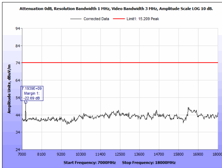
Figure 89: Radiated Spurious Emissions, Terminal, 2402 MHz, 7 GHz - 18 GHz, Peak, Horizontal
