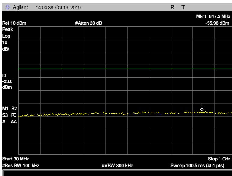
Figure 140: Conducted Spurious Emissions, Terminal, 2402 MHz, 1 Mbps, 30 MHz - 1000 MHz
