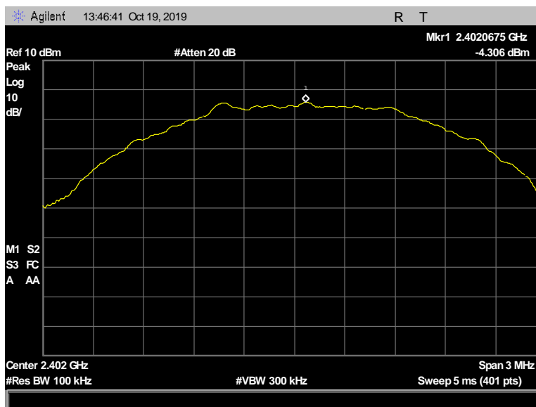
Figure 168: Peak Power Spectral Density, Terminal, 2402 MHz, 2 Mbps, -4.306 dBm
