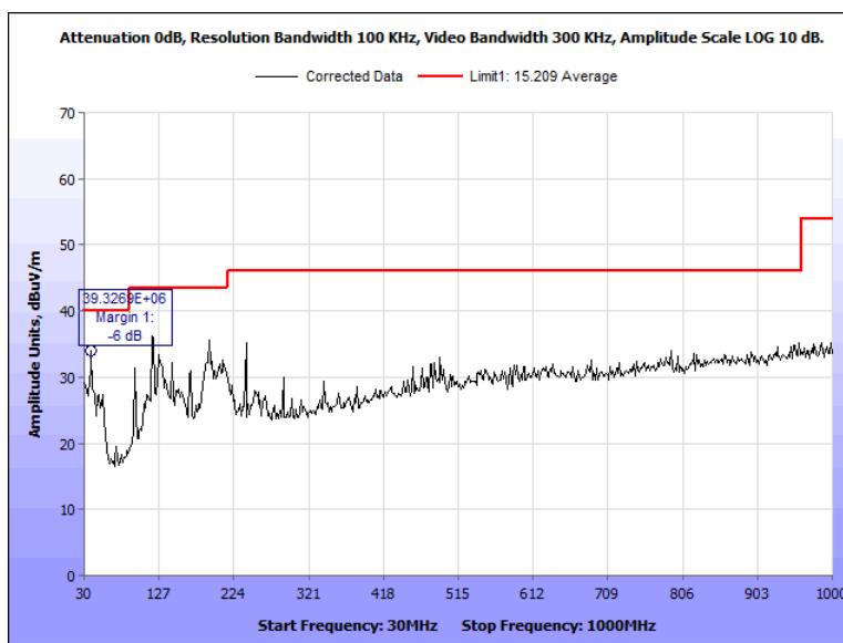
Figure 81: Radiated Spurious Emissions, Terminal, 2402 MHz, 30 MHz - 1000 MHz, Horizontal
