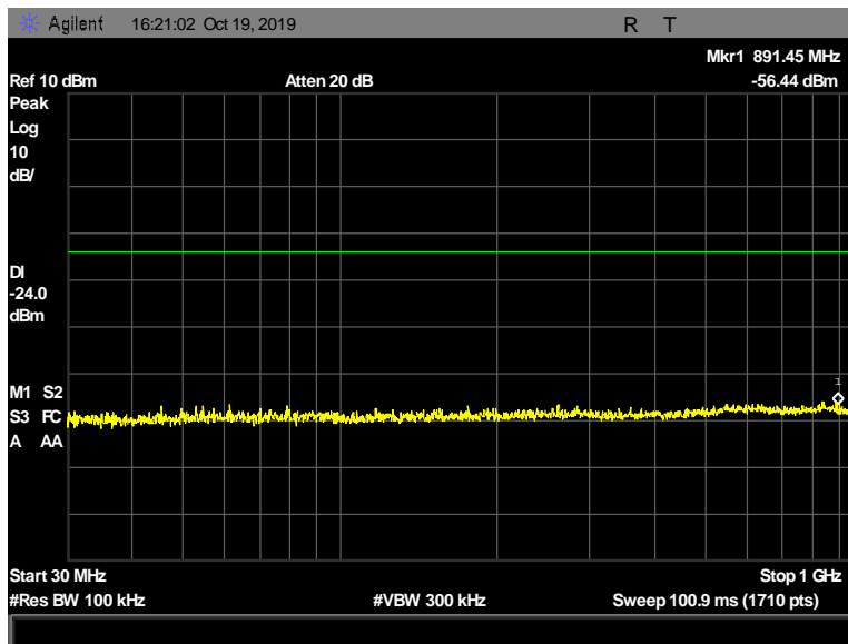
Figure 134: Conducted Spurious Emissions, Pigtail, 2480 MHz, 2 Mbps, 30 MHz - 1000 MHz
