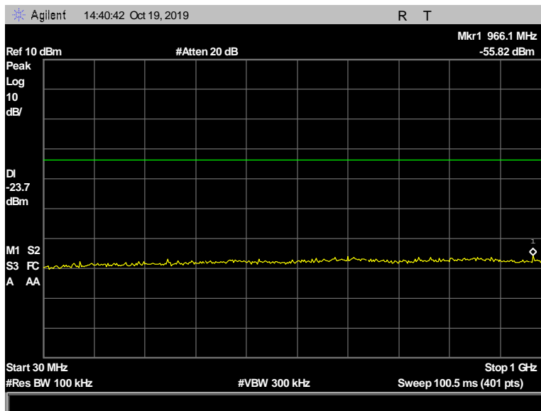
Figure 150: Conducted Spurious Emissions, Terminal, 2480 MHz, 2 Mbps, 30 MHz - 1000 MHz
