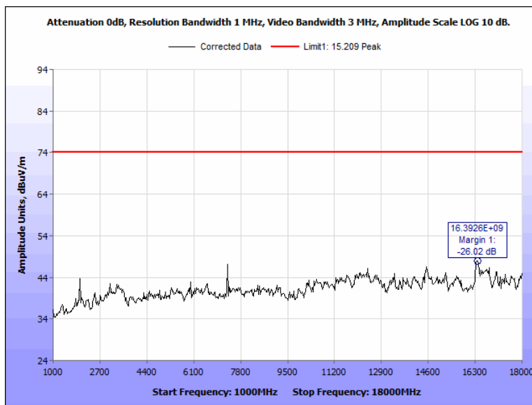
Figure 65: Radiated Spurious Emissions, Pigtail, 2442 MHz, 1 GHz - 18 GHz, Peak, Horizontal
