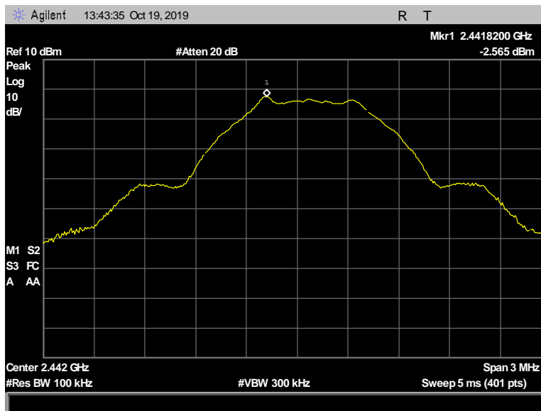
Figure 166: Peak Power Spectral Density, Terminal, 2442 MHz, 1 Mbps, -2.565 dBm
