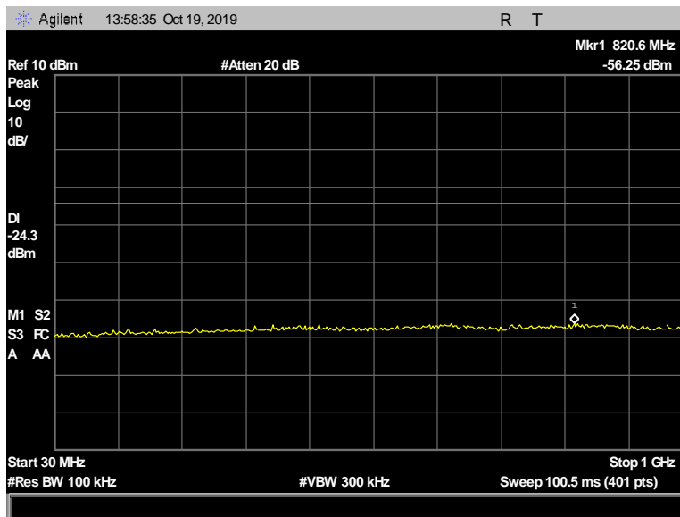
Figure 146: Conducted Spurious Emissions, Terminal, 2402 MHz, 2 Mbps, 30 MHz - 1000 MHz
