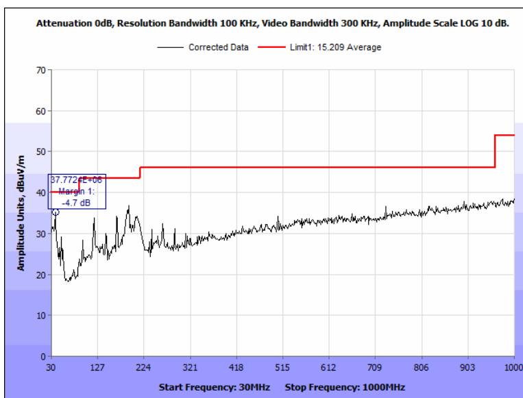
Figure 51: Radiated Spurious Emissions, Pigtail, 2402 MHz, 30 MHz - 1000 MHz, Horizontal
