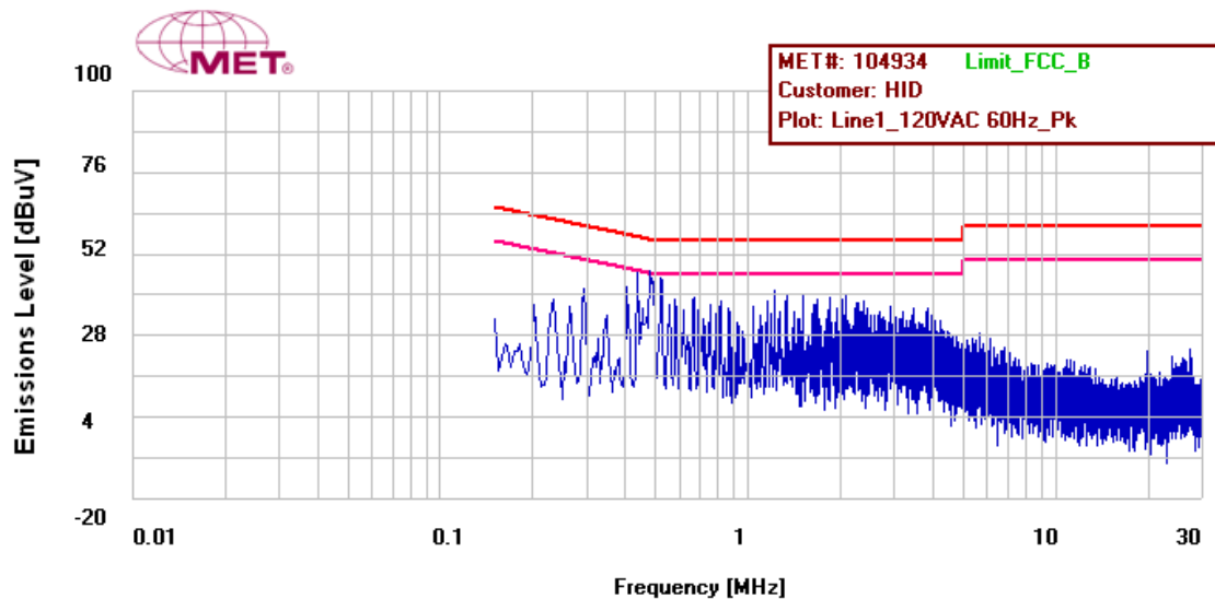
Figure 10: Conducted Emissions Limits, Pigtail, Phase Line, Prescan
