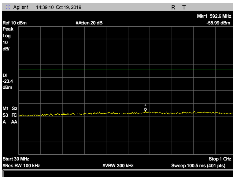
Figure 144: Conducted Spurious Emissions, Terminal, 2480 MHz, 1 Mbps, 30 MHz - 1000 MHz
