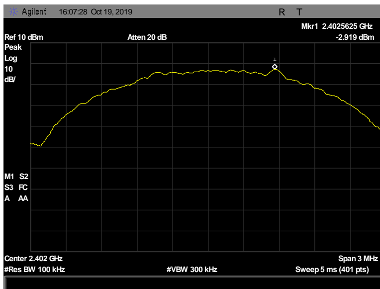
Figure 161: Peak Power Spectral Density, Pigtail, 2402 MHz, 2 Mbps, -2.919 dBm
