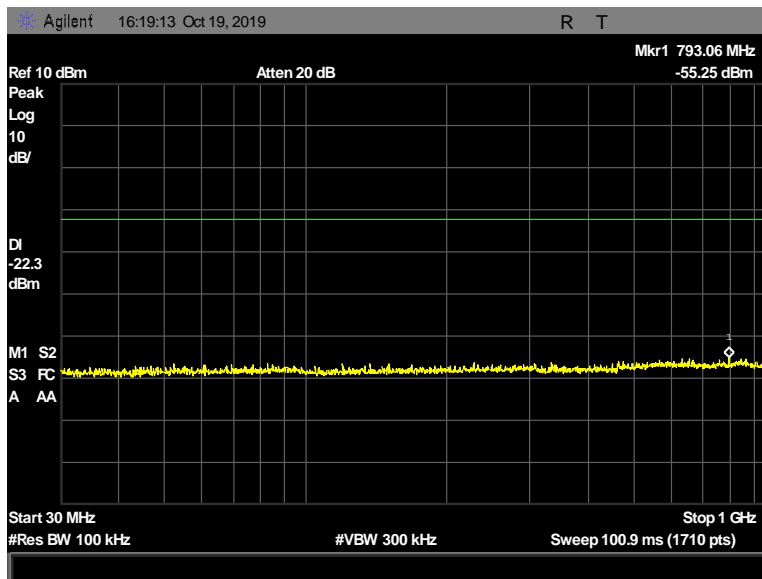
Figure 128: Conducted Spurious Emissions, Pigtail, 2480 MHz, 1 Mbps, 30 MHz - 1000 MHz
