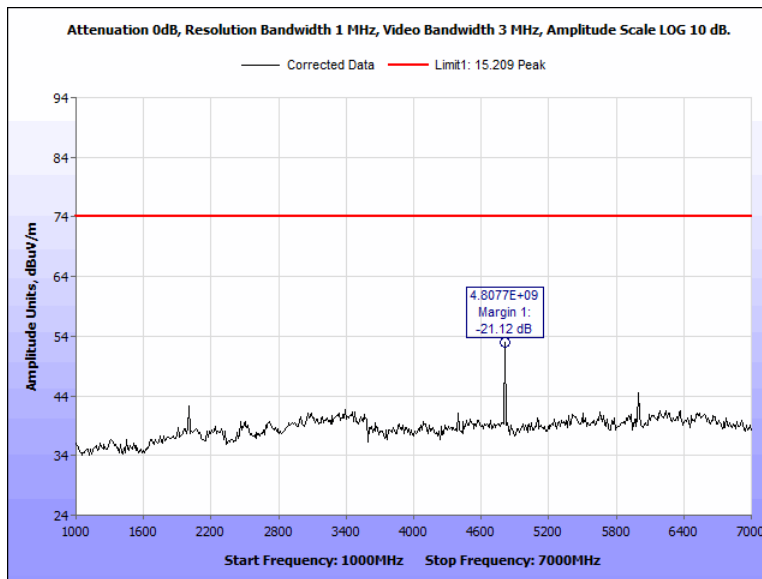
Figure 85: Radiated Spurious Emissions, Terminal, 2402 MHz, 1 GHz - 7 GHz, Peak, Horizontal
