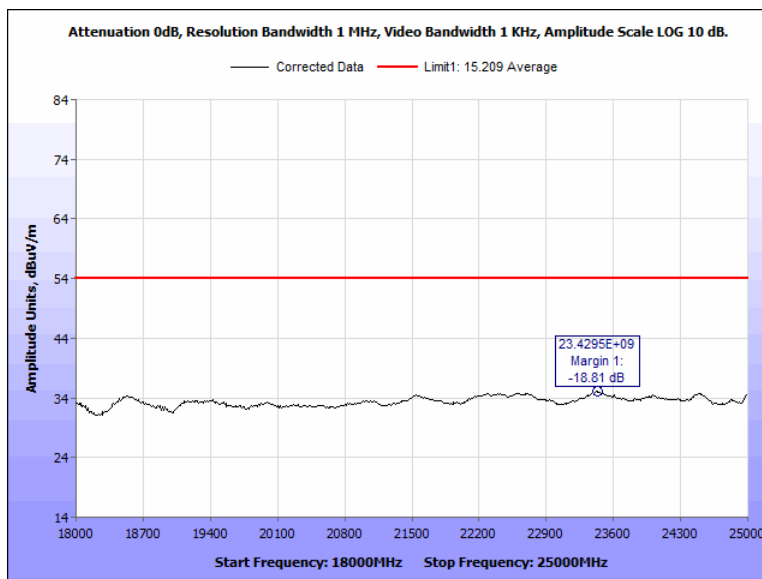
Figure 57: Radiated Spurious Emissions, Pigtail, 2402 MHz, 18 GHz - 25 GHz, Average, Vertical
