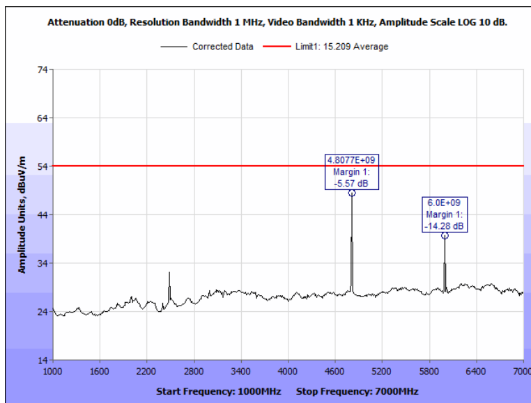
Figure 83: Radiated Spurious Emissions, Terminal, 2402 MHz, 1 GHz - 7 GHz, Average, Horizontal
