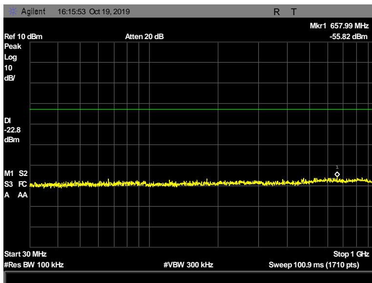
Figure 130: Conducted Spurious Emissions, Pigtail, 2402 MHz, 2 Mbps, 30 MHz - 1000 MHz
