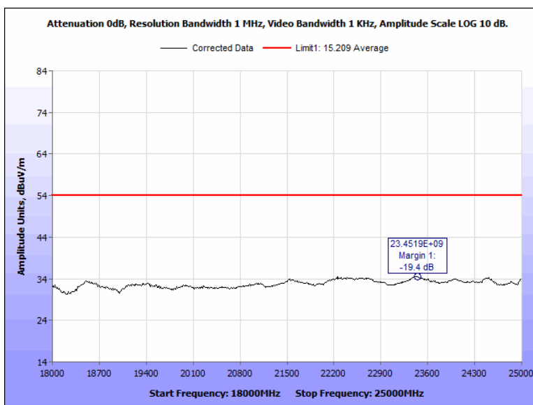
Figure 91: Radiated Spurious Emissions, Terminal, 2402 MHz, 18 GHz - 25 GHz, Average, Horizontal
