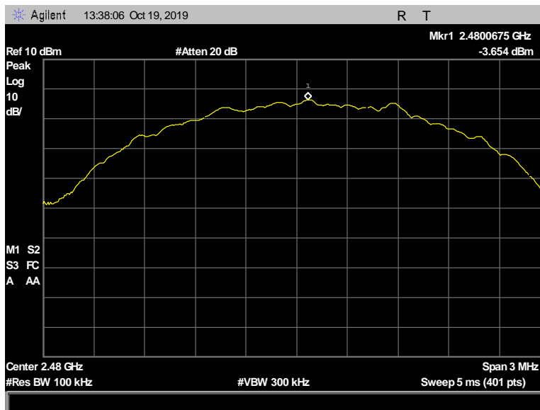
Figure 170: Peak Power Spectral Density, Terminal, 2480 MHz, 2 Mbps, -3.654 dBm
