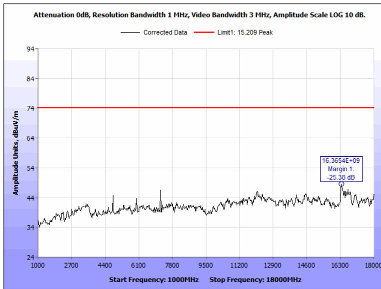
Figure 55: Radiated Spurious Emissions, Pigtail, 2402 MHz, 1 GHz - 18 GHz, Peak, Horizontal
