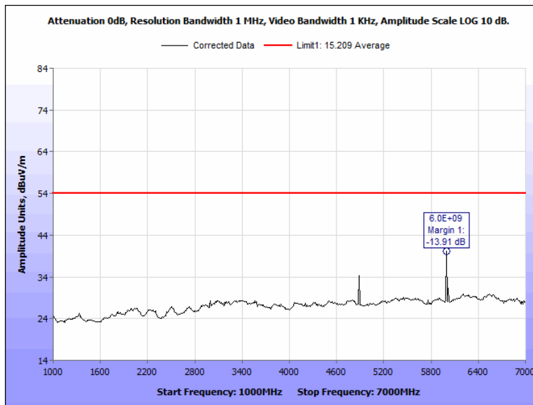
Figure 97: Radiated Spurious Emissions, Terminal, 2442 MHz, 1 GHz - 7 GHz, Average, Horizontal
