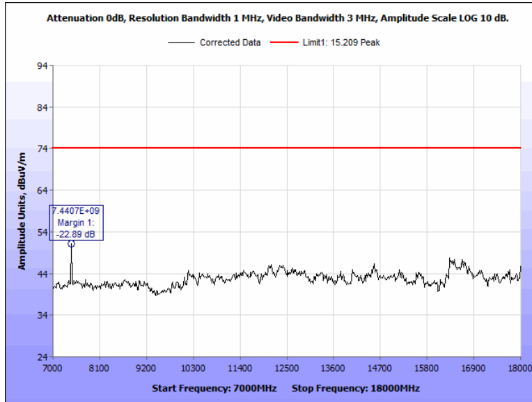
Figure 114: Radiated Spurious Emissions, Terminal, 2480 MHz, 7 GHz - 18 GHz, Peak, Vertical
