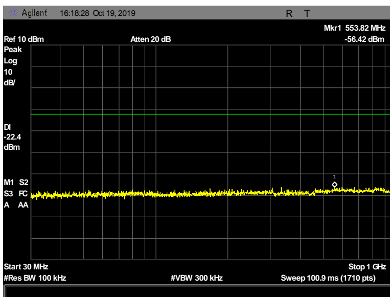
Figure 132: Conducted Spurious Emissions, Pigtail, 2442 MHz, 2 Mbps, 30 MHz - 1000 MHz
