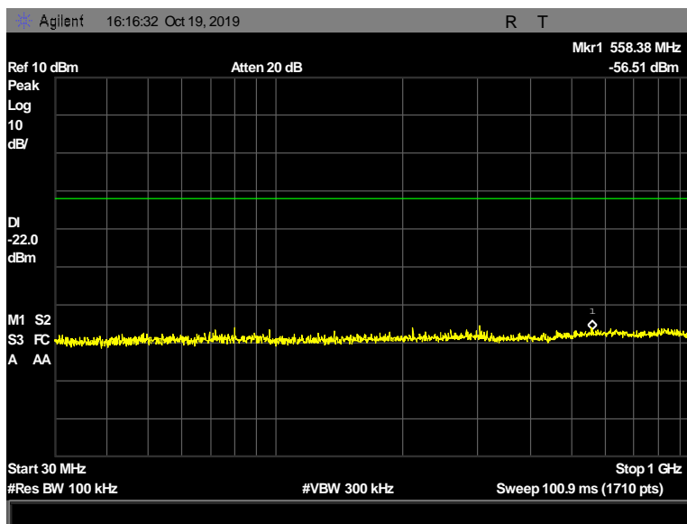
Figure 126: Conducted Spurious Emissions, Pigtail, 2442 MHz, 1 Mbps, 30 MHz - 1000 MHz
