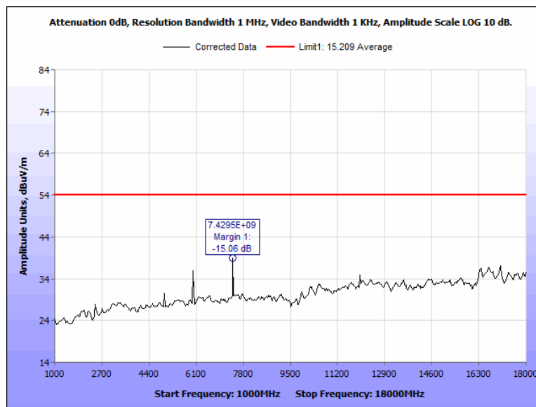
Figure 69: Radiated Spurious Emissions, Pigtail, 2480 MHz, 1 GHz - 18 GHz, Average, Horizontal
