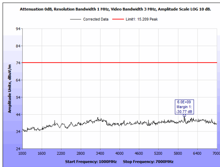
Figure 99: Radiated Spurious Emissions, Terminal, 2442 MHz, 1 GHz - 7 GHz, Peak, Horizontal
