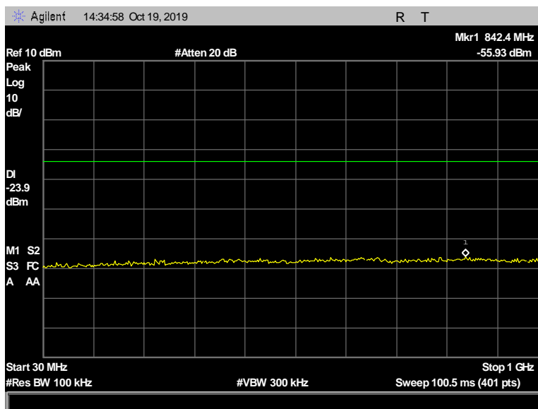
Figure 148: Conducted Spurious Emissions, Terminal, 2442 MHz, 2 Mbps, 30 MHz - 1000 MHz
