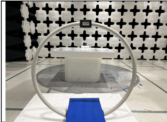
Radiated Emission Test below 30MHz Front View
