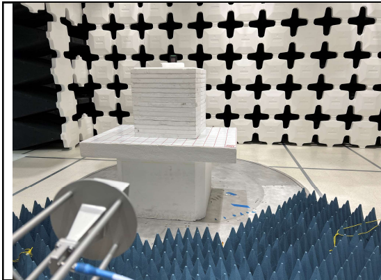
Radiated Emission Test 18-40GHz Front View
