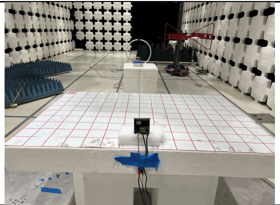
Radiated Emission Test below 30GHz Rear View
