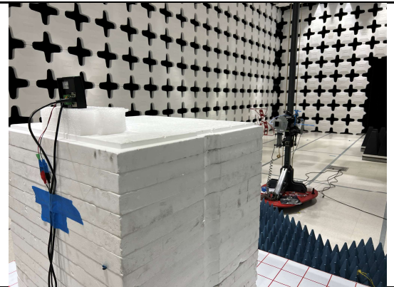
Radiated Emission Test 18-40GHz Rear View
