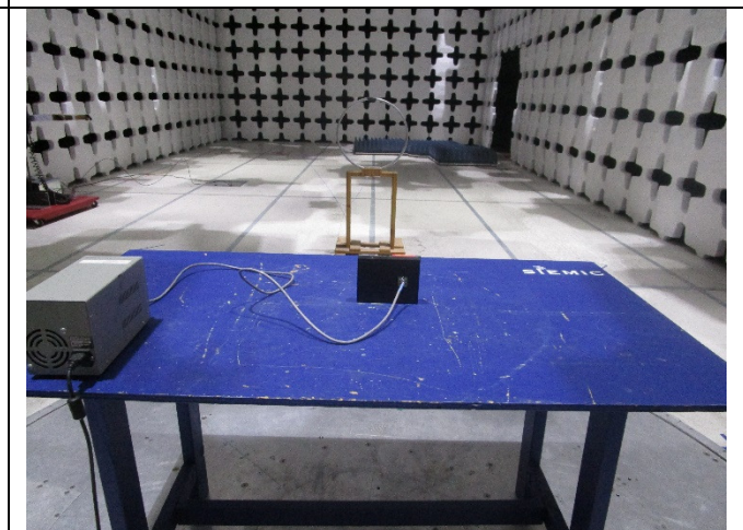
Radiated Emissions (<30MHz) – Rear View
