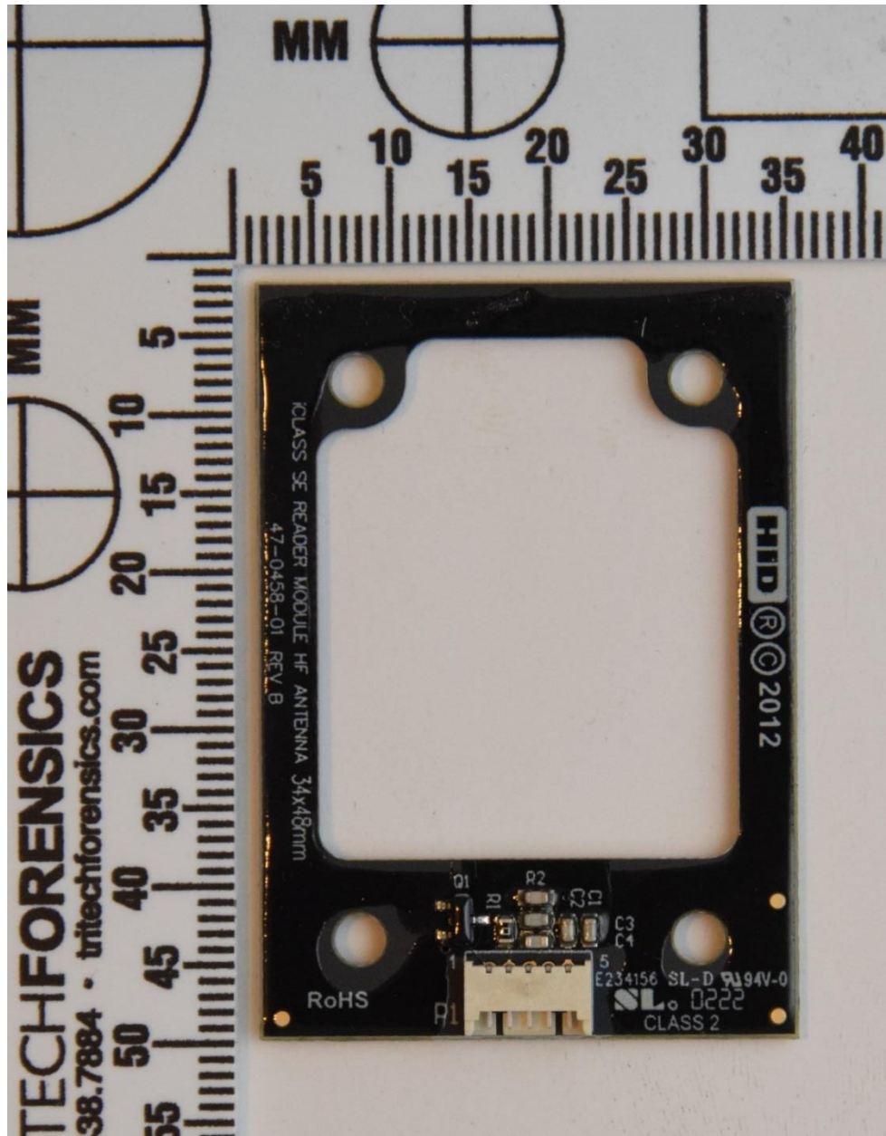
HF Antenna (Small) Front
