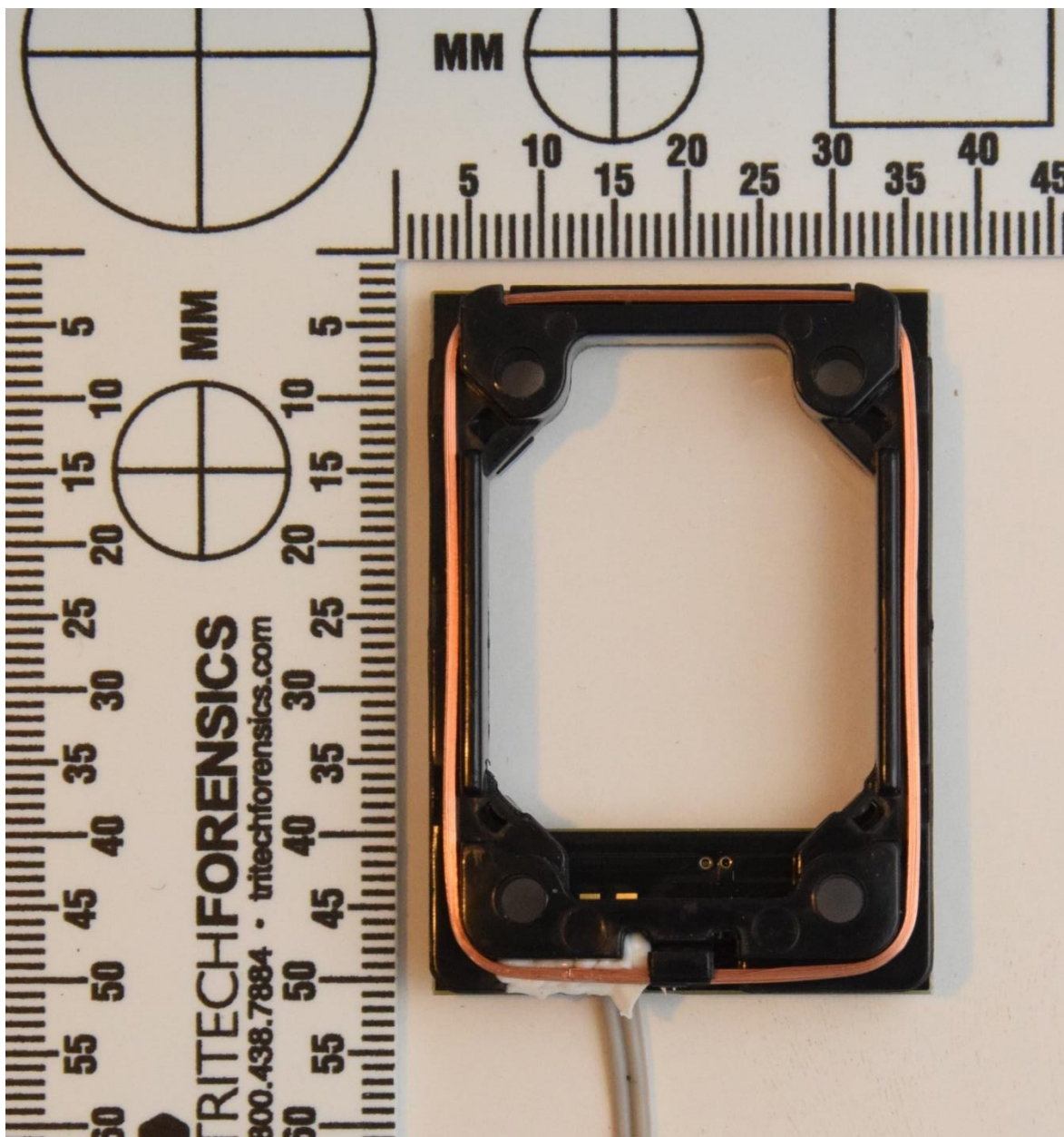
Combined LF/HF Antenna Back Side
