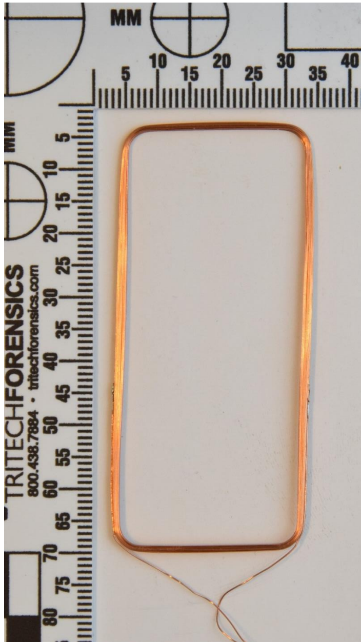
LF Antenna Coil
