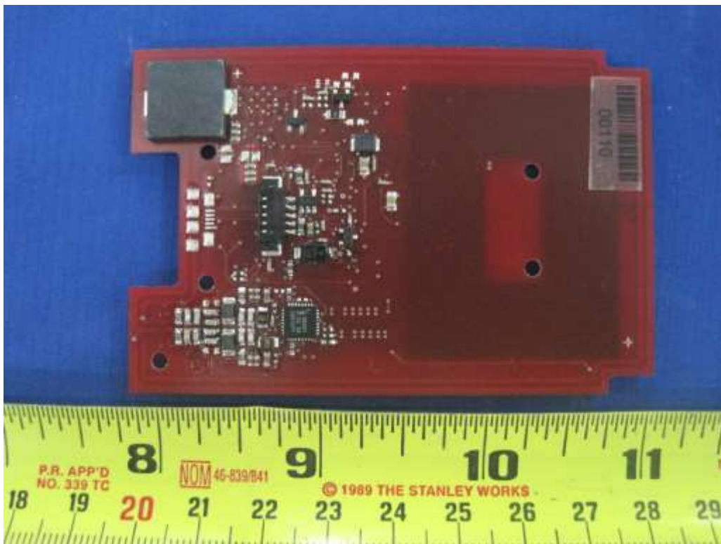
EUT radio board Bottom View
