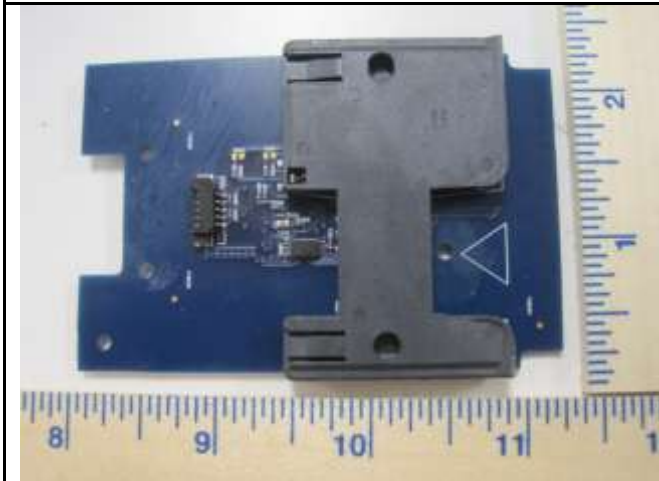
Main Board Bottom
