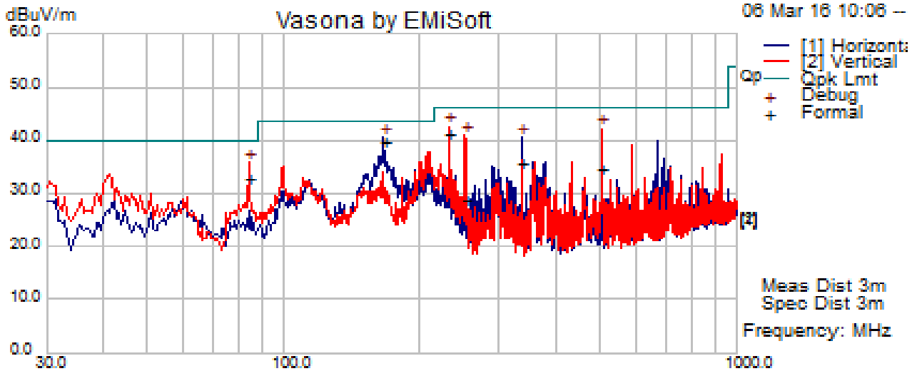
f=30\text{MHz} - 1000\text{MHz} Measurements
