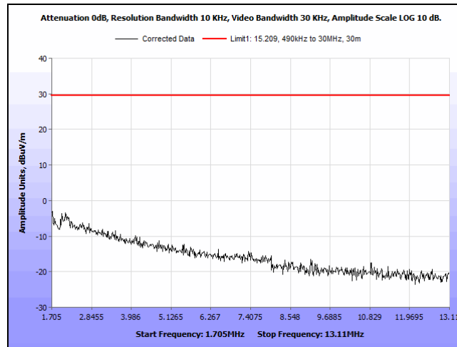
Plot 23. Spurious Emissions, Outside the Bands, 13.110 - 14. 010 MHz, 1.705MHz – 13.110MHz, 90 degrees
