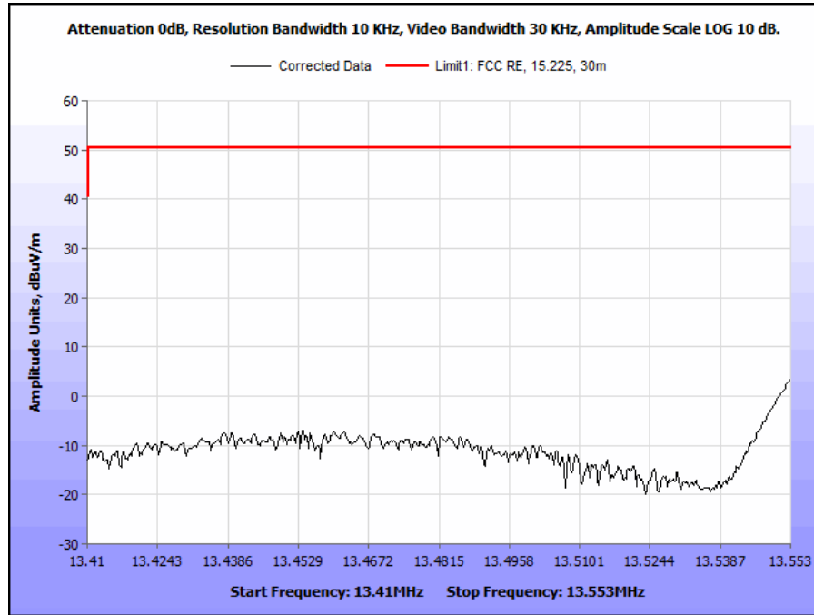
Plot 8. Operation Within the Band 13.410 – 13.553 MHz, 90 degrees
