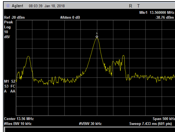
Plot 25. Frequency Stability, -15pct, -20 degrees
