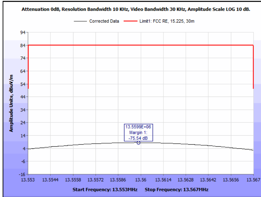
Plot 4. Operation Within the Band 13.553 – 13.567 MHz, 90 degrees
