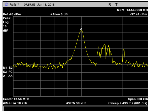
Plot 28. Frequency Stability, Vnom – -20 degree
