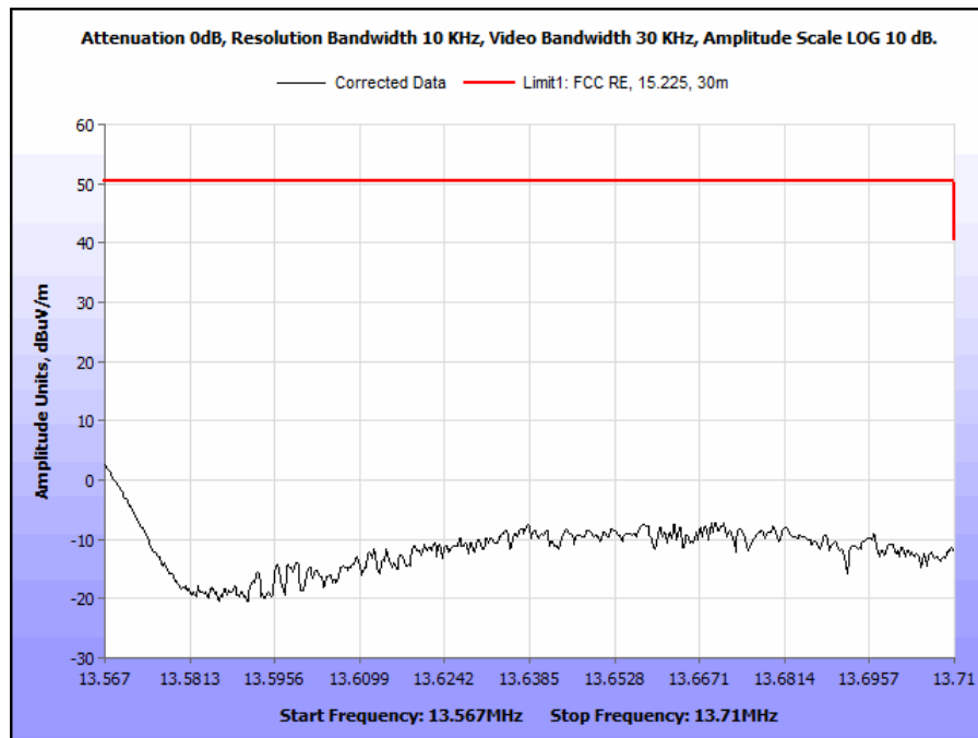
Plot 9. Operation Within the Band 13.567 – 13.710 MHz, 90 degrees
