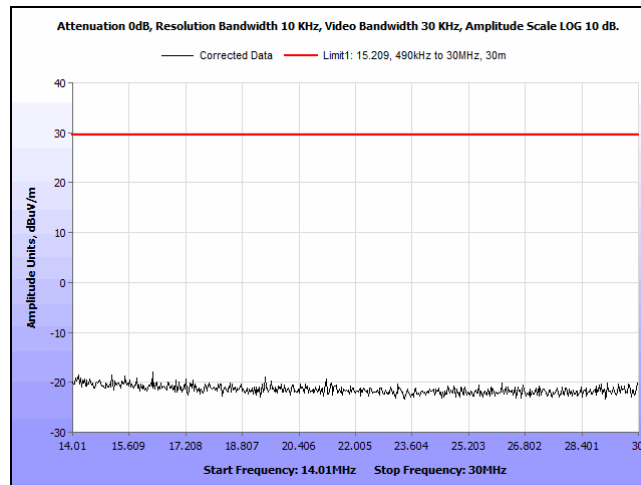
Plot 24 Spurious Emissions, Outside the Bands, 13.110 - 14. 010 MHz, 14.010MHz – 30MHz, 90 degrees
