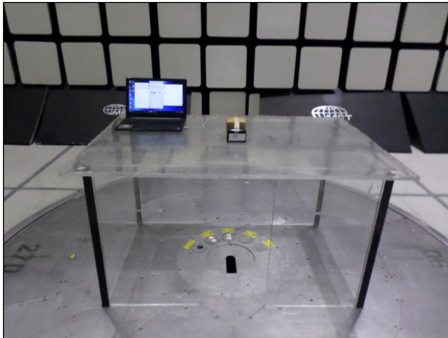
Photograph 8. Spurious Emissions, 30MHz – 135.6MHz, Front Setup
