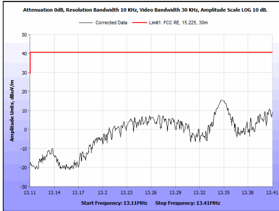
Plot 10. Operation Within the Band 13.110 – 13.410 MHz, 0 degrees
