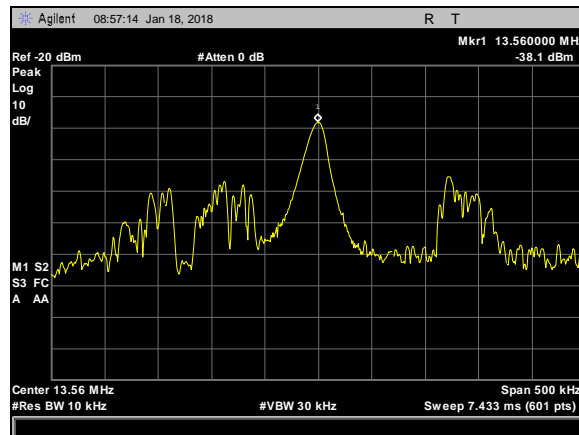
Plot 30. Frequency Stability, Vnom – 50 degree
