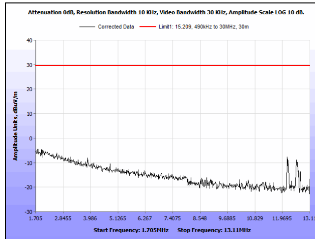
Plot 18. Spurious Emissions, Outside the Bands, 1.705MHz – 13.11MHz, 0 degrees
