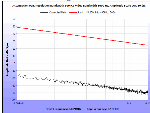
Plot 20. Spurious Emissions, Outside the Bands 13.110 - 14.010 MHz, 9KHz – 150KHz, 90 degrees
