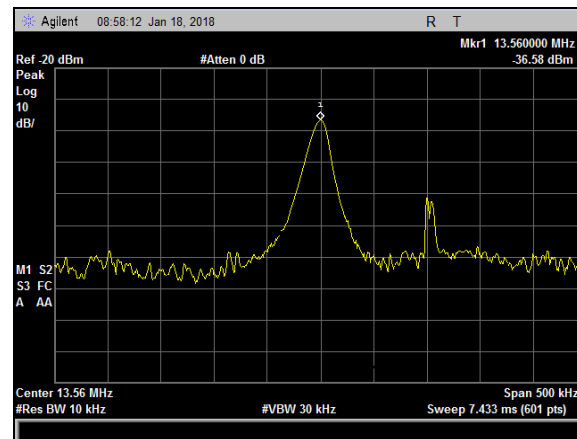
Plot 33. Frequency Stability, +15 pct, 50 degrees
