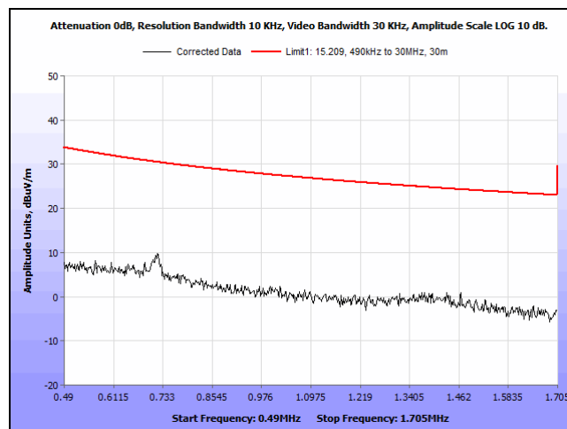
Plot 22. Spurious Emissions, Outside the Bands 13.110 - 14.010 MHz, 490KHz – 1.705MHz, 90 degrees
