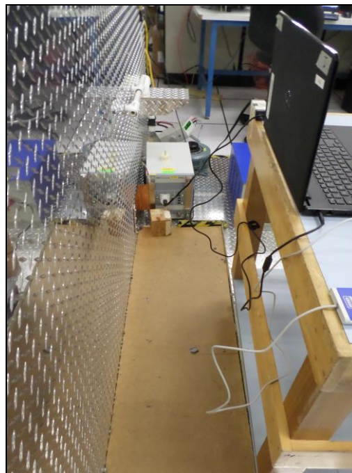
Photograph 2. Conducted Emissions, Rear LISN Connection, Test Results
