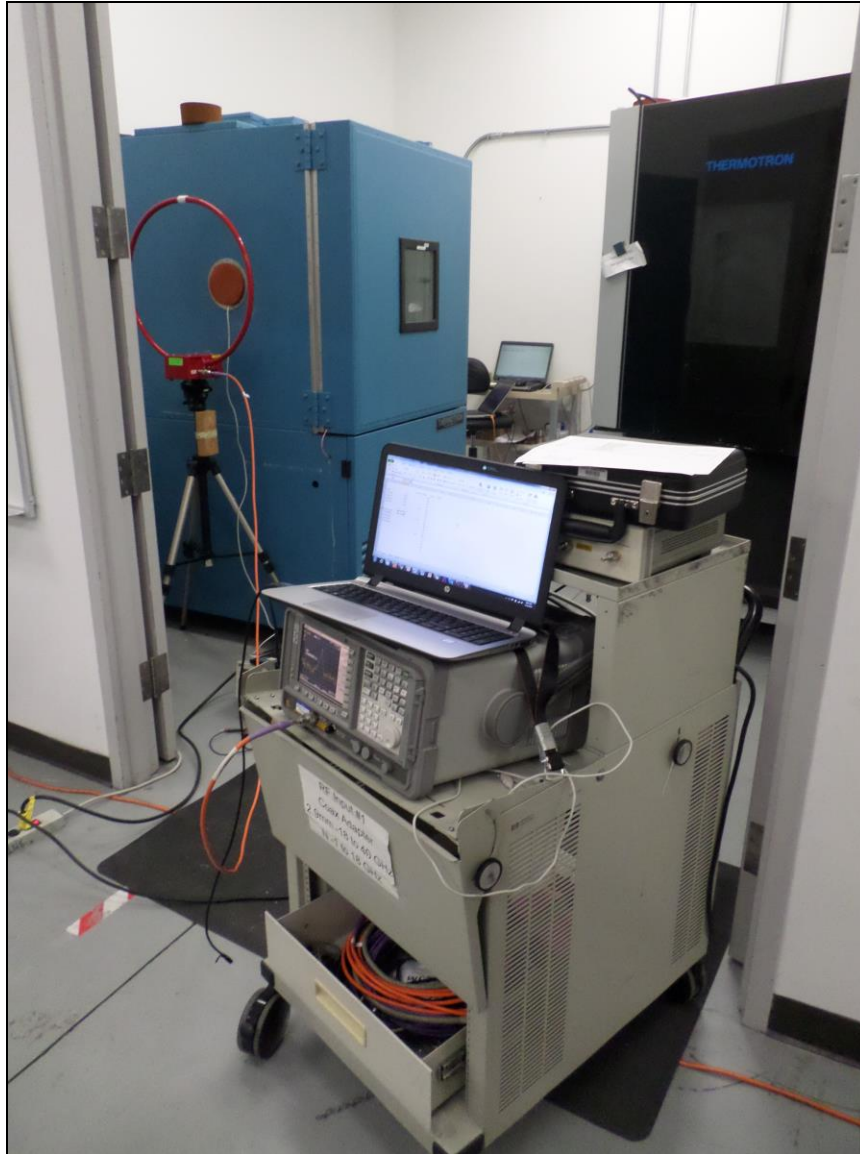
Photograph 10. Frequency Stability, Test Setup
