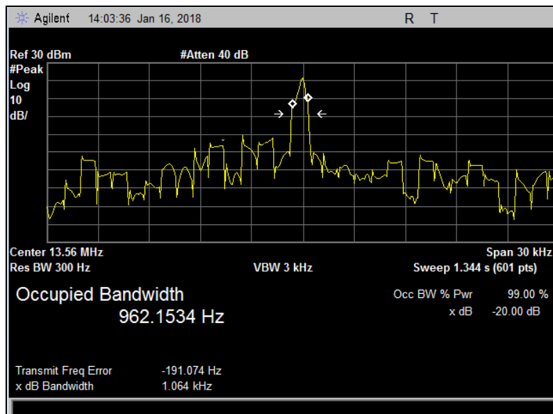
Plot 3. 20 dB and 99% Occupied Bandwidth
