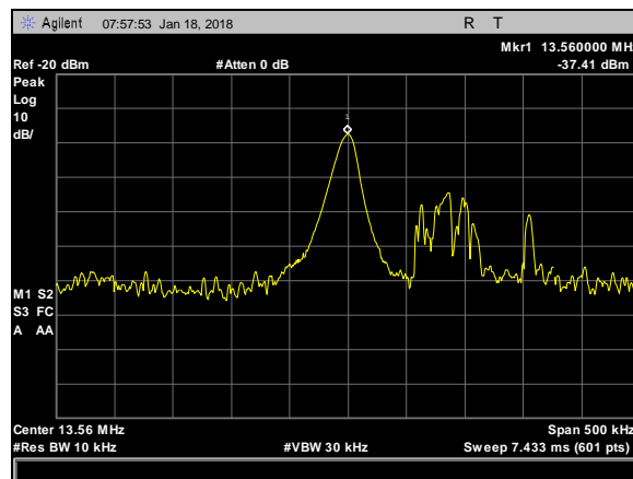
Plot 29. Frequency Stability, Vnom – 20 degree
