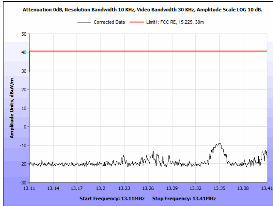
Plot 12. Operation Within the Band 13.110 – 13.410 MHz, 90 degrees
