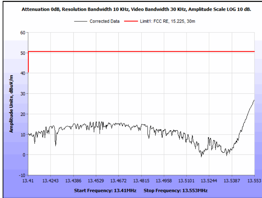
Plot 6. Operation Within the Band 13.410 – 13.553 MHz, 0 degrees
