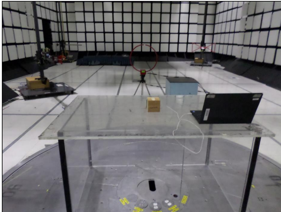
Photograph 5. Spurious Emissions, 9KHz - 30MHz, Rear Setup
