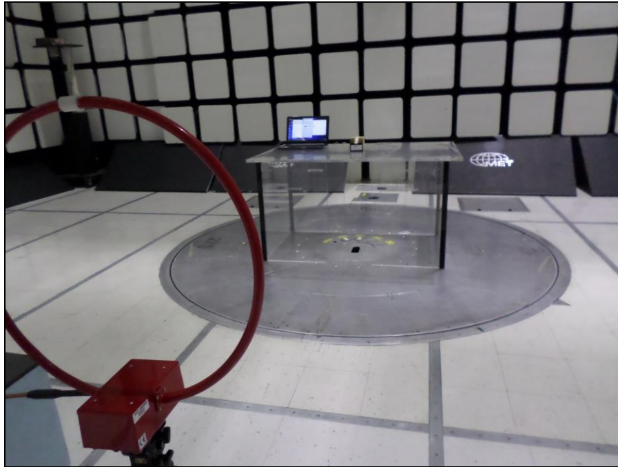
Photograph 3. Spurious Emissions, 9KHz - 30MHz, Antenna Setup
