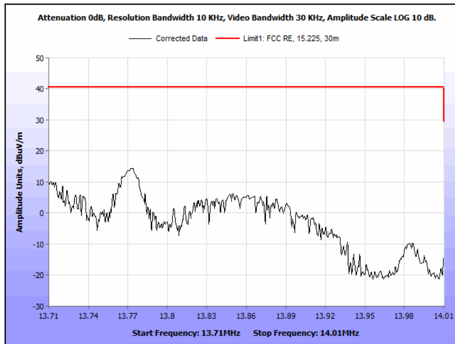
Plot 11. Operation Within the Band 13.710 – 14.010 MHz, 0 degrees
