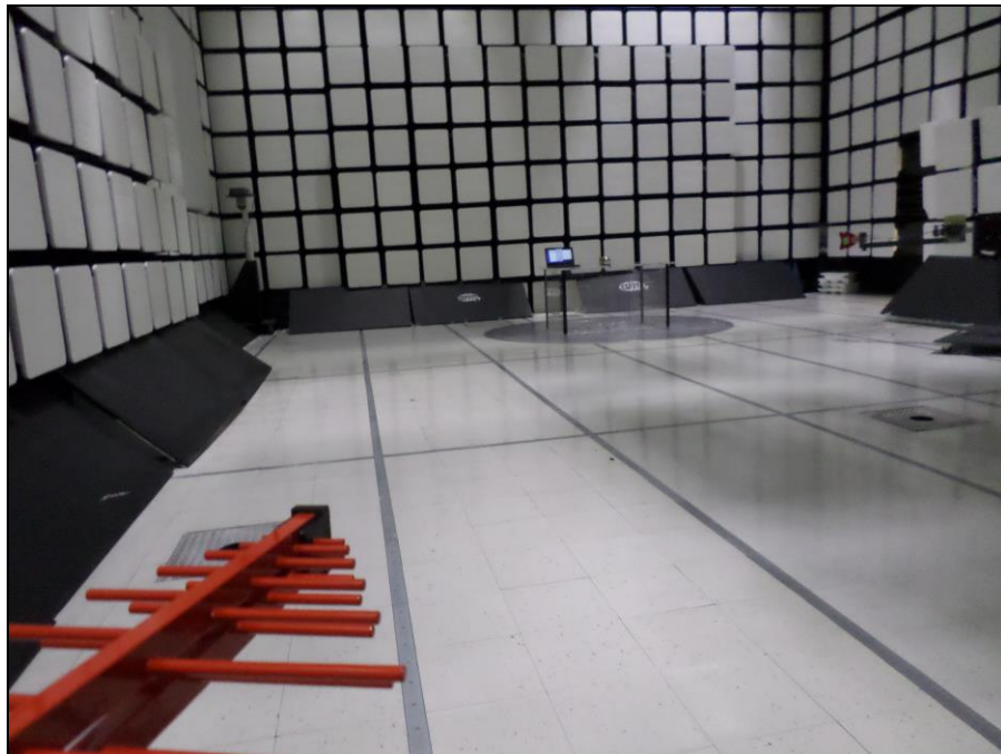
Photograph 6. Spurious Emissions, 30MHz - 135.6MHz, Antenna Setup
