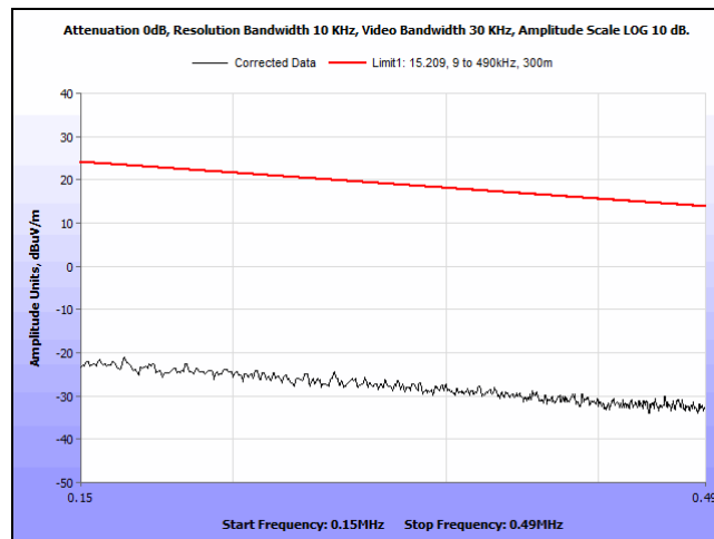
Plot 21. Spurious Emissions, Outside the Bands 13.110 - 14.010 MHz, 150KHz – 490KHz, 90 degrees
