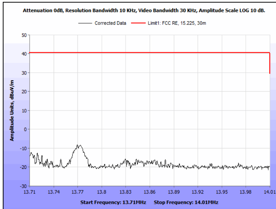
Plot 13. Operation Within the Band 13.710 – 14.010 MHz, 90 degrees
