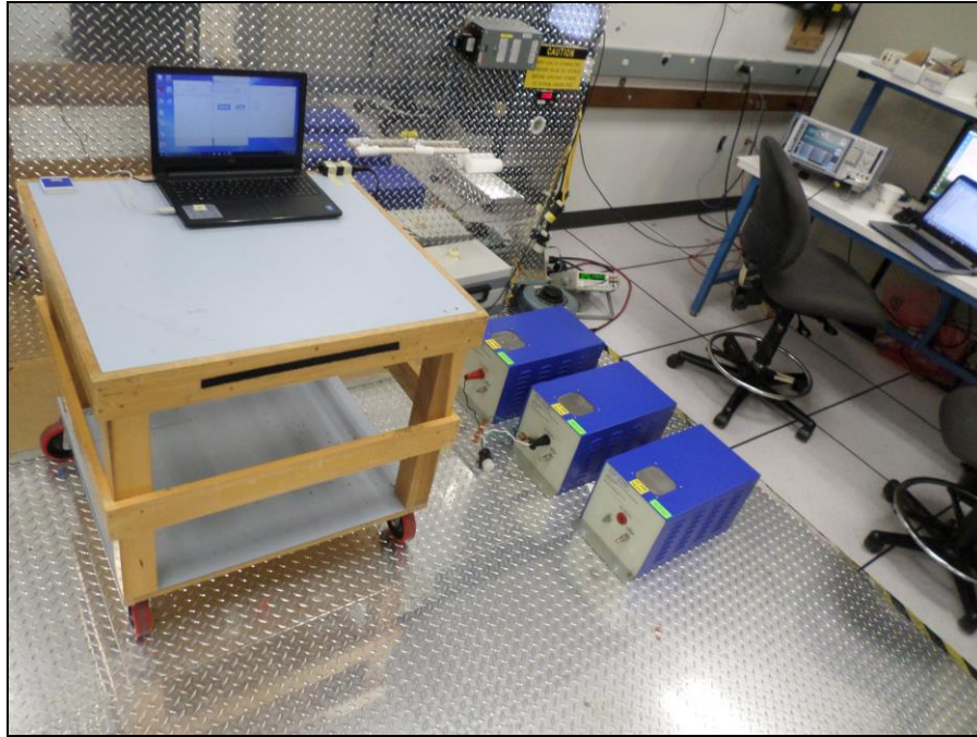
Photograph 1. Conducted Emissions, Station Setup
