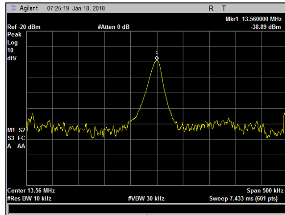
Plot 26. Frequency Stability, -15 pct, 20 degrees
