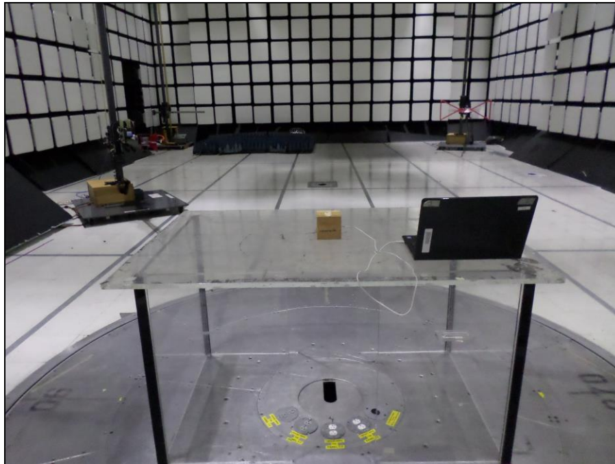
Photograph 9. Spurious Emissions, 30MHz – 135.6MHz, Rear Setup
