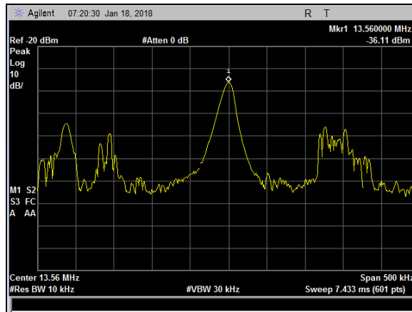
Plot 32. Frequency Stability, +15 pct, 20 degrees
