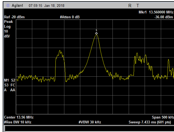
Plot 31. Frequency Stability, +15 pct, -20 degrees
