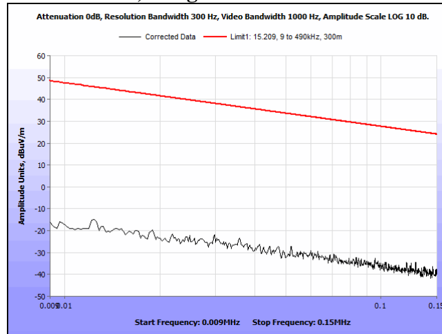
Plot 15. Spurious Emissions, Outside the Bands 13.110 - 14.010 MHz, 9KHz – 150KHz, 0 degrees
