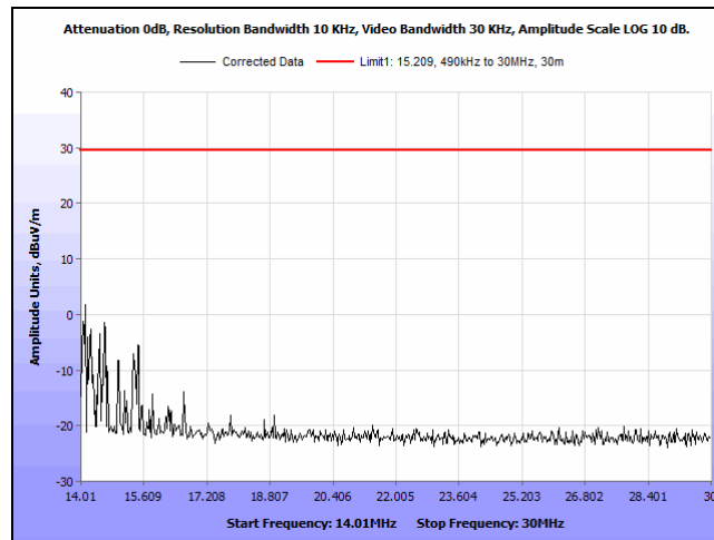
Plot 19 Spurious Emissions, Outside the Bands, 14.01MHz – 30MHz, 0 degrees
