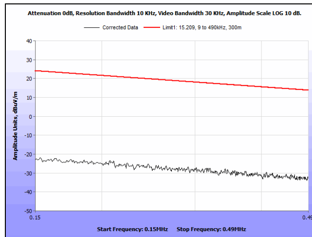
Plot 16. Spurious Emissions, Outside the Bands, 13.110 - 14.010 MHz, 150KHz – 490KHz, 0 degrees
