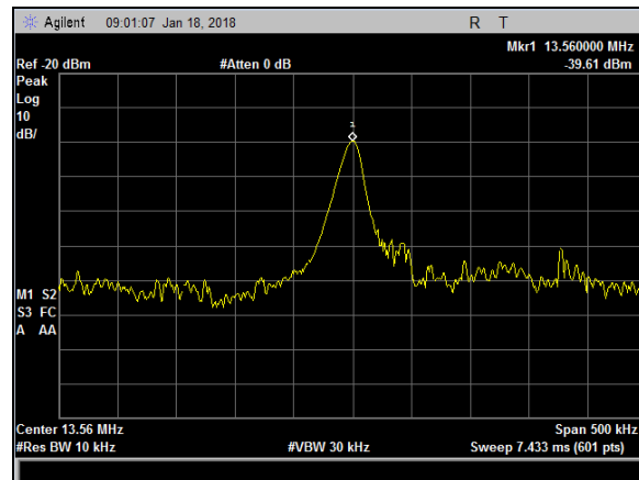
Plot 27. Frequency Stability, -15 pct, 50 degrees
