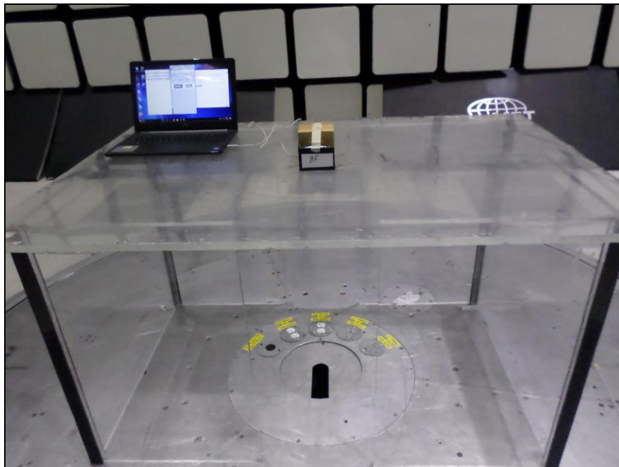
Photograph 4. Spurious Emissions, 9KHz - 30MHz, Front Setup
