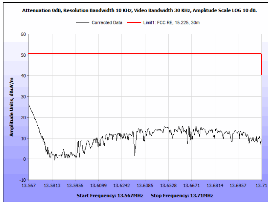
Plot 7. Operation Within the Band 13.567 – 13.710 MHz, 0 degrees
