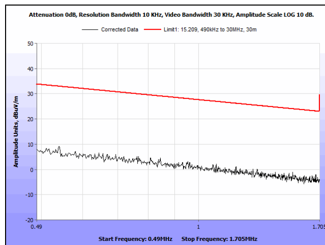
Plot 17. Spurious Emissions, Outside the Bands 13.110 - 14.010 MHz, 490KHz – 1.705MHz, 0 degrees
