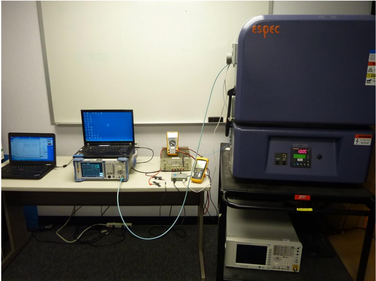
Figure 9: Frequency Stability Test Setup (Outside Thermo Chamber)
