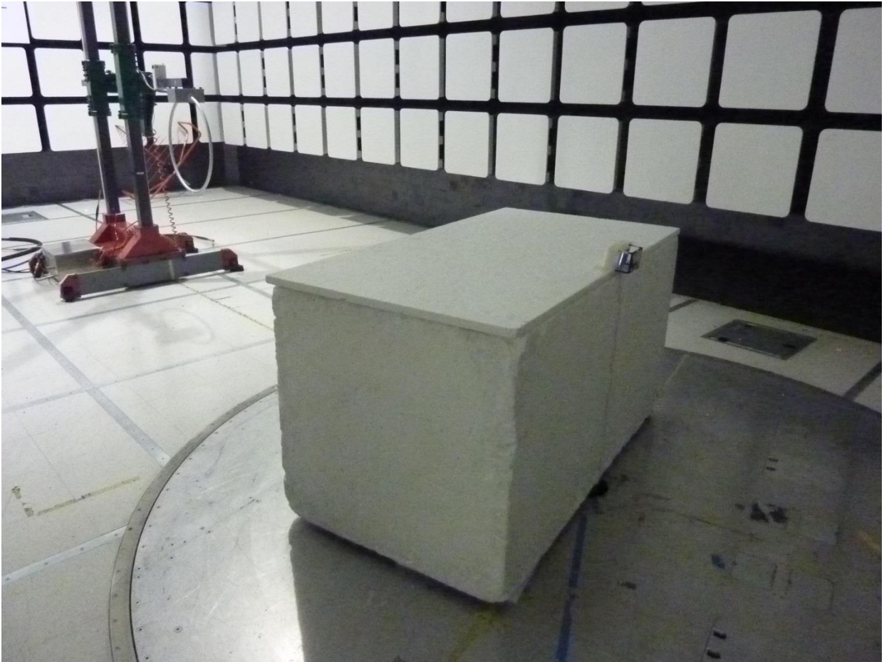
Figure 6: Test Setup for 9 kHz to 30 MHz; antenna at 90 degrees (Mode 2)
