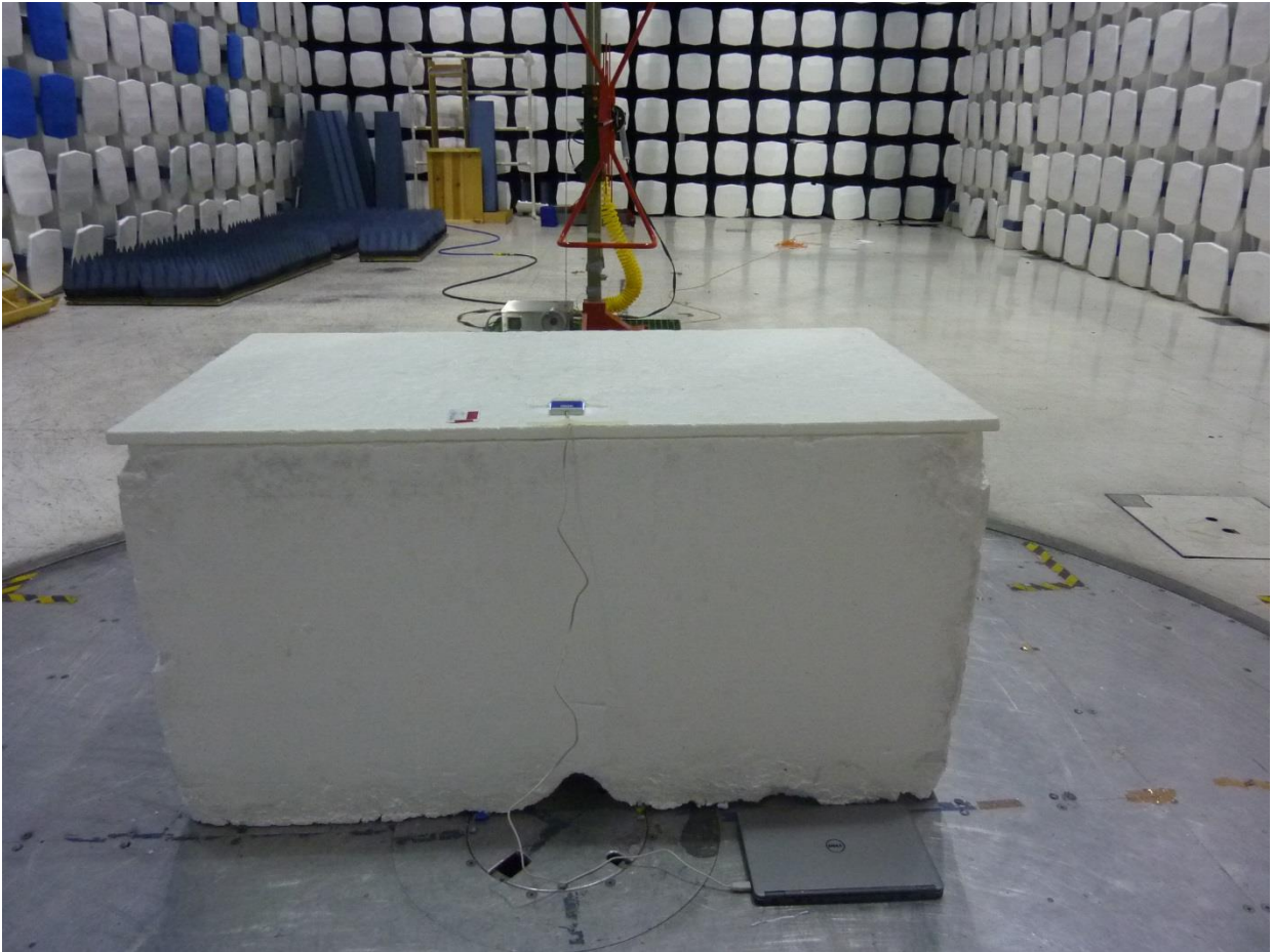
Figure 7: Test Setup for 30 MHz – 1000 MHz (Mode 1)
