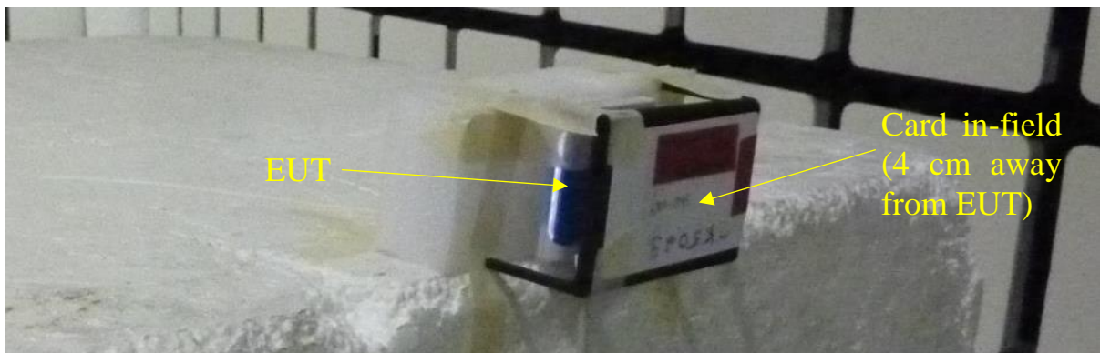
Figure 1: Test Setup of EUT – Mode 1
