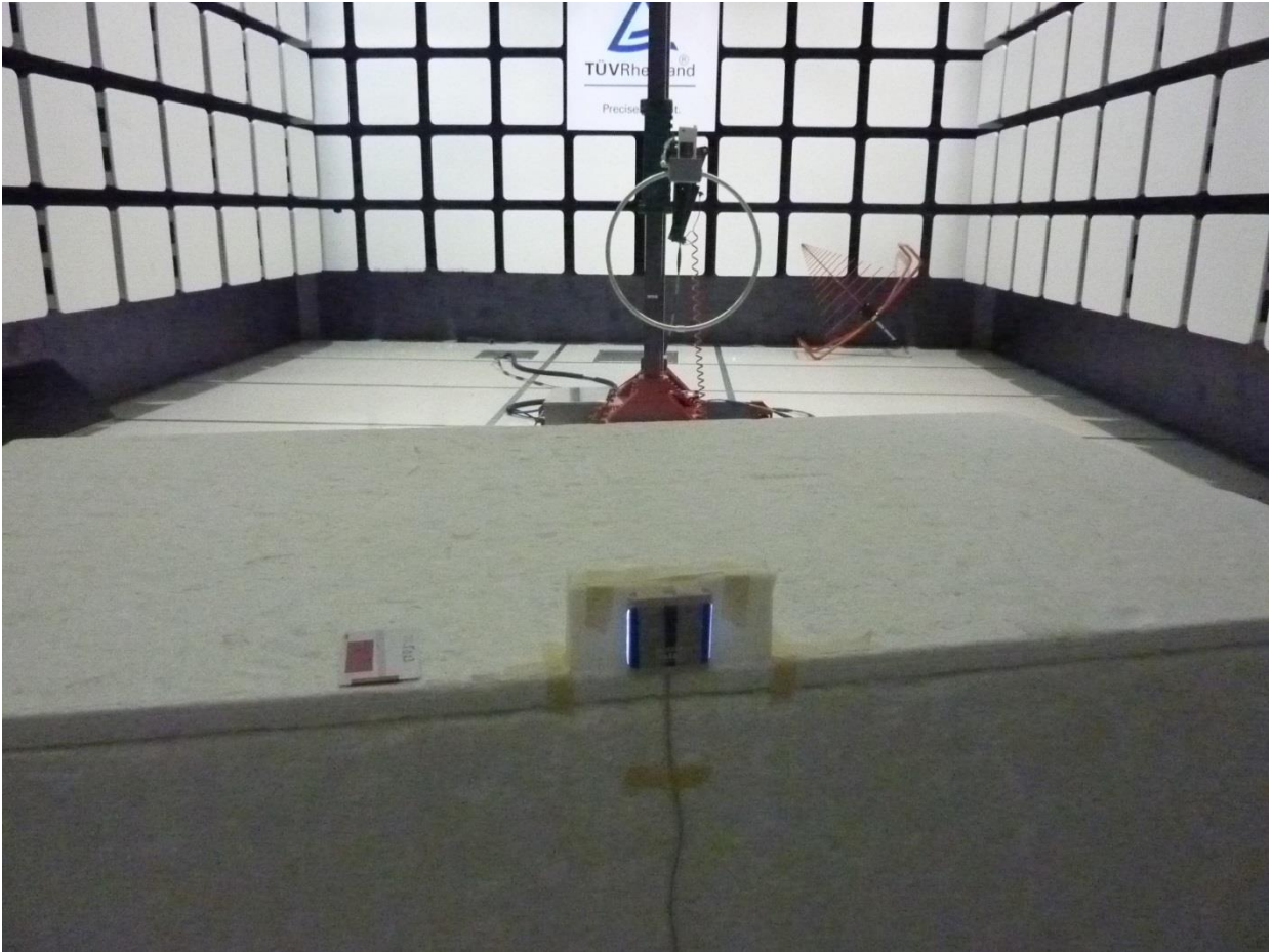
Figure 3: Test Setup for 9 kHz to 30 MHz; antenna at 0 degree (Mode 1)
